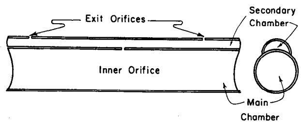
Figure 7-15.—Twin-wall emitter lateral.
