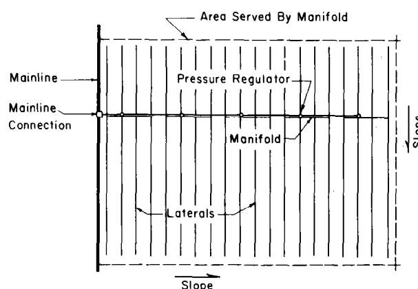
Figure 7-9.—Manifold layout showing inlet connection uphill from center and showing pressure-regulated manifolds.
