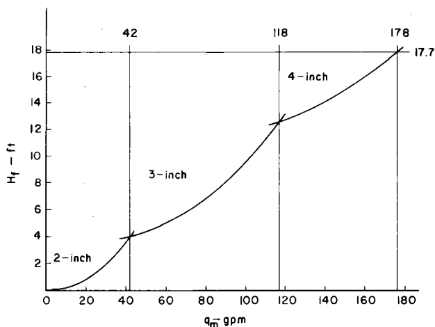
Figure 7-52.—Friction curve overlay to demonstrate graphical solution for determining manifold friction loss ( H_f ) for a spray system. q_m = manifold flow rate.
