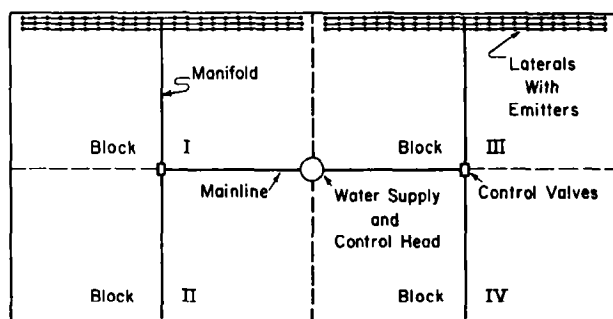
Figure 7-27.—Typical two-station split-flow layout for trickle irrigation system with Blocks I and III, or II and IV, operating simultaneously.
