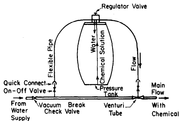
Figure 7-6.—Pressure-differential injection system.
