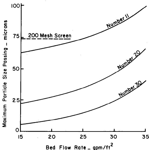
Figure 7-8.—Effect of flow rate on the maximum particle size passing through a typical free-flow sand filter with media of various sizes.
