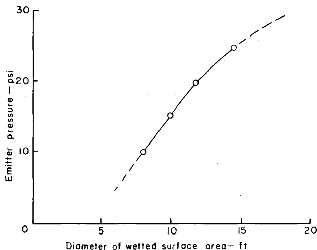
Figure 7-51.—Plot of spray diameter vs. emitter pressure developed from manufacturer's data for 0.04-in.-diameter orifice.
