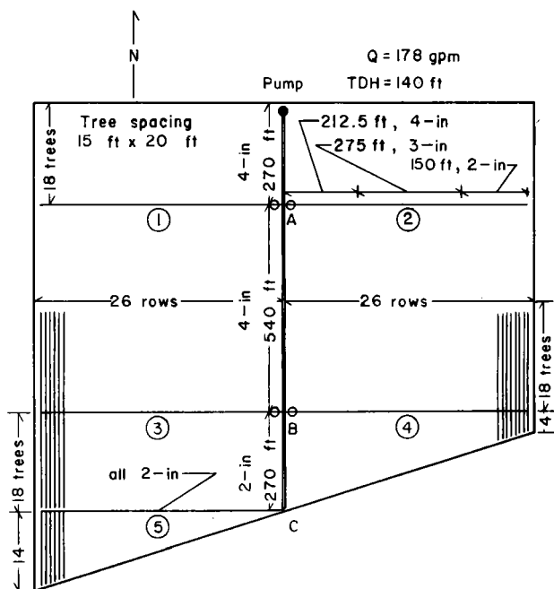
Figure 7-49.—Citrus grove with spray irrigation system. Lateral lines are 0.70-in. polyethylene and manifolds and main lines are polyvinyl chloride pipe.
