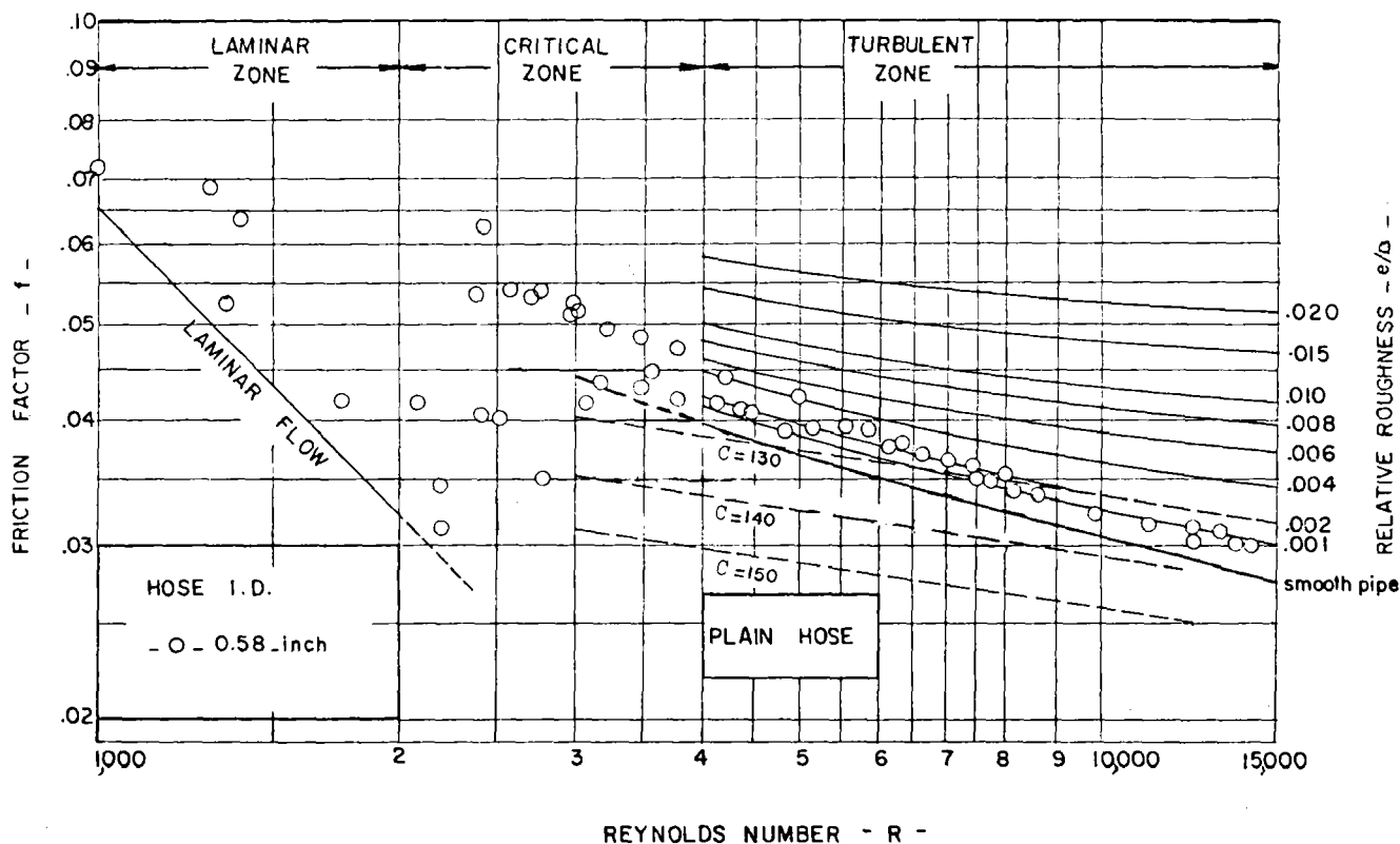
Figure 7-30.—Darcy-Weisbach f values for 1/2-in. (0.58-in. inside diameter) trickle irrigation hose.
