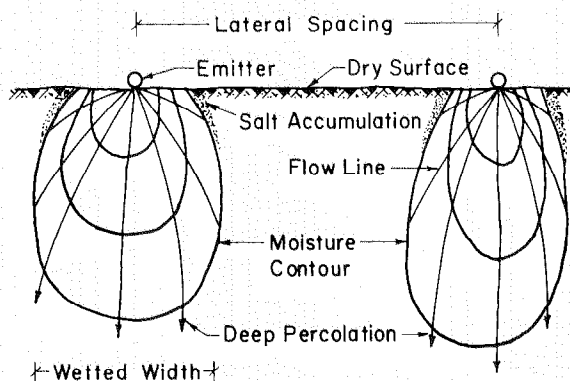
Figure 7-4.—Typical soil moisture pattern under trickle irrigation, showing salt accumulation.
