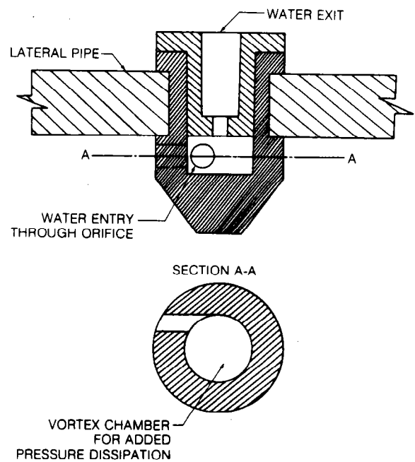
Figure 7-14.—Orifice-vortex-type emitter.
