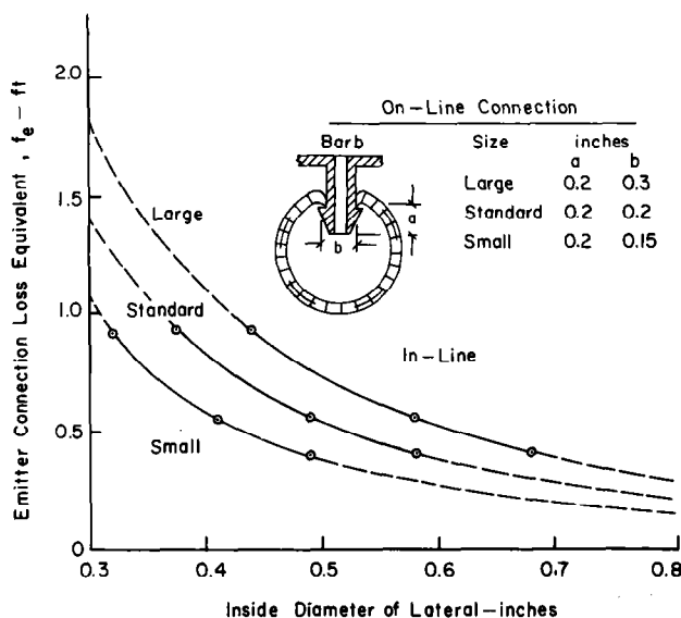
Figure 7-23.—Emitter-connection loss ( f_e ) values for various sizes of barbs and inside diameters of laterals
