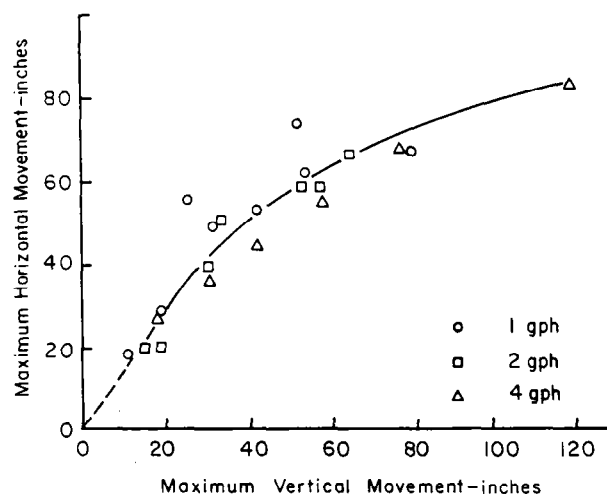
Figure 7-19.—Relationship between vertical and horizontal water movement in a dry sandy soil for various amounts of water and various application rates.
