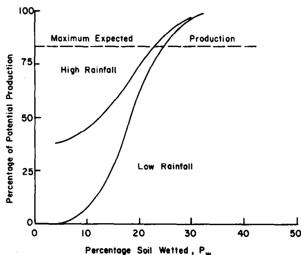
Figure 7-21.—Hypothetical relation of potential production to percent area wetted.
