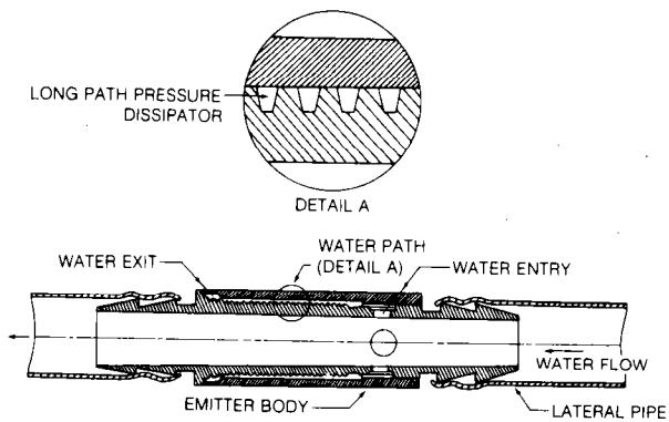
Figure 7-11.—Single-exit long-path emitter.
