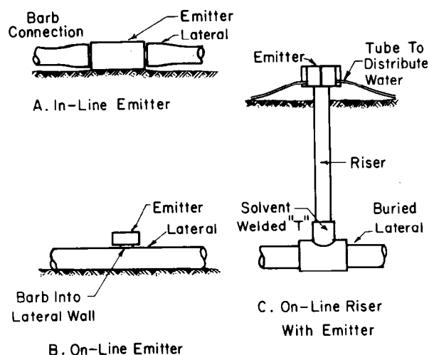
Figure 7-17.—Typical means for connecting emitters to laterals.
