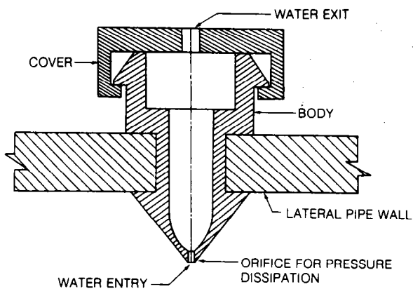
Figure 7-13.—Single-exit orifice-type emitter.
