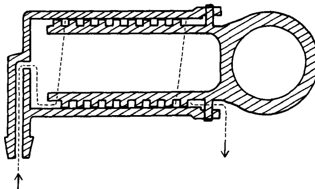
Figure 7-25.—Cross section of a long-path emitter that can be opened for easy cleaning.
