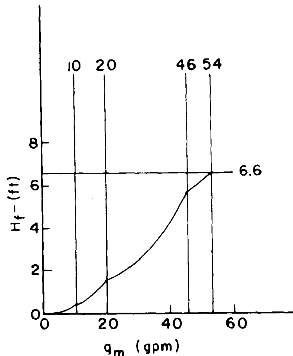
Figure 7-47.—Friction curve overlay to demonstrate graphical solution for determining manifold friction loss ( H_f ) for a drip system. q_m = manifold flow rate.
