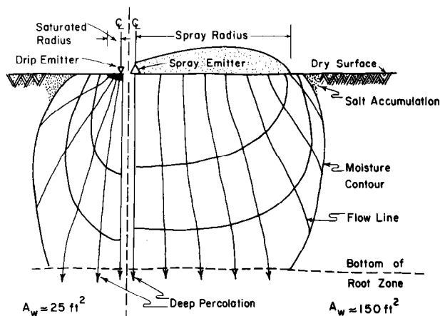
Figure 7-20.—Idealized wetting patterns in a homogeneous fine sandy soil under a drip and a spray emitter.
