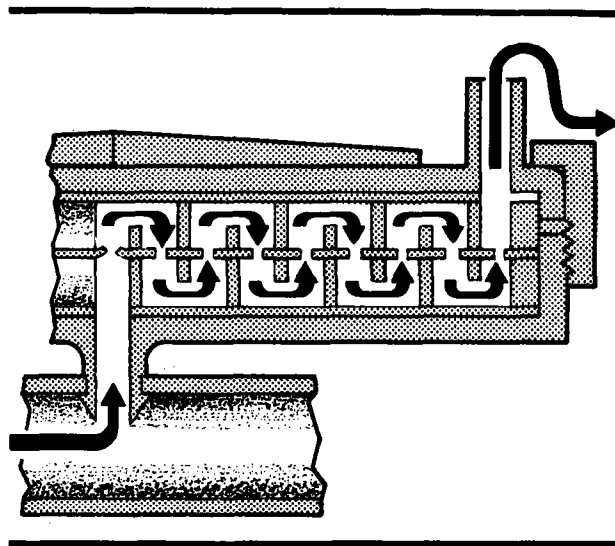
Figure 7-26.—Cross section of a continuous-flushing emitter.
