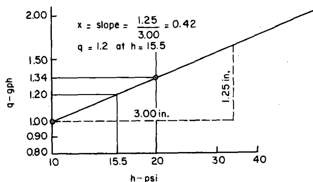
Figure 7-24.—Graphical method for determining the discharge exponent ( x ) in a sample calculation.
