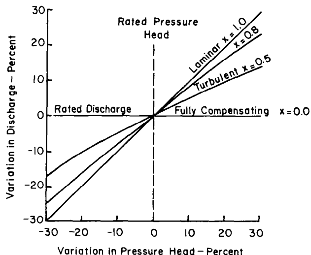
Figure 7-22.—Discharge variations resulting from pressure changes for emitters with various discharge exponents ( x ).
