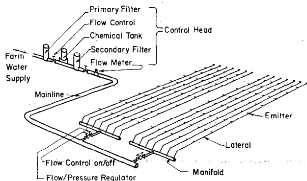
Figure 7-5.—Basic components of a trickle irrigation system.
