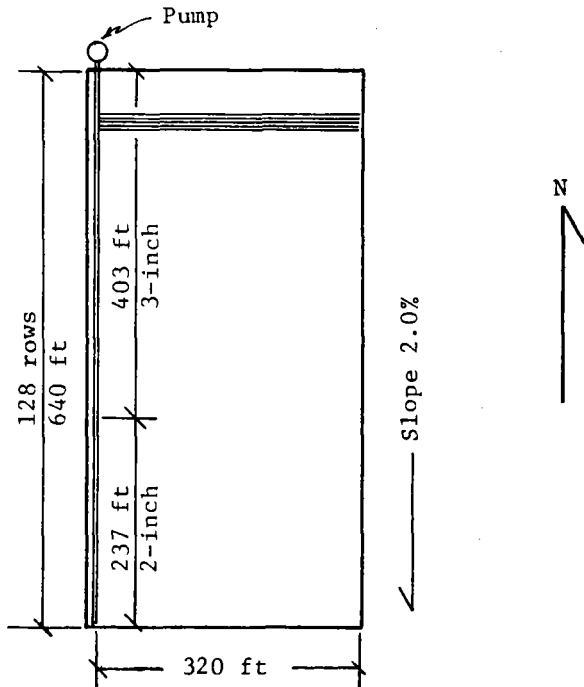
Figure 7-54.—Tomato field with line-source drip irrigation. Lateral lines are single-chamber 0.625-in. (ID) polyethylene tubing that discharge 0.4333 gpm/100 ft; the manifold is buried polyvinyl chloride pipe.
