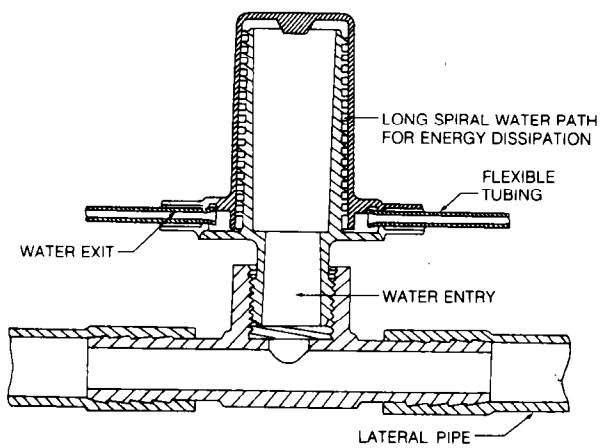
Figure 7-12.—Multiexit long-path emitter.
