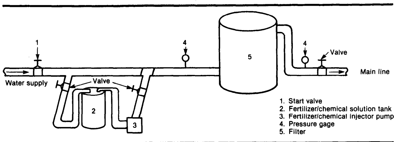
Figure 7-7.—Valves at the head of a trickle irrigation system.
