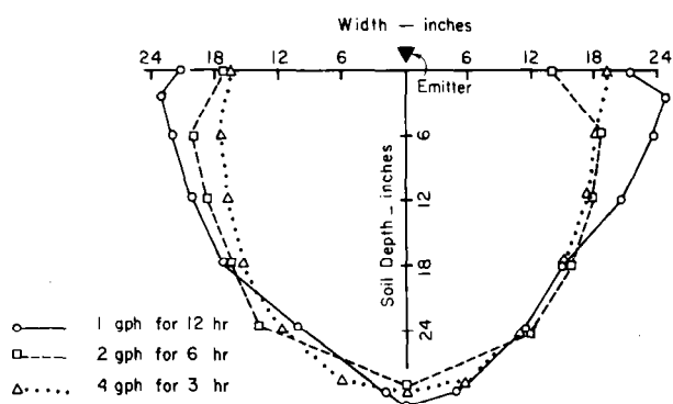
Figure 7-18.—Wetting pattern profiles for equal volumes (12 gal) of water applied at three rates to a dry sandy soil.
