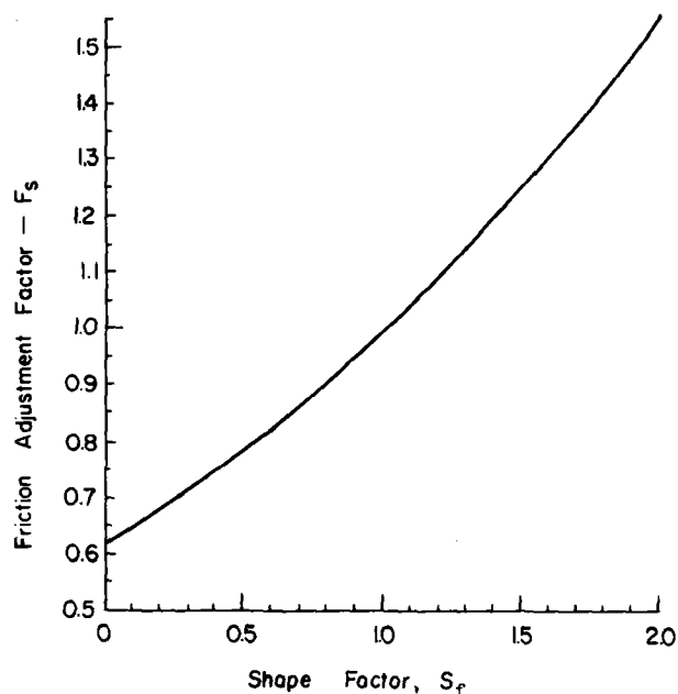
Figure 7-38.—Graph for determining manifold pipe-friction adjustment factors for trapezoidal subunits.
