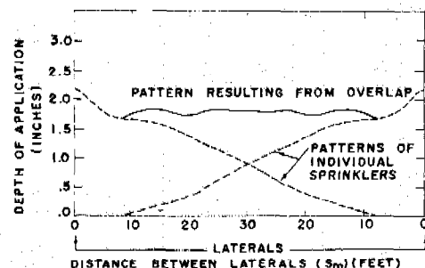
Figure 11-22.—Example of the distribution patterns between sprinklers along the lateral and between laterals.
