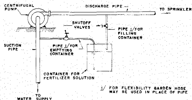
Figure 11-59.—A method for adding fertilizers in solution to a centrifugal pump system.
