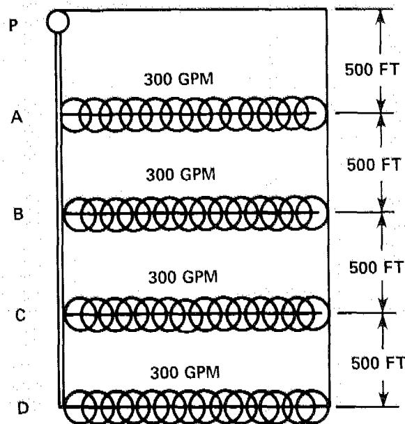
Figure 11-40.—System layout for sample calculation 11-13, as shown in table 11-23.
