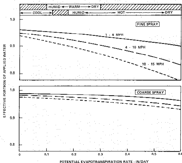
Figure 11-17.—Effective portion of water applied, R_e , by sprinkling with fine and coarse sprays in different wind conditions and with different potential evapotranspiration rates on crops with full canopies.
