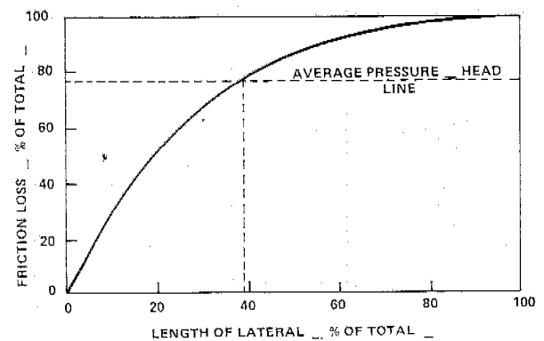
Figure 11-47.—Loss of pressure due to friction along a lateral having only one size of pipe.
