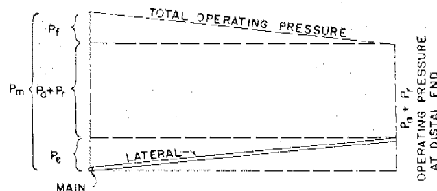
Figure 11-32.—Lateral laid uphill.
