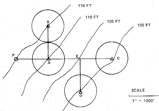
Figure 11-41.—Layout of project with four small center pivot laterals.
