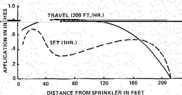
Figure 11-49.—Typical application patterns of a traveling and a set gun sprinkler operating in very low wind.
