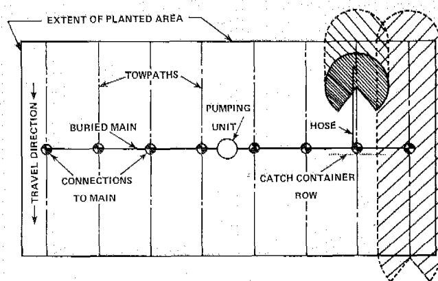
Figure 11-9.—Typical layout for traveling sprinklers showing location of the line of catch containers used for evaluating the distribution uniformity.
