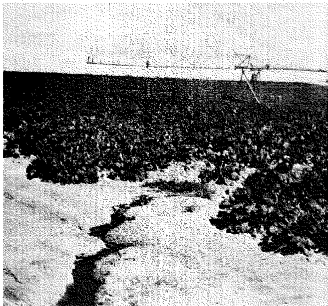
Figure 11-58.—Runoff near the moving end of a center-pivot lateral.
