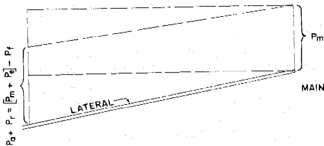
Figure 11-33.—Lateral laid downhill.
