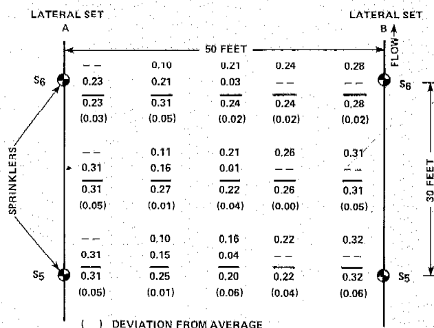
Figure 11-25.—Combined catch pattern in inch per hour between sprinklers 5 and 6 for a 50-ft lateral spacing.
