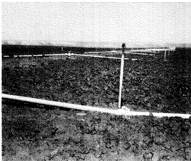
Figure 11-4.—Solid-set sprinkler laterals connected to buried mainline.
