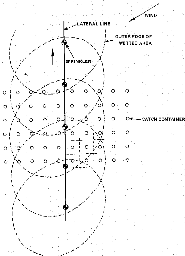
Figure 11-48.—Layout of catch containers for testing the uniformity of distribution along a sprinkler lateral line.
