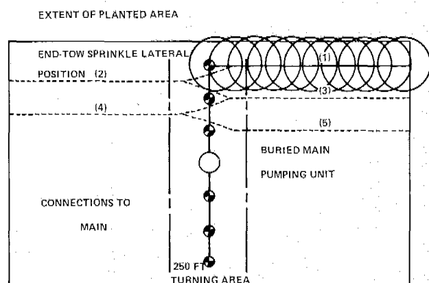
Figure 11-2—Schematic of move sequence for end-tow.
