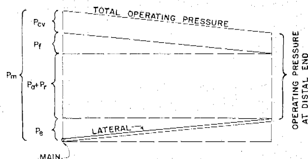
Figure 11-34.—Lateral with flow-control valves.
