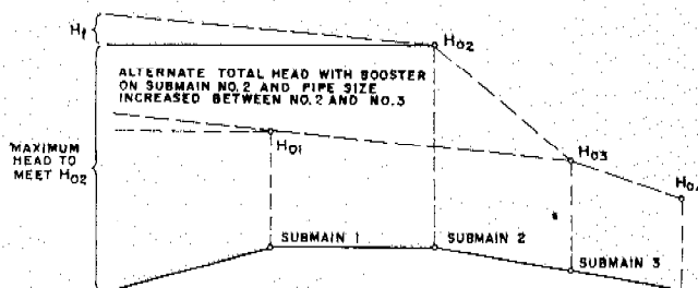
Figure 11-37.—Maximum operating conditions with submain.
