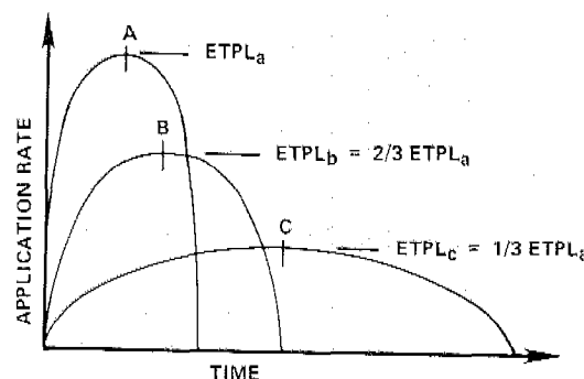
B) WATER APPLICATION RATES AT DIFFERENT POINTS ALONG PIVOT LATERAL.
