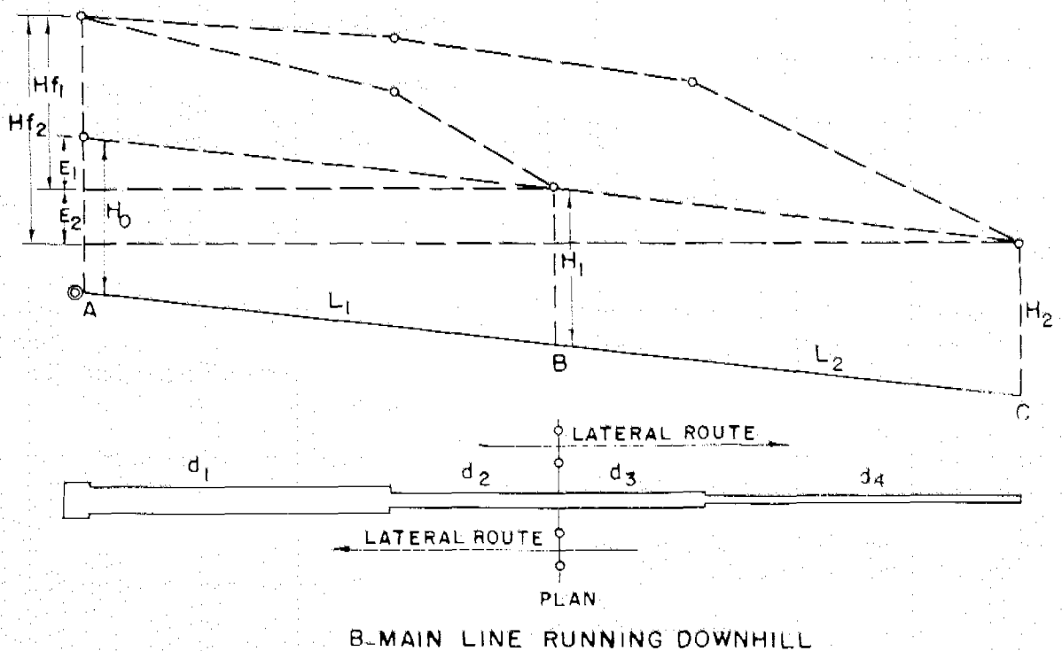
Figure 11-35.—Design of mainline with twin laterals, split-line operation.
