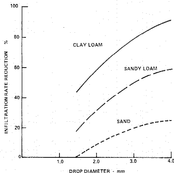
Figure 11-16.—Relation of infiltration rate reduction due to sprinkling three different soils at an application rate of approximately 0.5 iph.
