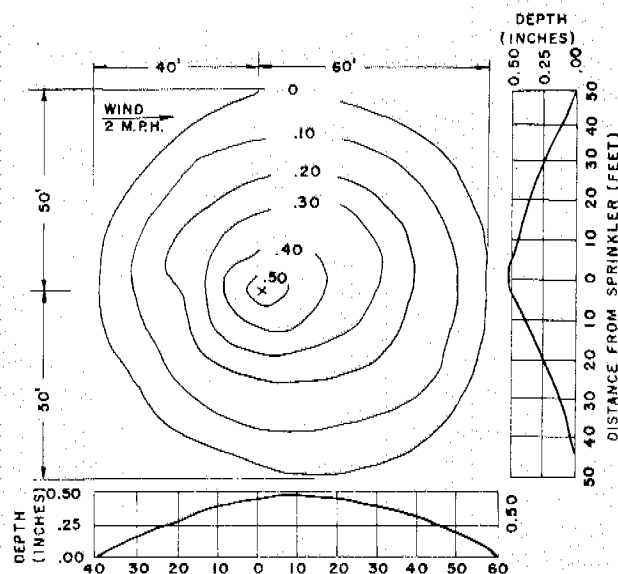
Figure 11-19.—Distribution pattern and precipitation profiles from a typical double-nozzle sprinkler operating under favorable conditions.
