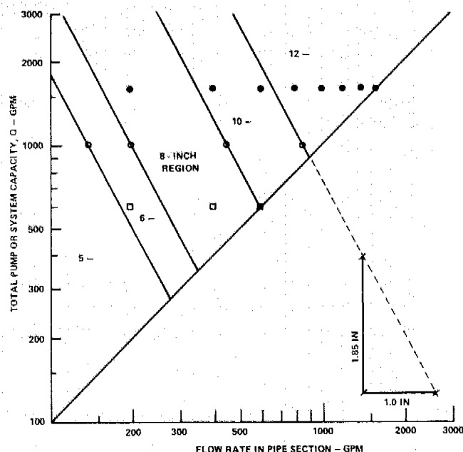
Figure 11-38.—Economic pipe selection chart for portable aluminum pipe with C=130 , CRF=0.214 , and U' = \$138.60/\text{WHP-year} .
