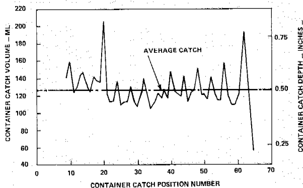
Figure 11-57.—Profile of container catch from center-pivot sprinkler evaluation test.
