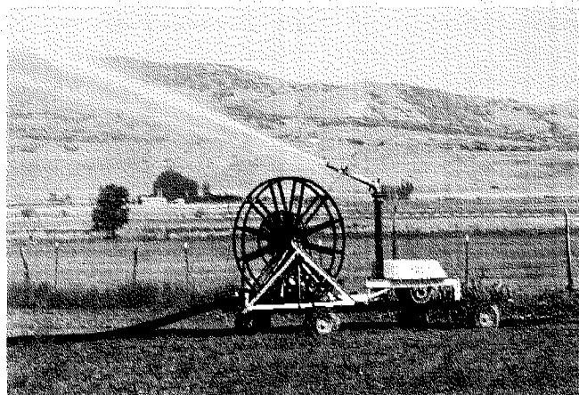
Figure 11-8.—Hose-fed traveling gun-type sprinkler in operation.
