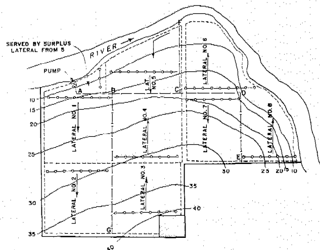
Figure 11-12.—Layout of a complete periodic hand-move sprinkle system. The odd-shaped area of 72 acres illustrates the subdivision of the design area to permit rotation to all areas except one small tract near the pumping location. Number of sprinklers required per acre, 1.5; number of settings for each lateral per irrigation, 10; required number of sprinklers, 72 \times 1.5 = 108 ; total sprinklers required for the eight laterals, 124. Lateral 8 will require an intermediate pressure-control valve.
