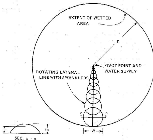
Figure 11-53.—Watering characteristics of center-pivot irrigation machines.
