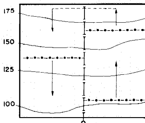
B-Layout illustrating use of odd number of laterals to provide required number of operating sprinklers.
