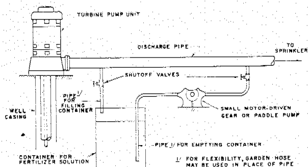
Figure 11-60.—A method for adding fertilizers to a turbine pump system using a small gear or paddle pump.
