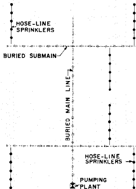
D—Permanent mains and submains with portable hose lines.
