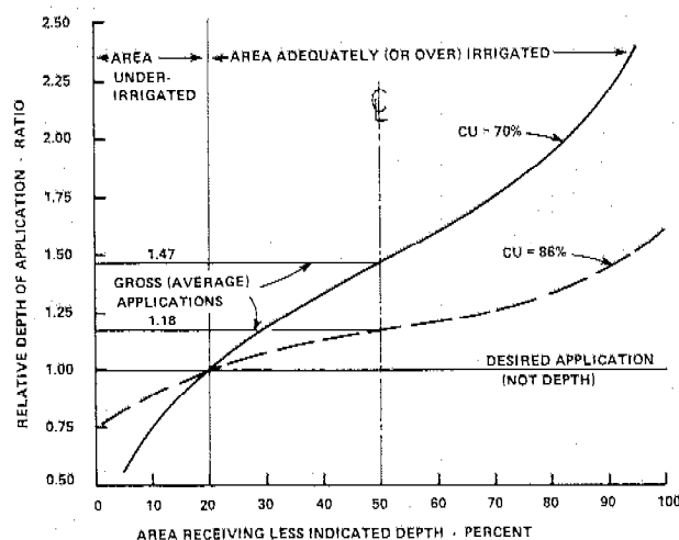
Figure 11-27.—Relationships between surface area and depth of water applied for CU values of 70 and 86 percent when 20 percent of the area is underirrigated and the remaining 80 percent of the area is adequately (or over) irrigated.
