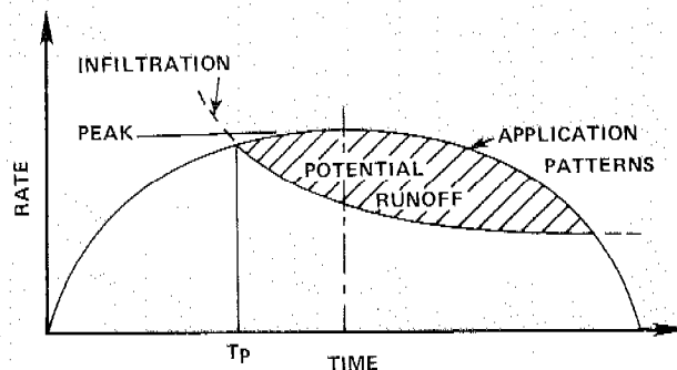
Figure 11-51.—Intersection between a typical elliptical pattern of water application rate under a center pivot and a potential infiltration curve.
