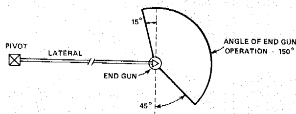
Figure 11-54.—Top view of end-gun sprinkler wetting pattern showing recommended angle of operation.
