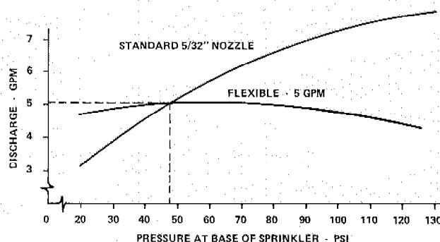
Figure 11-26.—Comparison of pressure versus discharge relationship for a standard fixed nozzle and a special flexible orifice nozzle.
