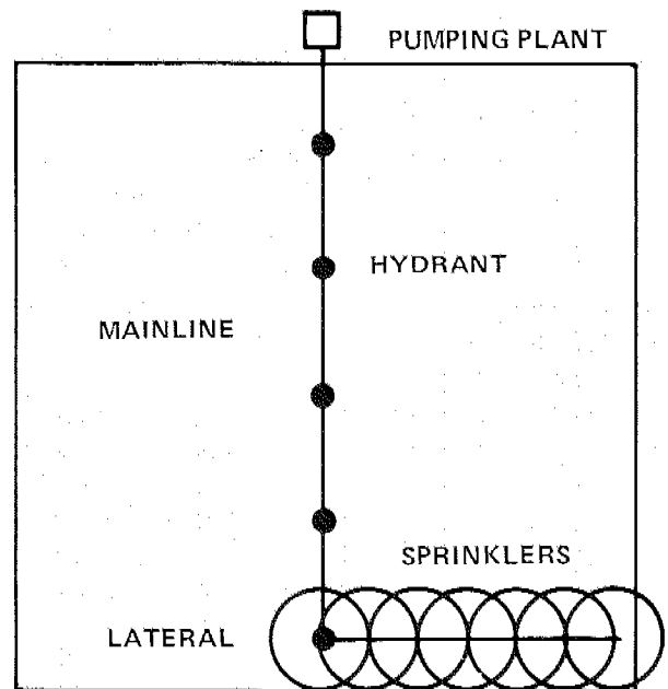
Figure 11-18.—Basic sprinkle system components.
