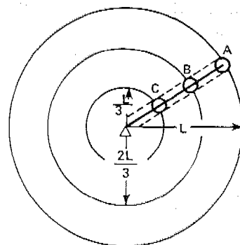
A) AERIAL VIEW OF CENTER PIVOT FIELD WITH UNIFORM WIDTH OF WETTED STRIP.
