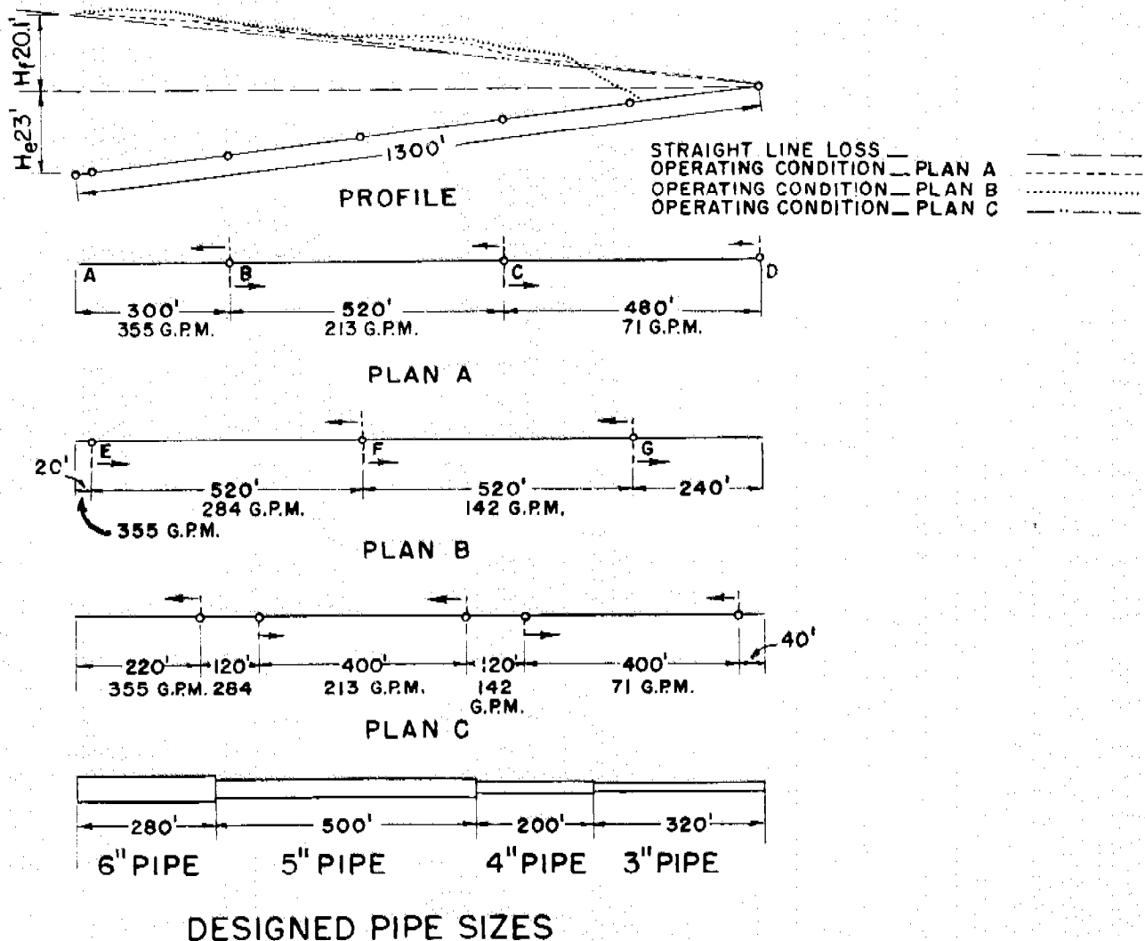
Figure 11-36.—Design of an uphill mainline with five 71 gpm laterals, split-line operation assuming the allowable friction head loss is 20.1 ft and the elevation difference is 23 ft.
