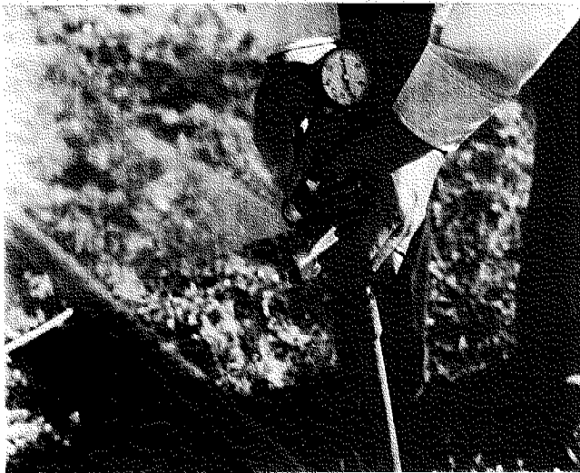
Figure 11-45.—Measuring pressure at sprinkler nozzle with gage connected to pitot tube.
