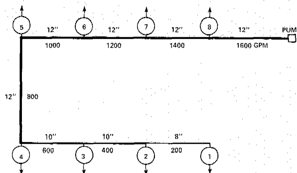
(A) 1600 - GPM SYSTEM WITH EIGHT 200 - GPM OUTLETS.
