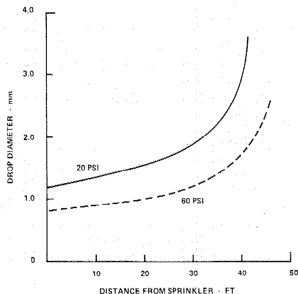
Figure 11-15.—Drop sizes at various distances from a standard 5/32-in nozzle operating at 20 and 60 psi.
