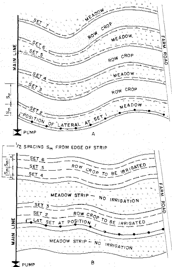
Figure 11-31.—Typical sprinkler lateral layouts on stripcropped areas.
