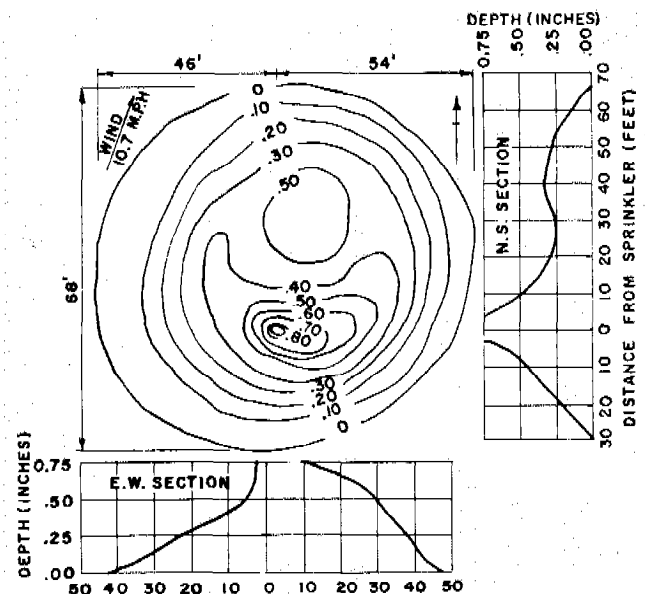
Figure 11-21.—Effect of wind on distribution pattern and precipitation profiles from a typical intermediate double-nozzle sprinkler.
