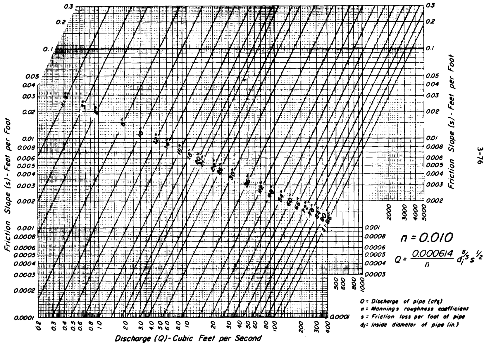
Exhibit 3-5 Discharge of circular pipes flowing full. Manning's n = 0.010 (Sheet 1 of 6)
