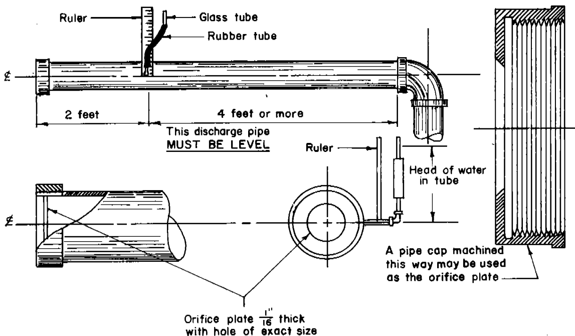
Figure 3-27 Pipe orifice
