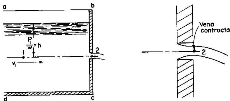
Figure 3-16 Flow through an orifice
