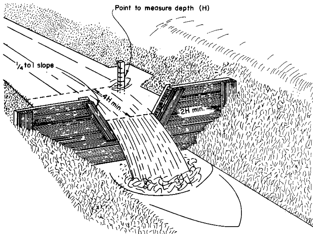
Figure 3-22 Cipolletti weir
