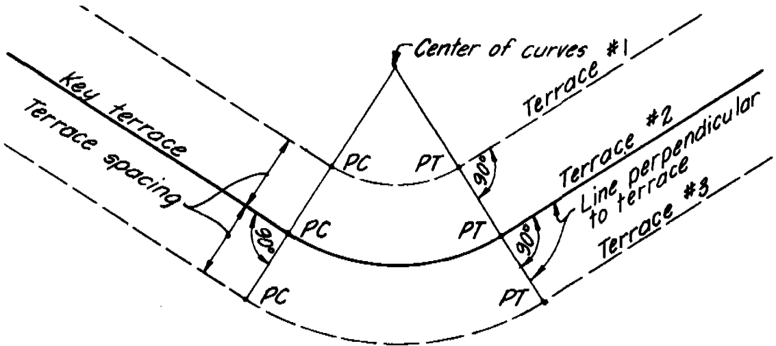
Figure 8-39 Layout geometry
