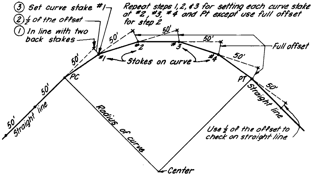
Figure 8-52 Step offset method for staking a curve
