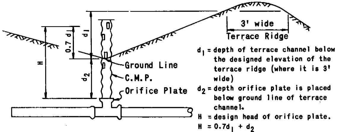
Figure 8-65 Design head for orifice plate
