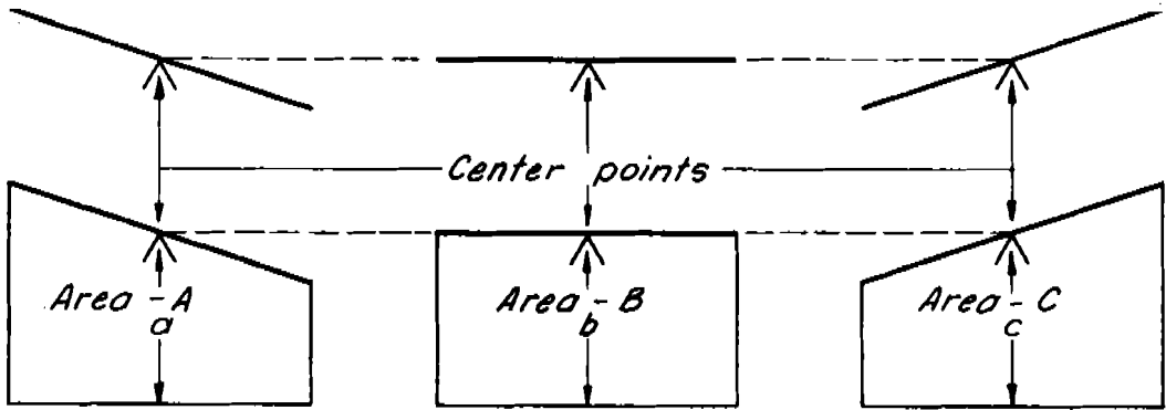
Figure 8-53 Theory of the balance point
