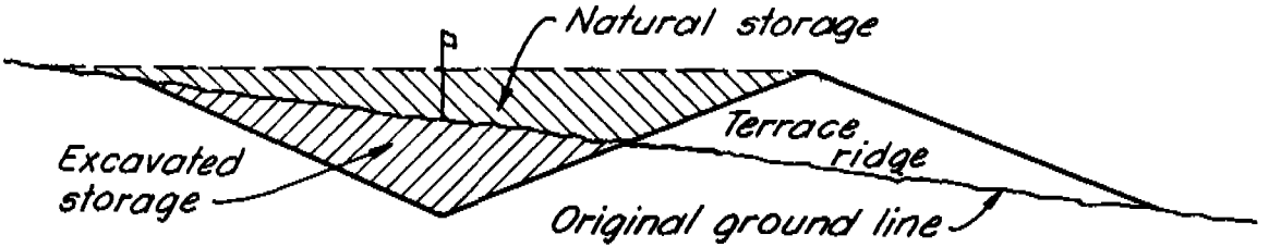
Figure 8-55 Storage - Natural and excavated
