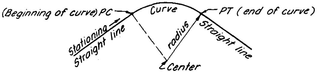
Figure 8-37 Single curve
