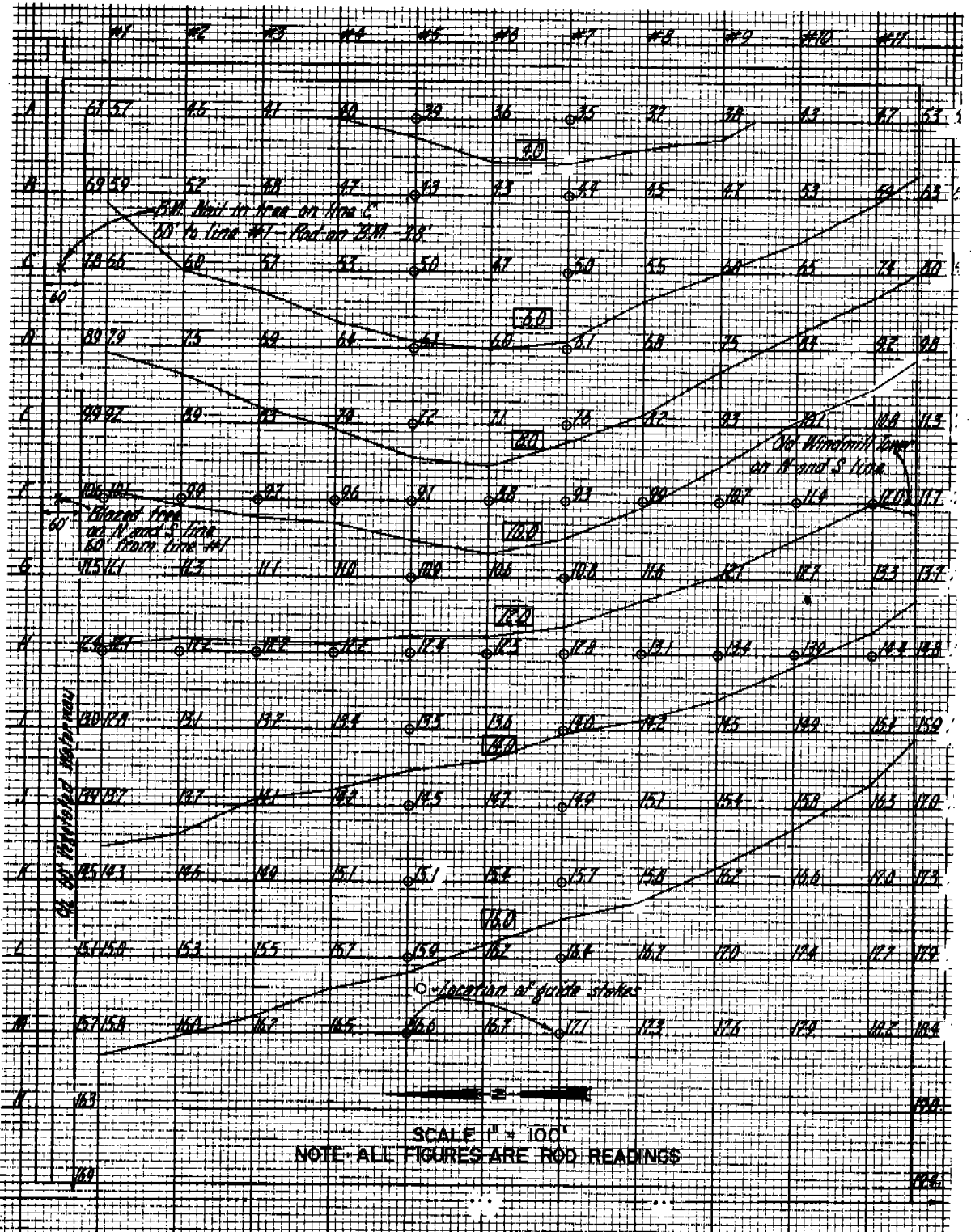
Figure 8-44 Grid survey map for use in parallel terrace system design and layout (Sheet 1 of 2)
