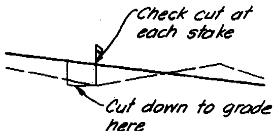
Figure 8-73 Guide for construction
