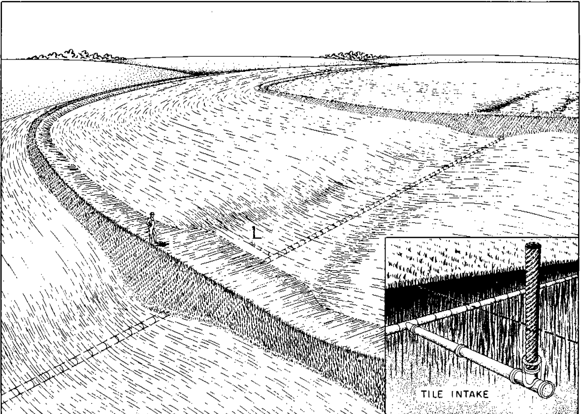
Figure 8-4 Gradient terraces with tile outlets
