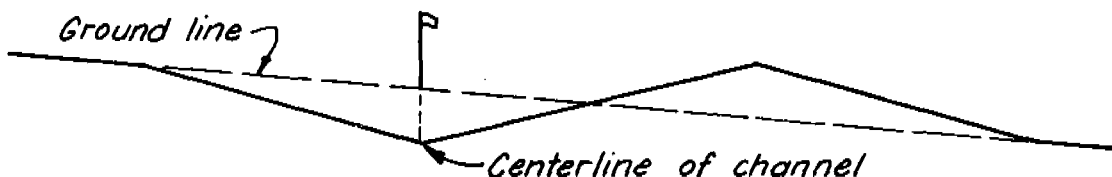
Figure 8-47 Method 1 - Staking
