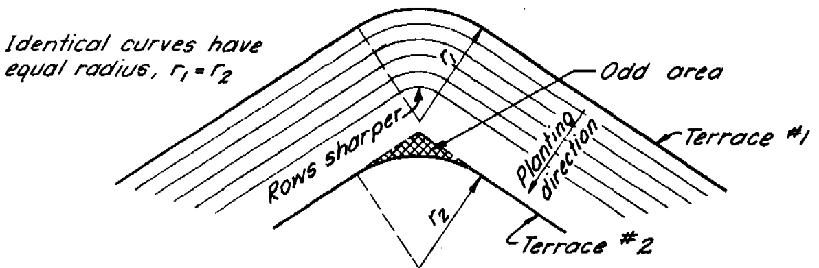
Figure 8-31 Planting toward center of curves
