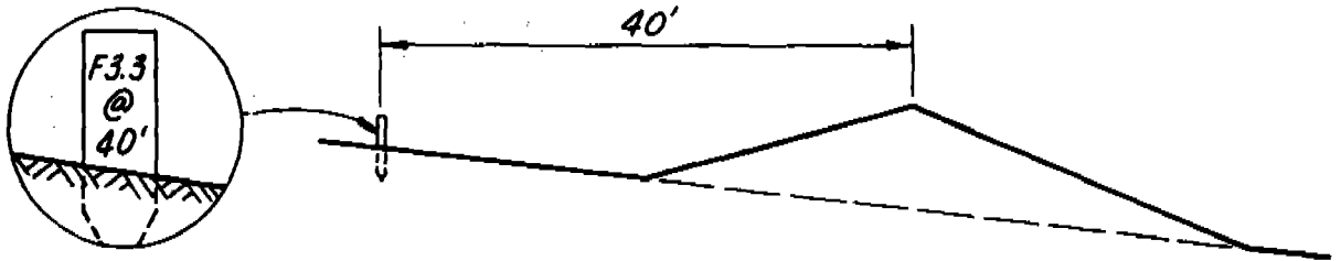
Figure 8-71 Reference stake
