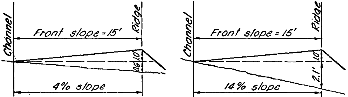
Figure 8-16 Slope increased with broad base ridge section
