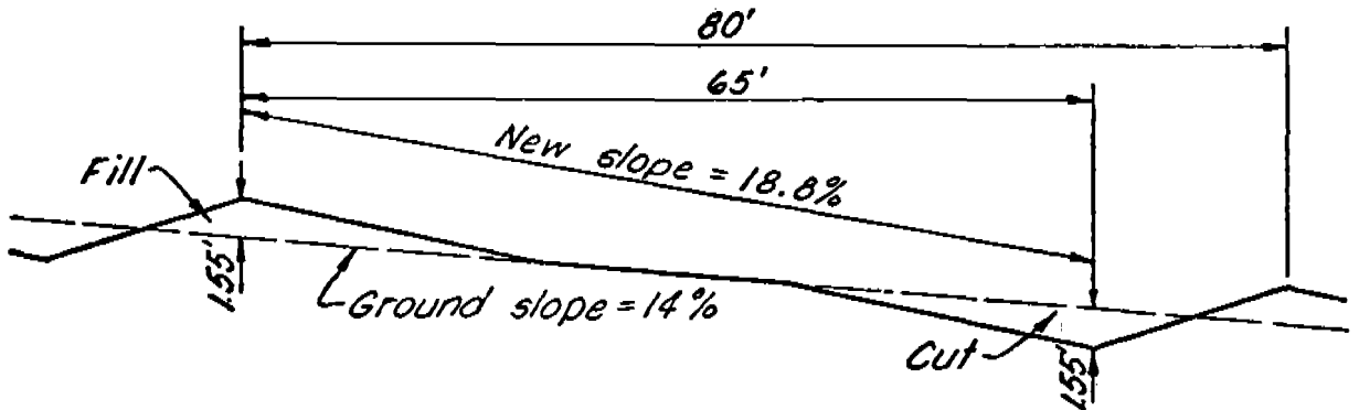
Figure 8-17 No excavation on uphill side
