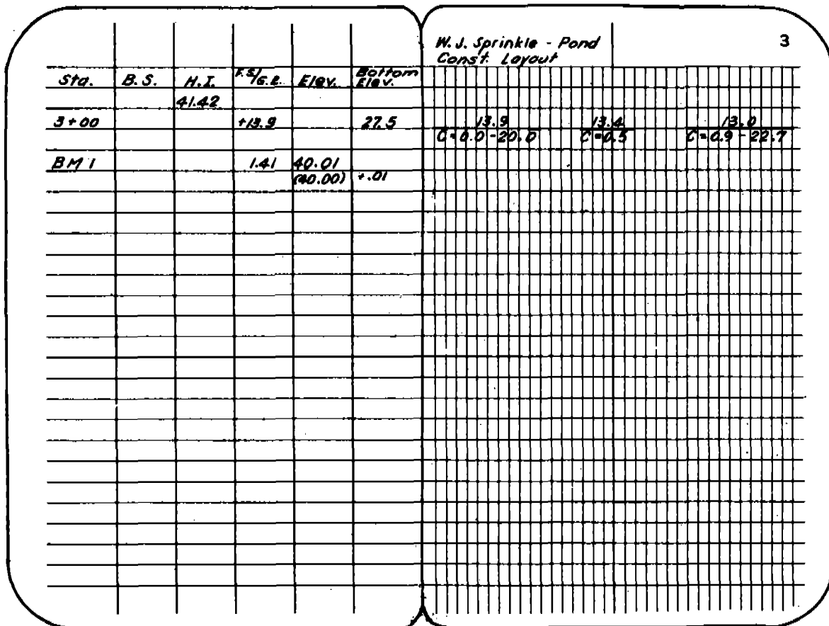
Figure 11–10 Construction layout notes (Sheet 2 of 2)
