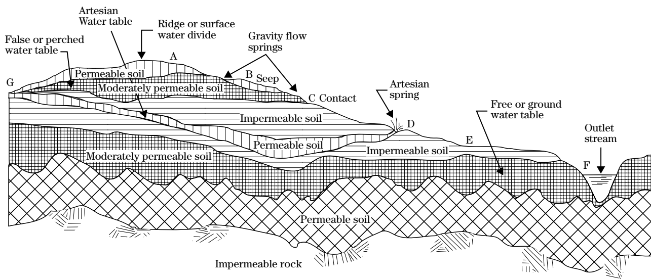
Figure 14-49 Ground water movement
