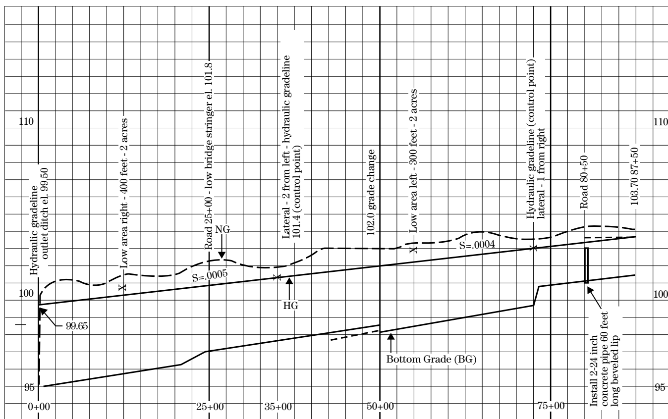
Figure 14-17 Design profile
