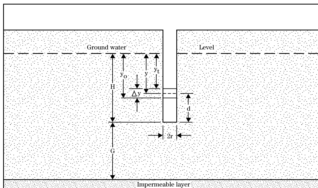
Figure 1 Symbols for auger-hole method of measuring hydraulic conductivity
