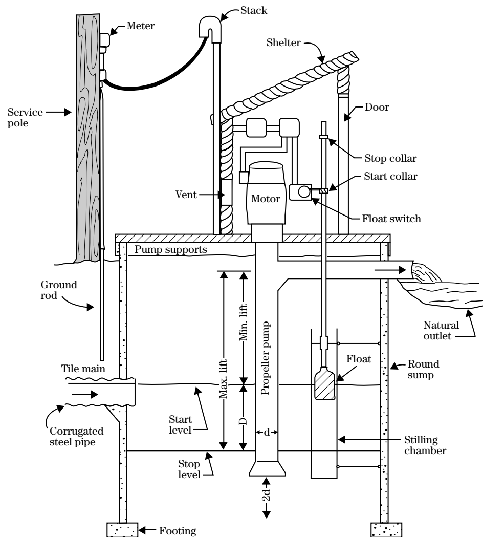
Figure 14-60 Pump installation
