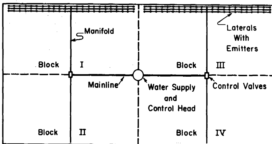
Figure 15-3—Typical two-station, split-flow layout for a trickle irrigation system with blocks I and III, or II and IV operating simultaneously.
