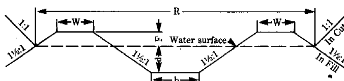
Finished Ditch Section
