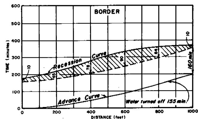
Figure 15-4A—Sample advance and recession curves (in feet).
