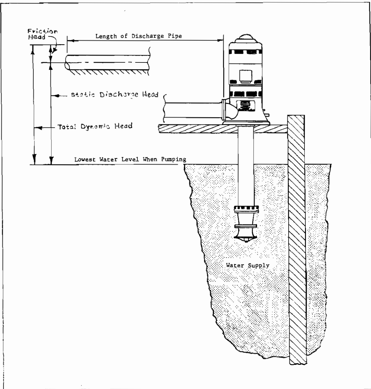
FIGURE 3. PROPELLER PUMP
