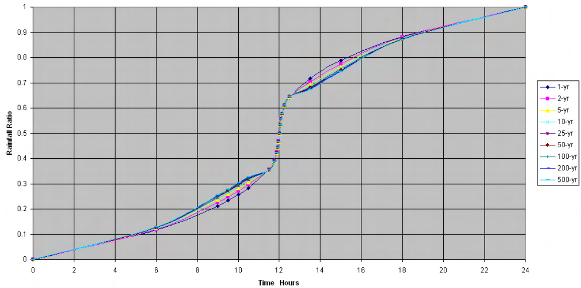
Figure 5-1D. Design rainfall distribution for 1-year to 500-year for Taguac (914229), Guam
