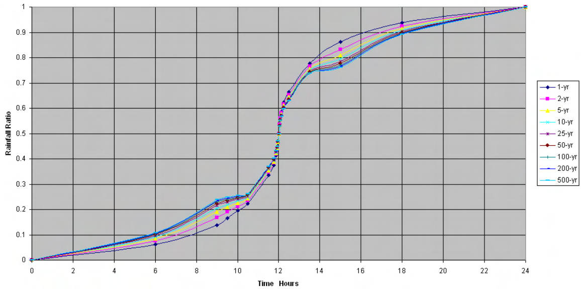
Figure 5-1L. Design rainfall distribution for 1-year to 500-year for Koror (914351), Palau
