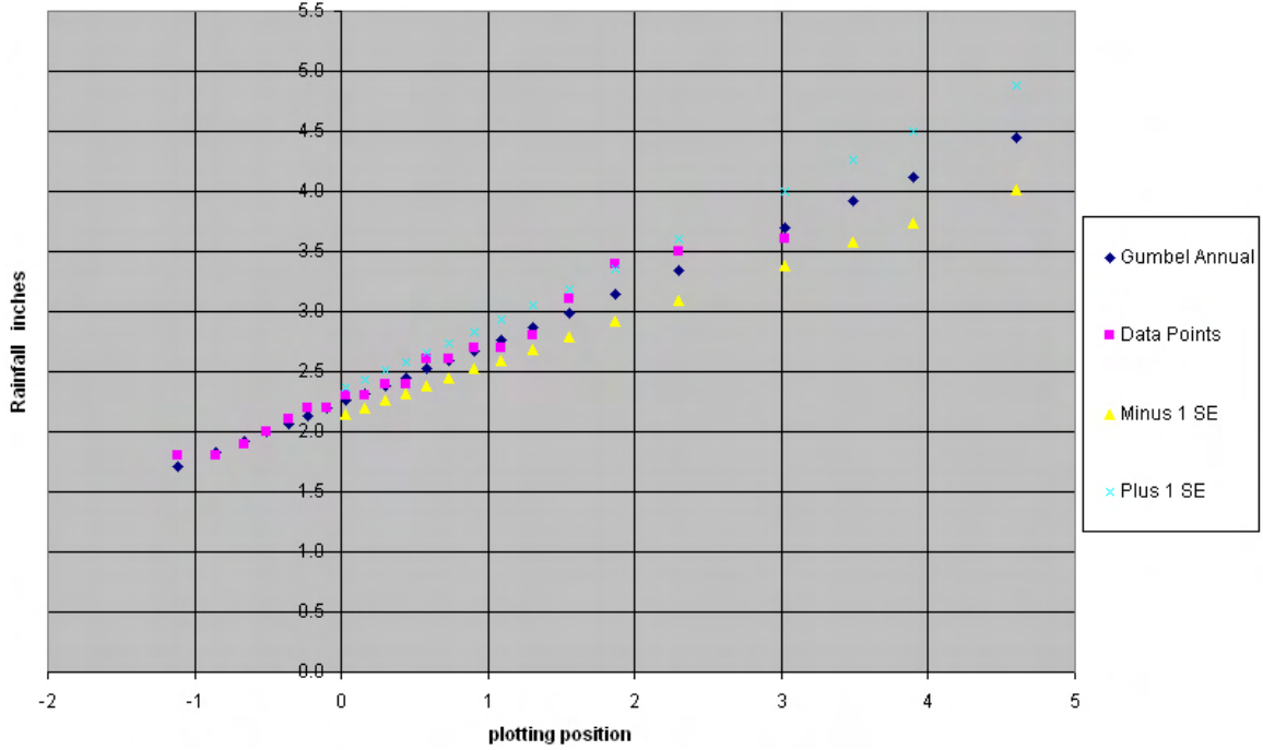
Figure 7-O1. Plot of 1-hour data points versus Gumbel analysis for Atuu, Tutuila, American Samoa.
