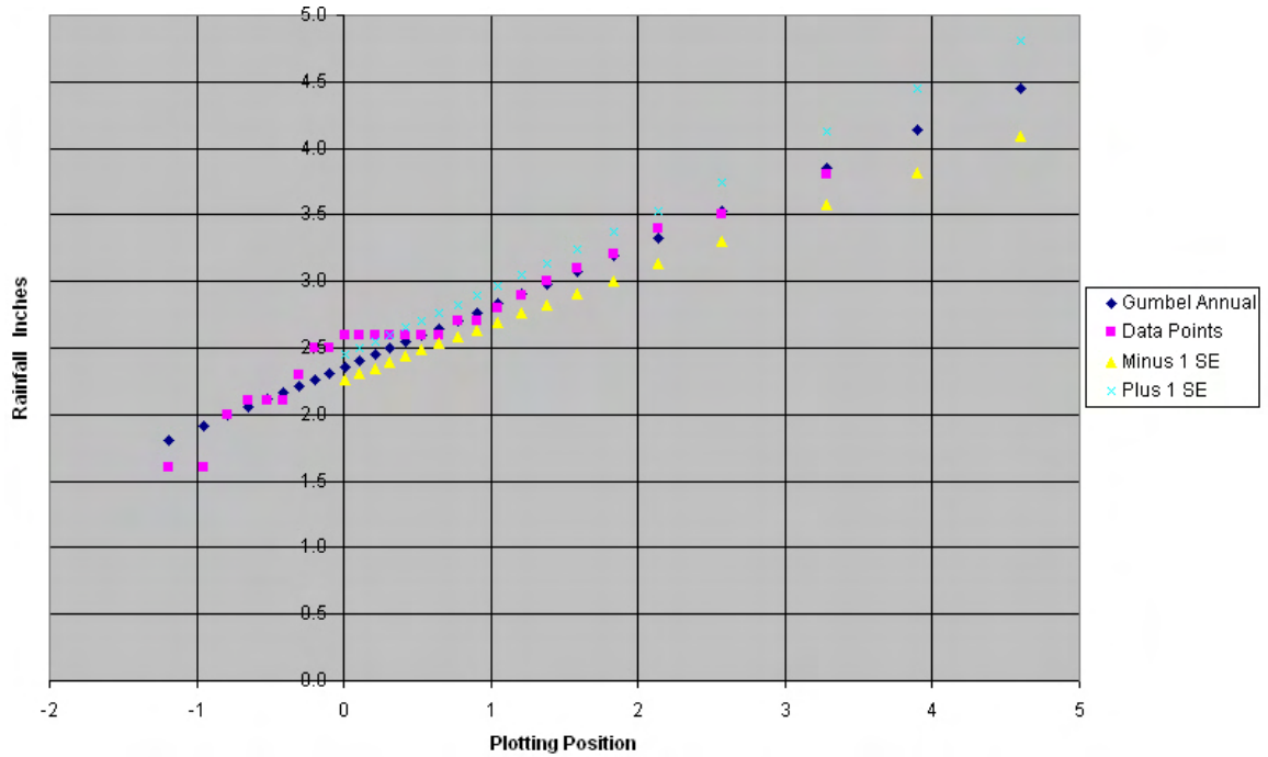
Figure 7-P1. Plot of 1-hour data points versus Gumbel analysis for Malaeloa, Tutuila, American Samoa.
