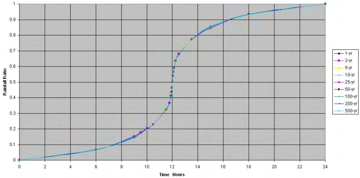
Figure 5-1C. Design rainfall distribution for 1-year to 500-year for Piti (914670), Guam
