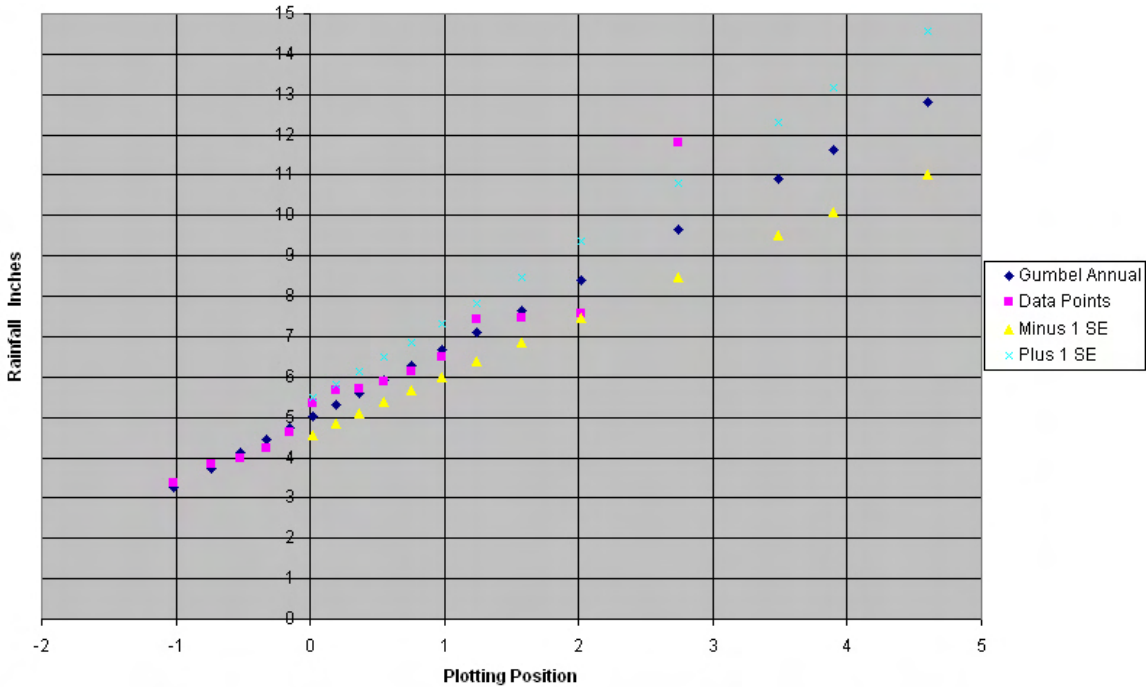
Figure 7-H3. Plot of 24-hour data points versus Gumbel analysis for Yap, FSM.
