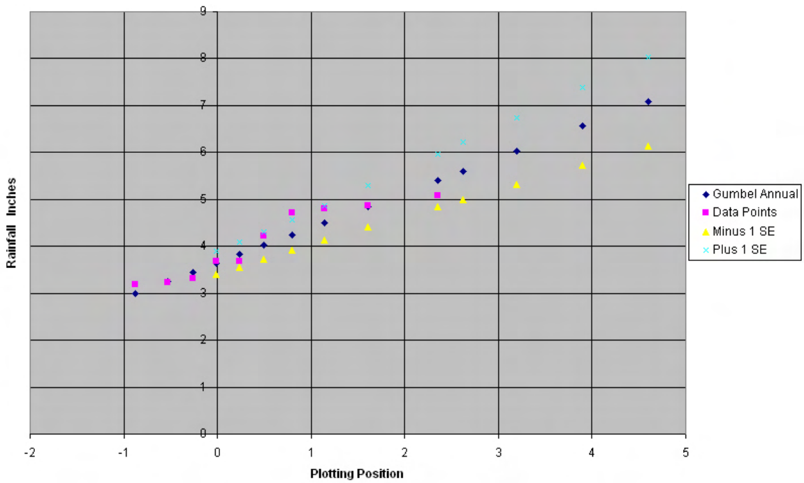
Figure 7-I2. Plot of 6-hour data points versus Gumbel analysis for Chuuk, FSM.
