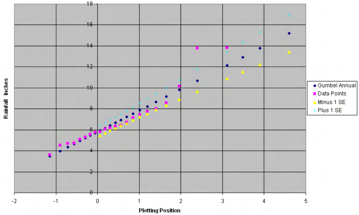
Figure 7-M3. Plot of 24-hour data points versus Gumbel analysis for Koror, Palau.
