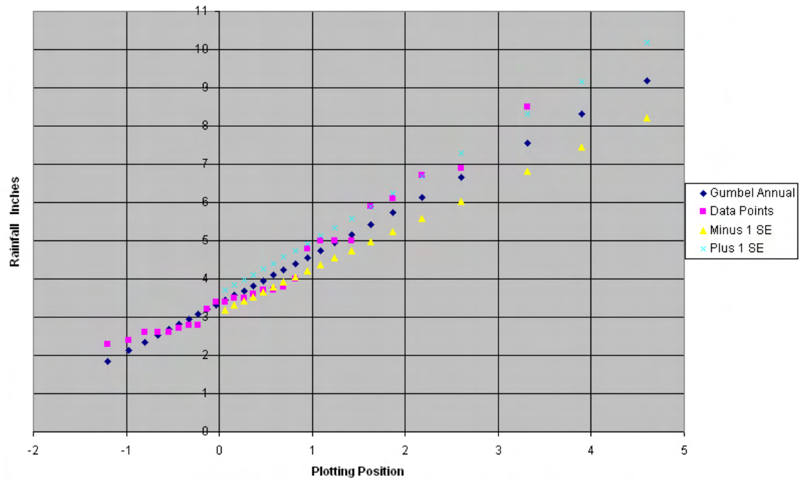
Figure 7-C2. Plot of 6-hour data points versus Gumbel analysis for Piti, Guam.
