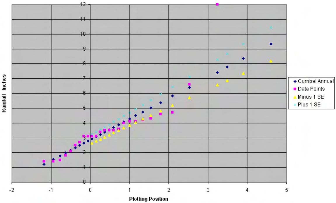
Figure 7-G2. Plot of 6-hour data points versus Gumbel analysis for Saipan IA, CNMI.
