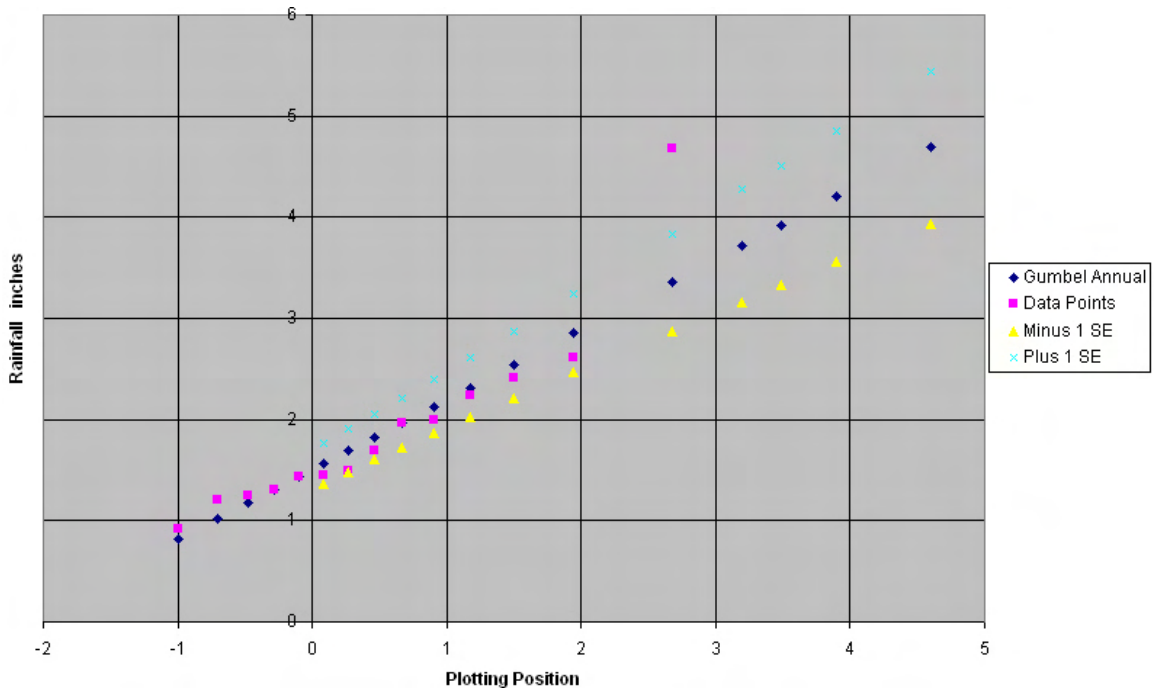
Figure 7-D1. Plot of 1-hour data points versus Gumbel analysis for Taguac, Guam.
