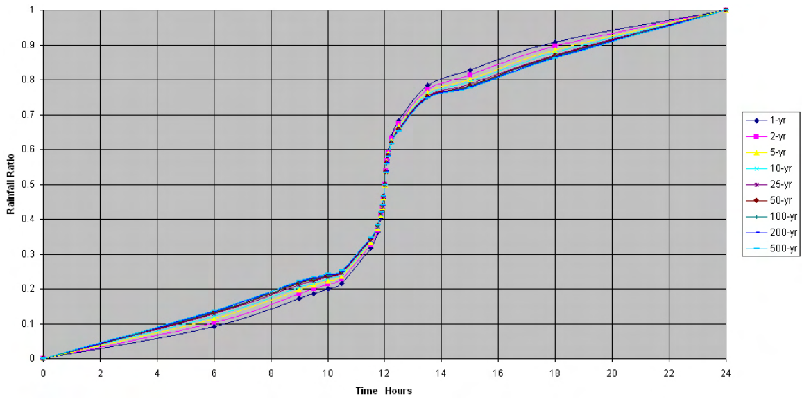
Figure 5-1H. Design rainfall distribution for 1-year to 500-year for Yap WSO (914951), FSM
