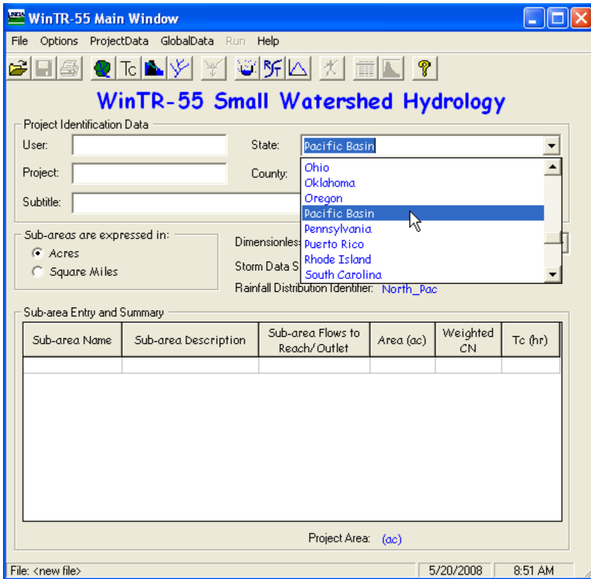
Figure 10. WinTR-55 main input window with “State” selected.
