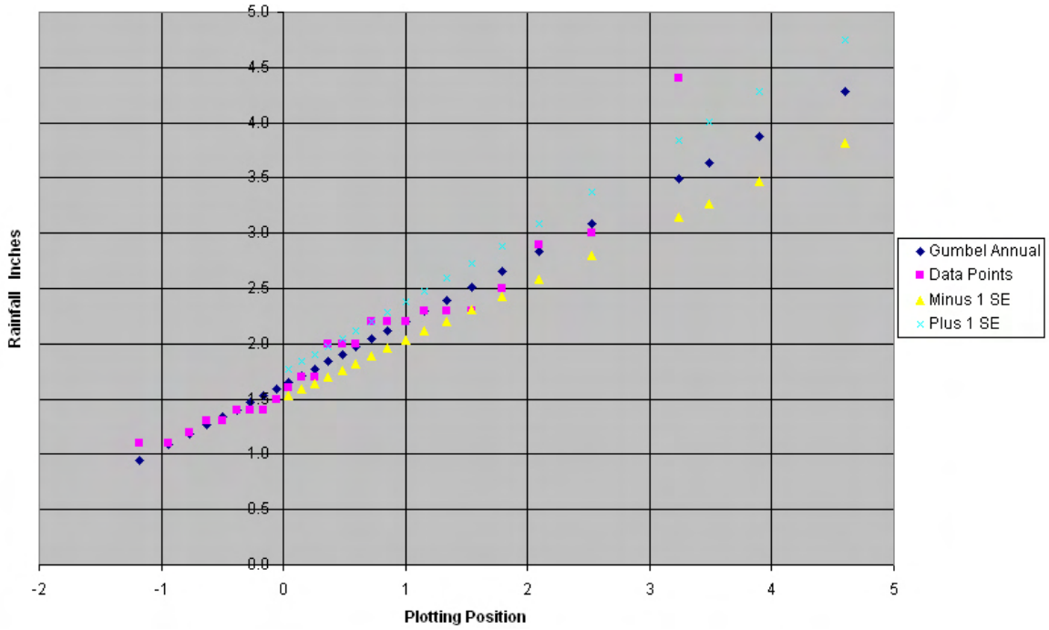
Figure 7-G1. Plot of 1-hour data points versus Gumbel analysis for Saipan IA, CNMI.
