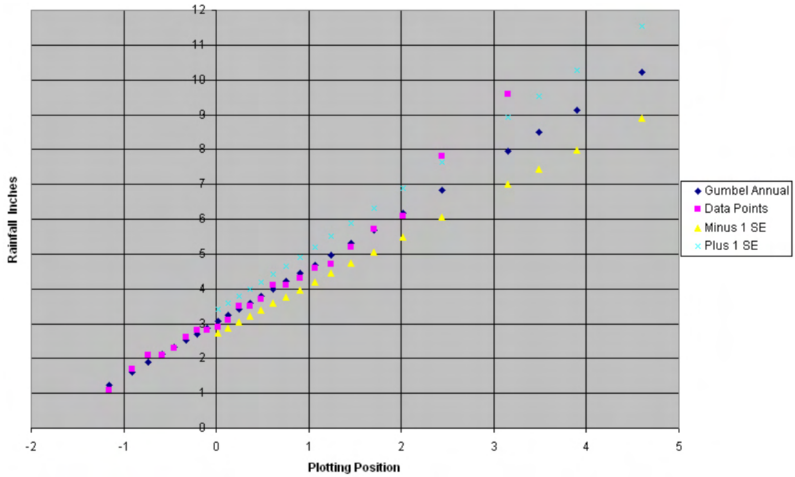
Figure 7-F2. Plot of 6-hour data points versus Gumbel analysis for Rota, CNMI.
