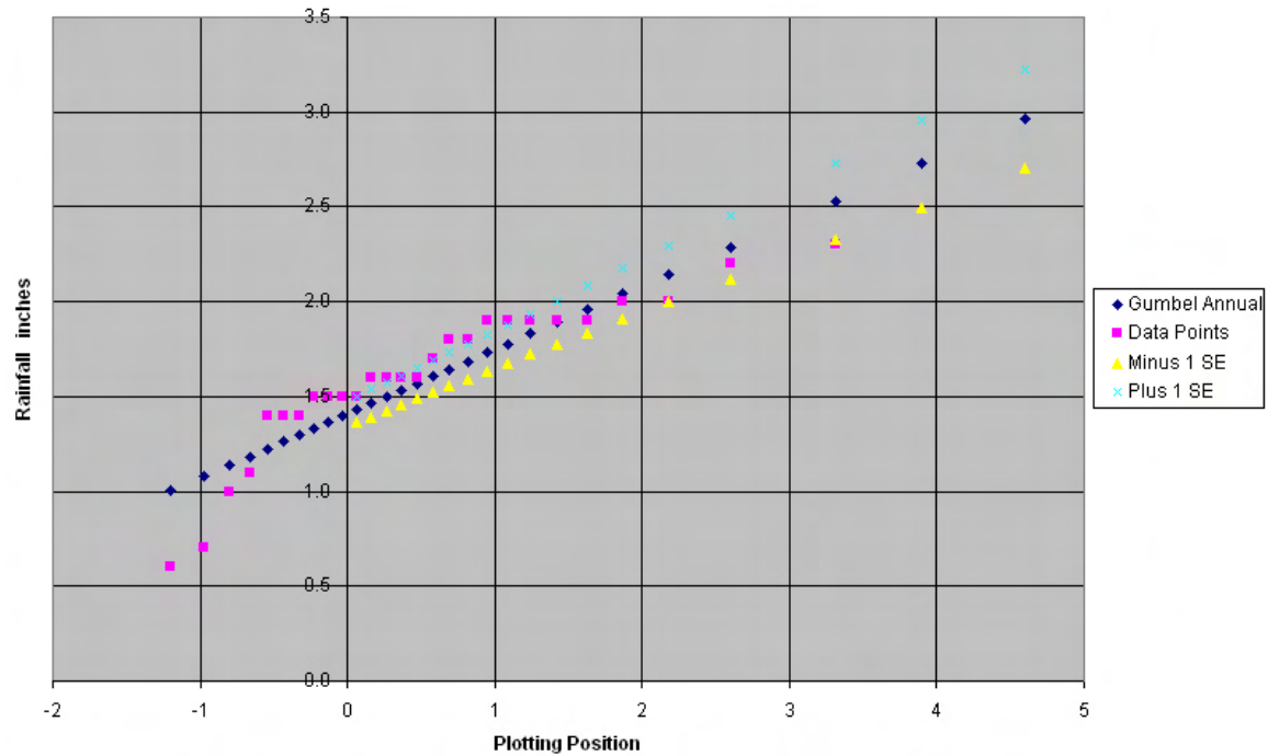
Figure 7-B1. Plot of 1-hour data points versus Gumbel analysis for Inarajan, Guam.
