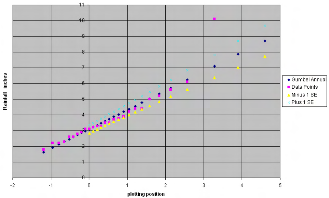
Figure 7-A2. Plot of 6-hour data points versus Gumbel analysis for Fena Lake, Guam.
