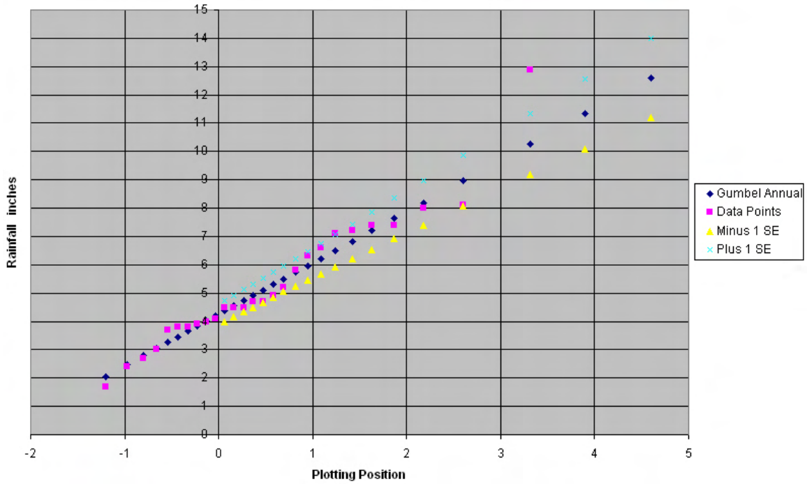
Figure 7-B3. Plot of 24-hour data points versus Gumbel analysis for Inarajan, Guam.
