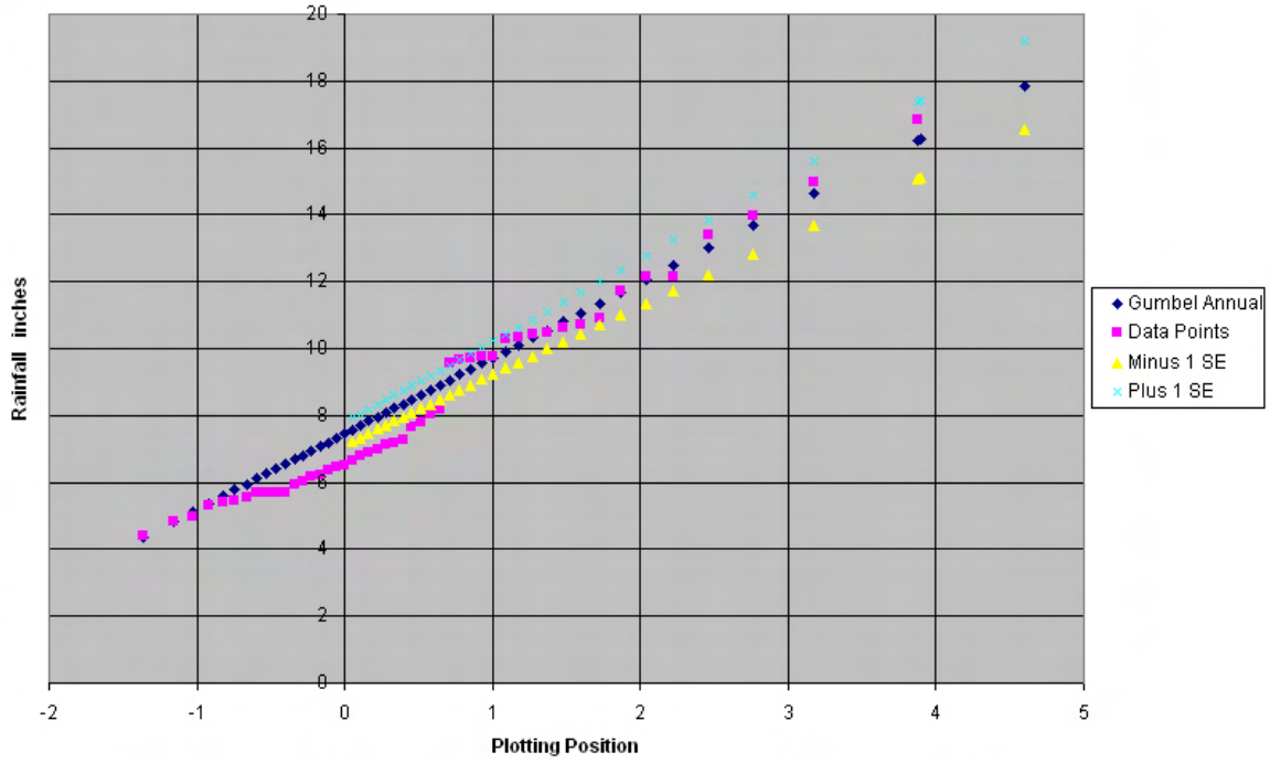
Figure 7-L2. Plot of 48-hour data points versus Gumbel analysis for Kosrae, FSM.
