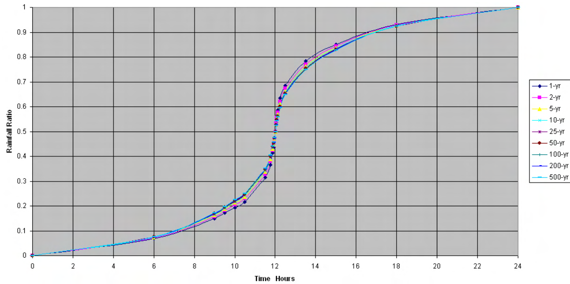
Figure 5-1F. Design rainfall distribution for 1-year to 500-year for Rota (914801), CNMI
