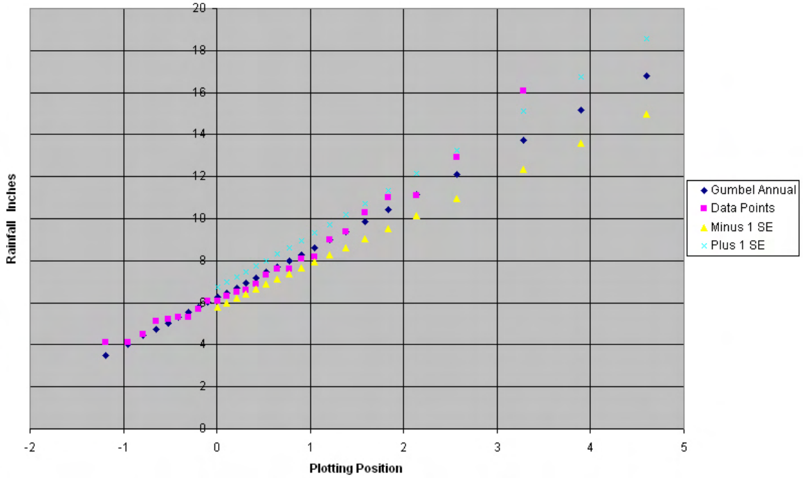
Figure 7-J3. Plot of 24-hour data points versus Gumbel analysis for Pohnpei Hospital, FSM.
