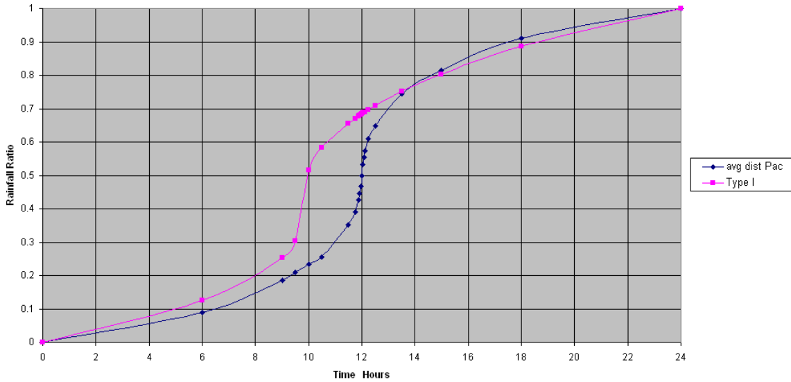
Figure 6-1. Design Rainfall Distribution for Guam, CNMI, Marshall Islands, Wake Island, Federated States of Micronesia.
