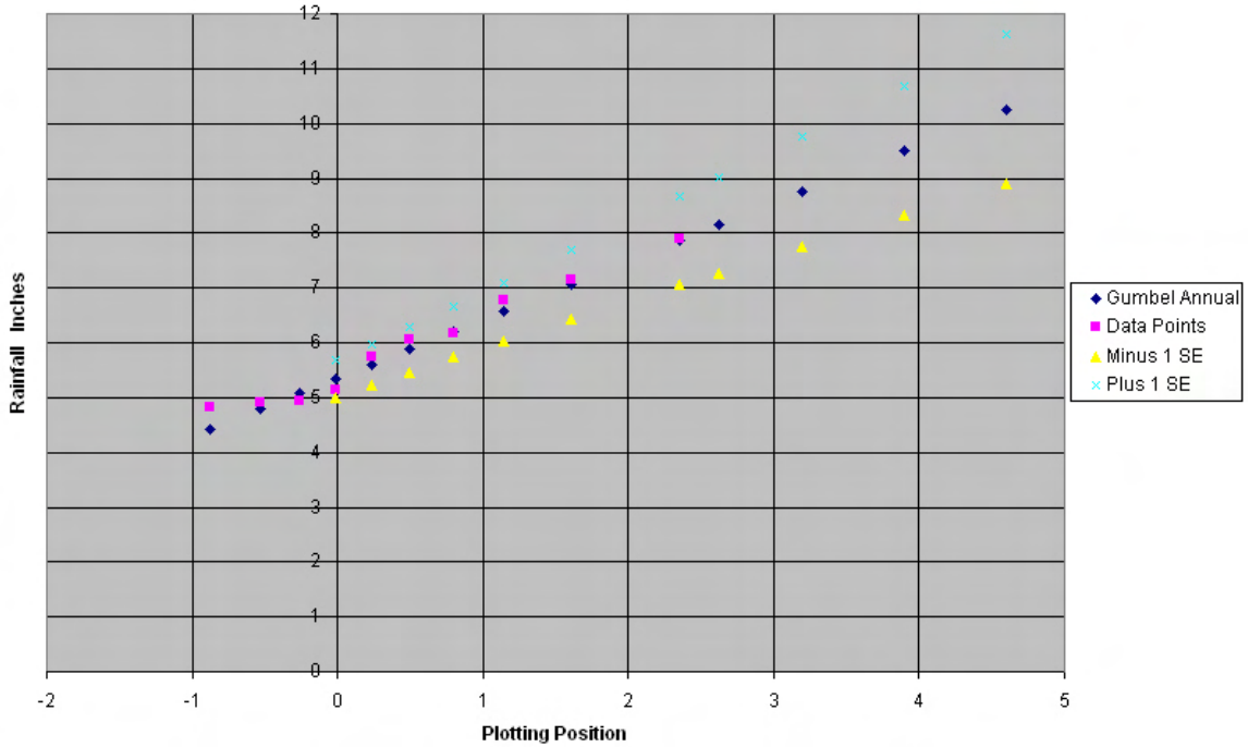
Figure 7-I3. Plot of 24-hour data points versus Gumbel analysis for Chuuk, FSM.
