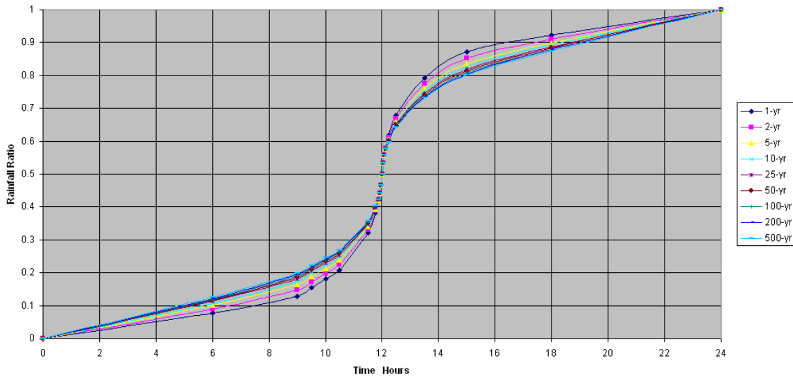
Figure 5-1N. Design rainfall distribution for 1-year to 500-year for Atu'u (914060), Tutuila, American Samoa.
