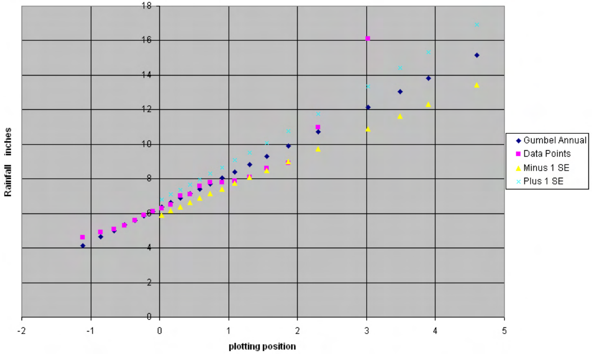
Figure 7-O3. Plot of 24-hour data points versus Gumbel analysis for Atuu, Tutuila, American Samoa.
