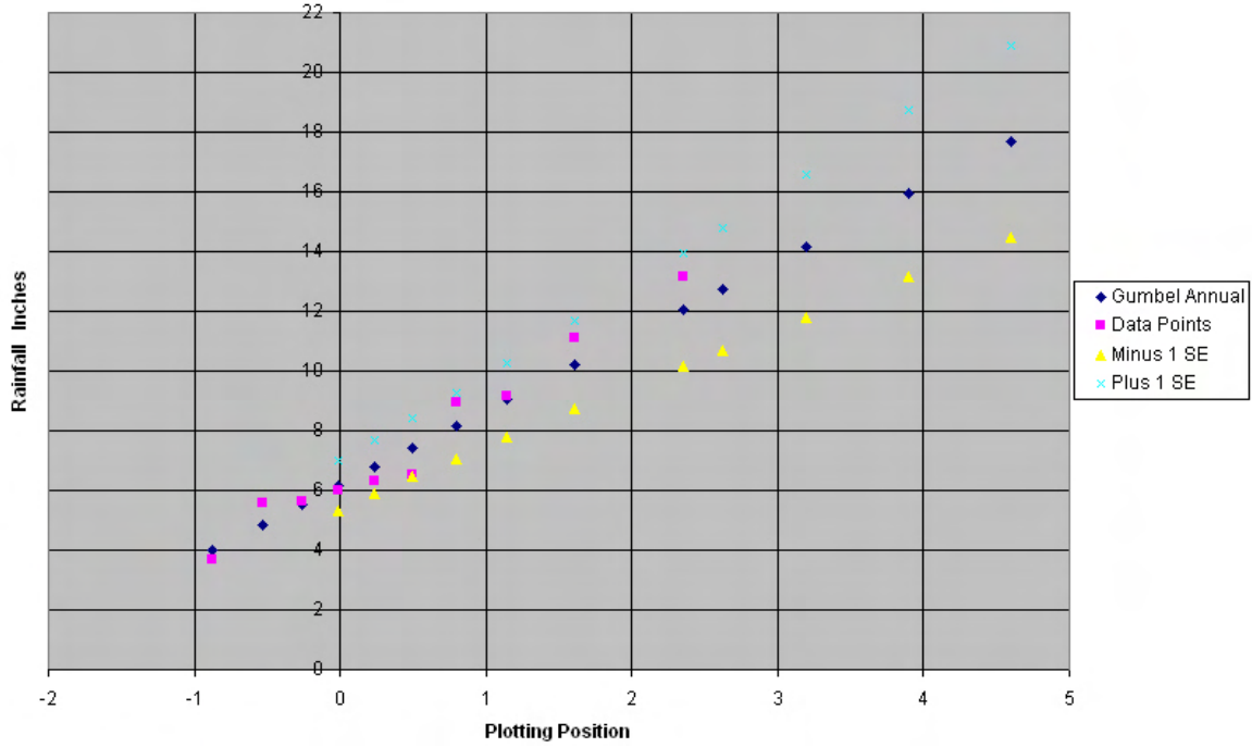
Figure 7-K3. Plot of 24-hour data points versus Gumbel analysis for Pohnpei WSO, FSM.
