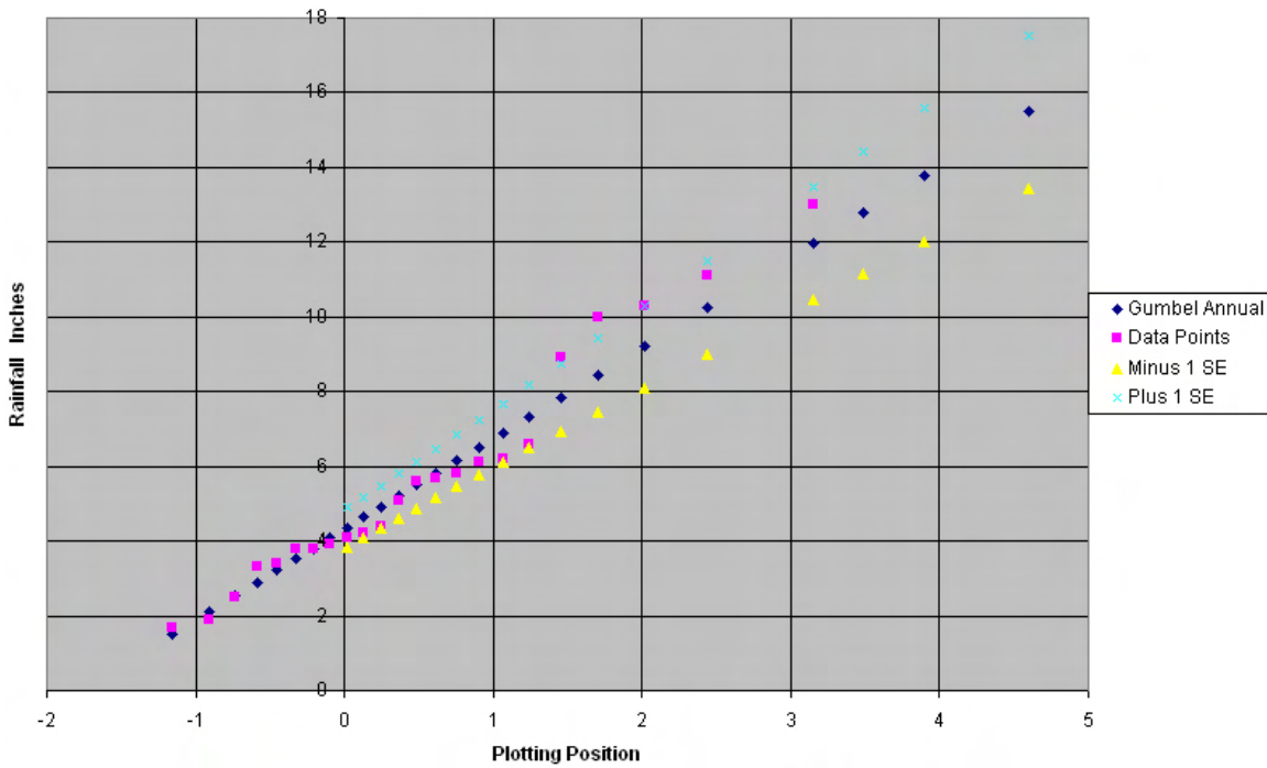
Figure 7-F3. Plot of 24-hour data points versus Gumbel analysis for Rota, CNMI.
