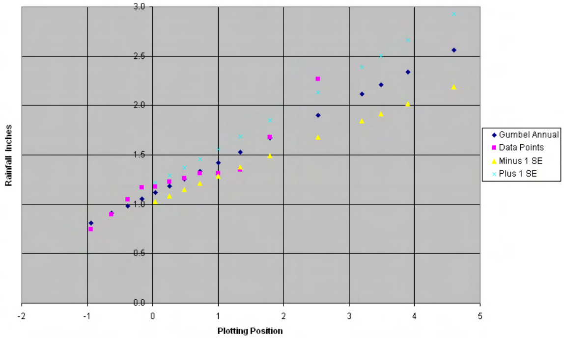
Figure 7-Q1. Plot of 1-hour data points versus Gumbel analysis for Wake Island.
