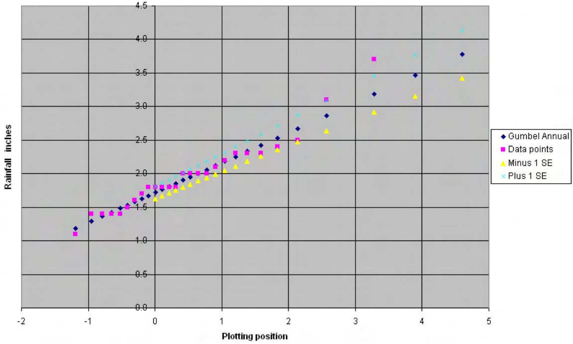
Figure 7-A1. Plot of 1-hour data points versus Gumbel analysis for Fena Lake, Guam.
