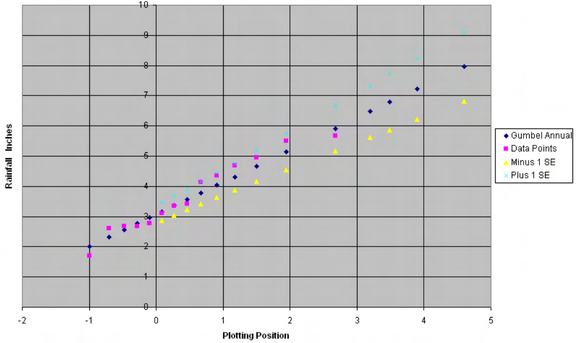
Figure 7-D2. Plot of 6-hour data points versus Gumbel analysis for Taguac, Guam.
