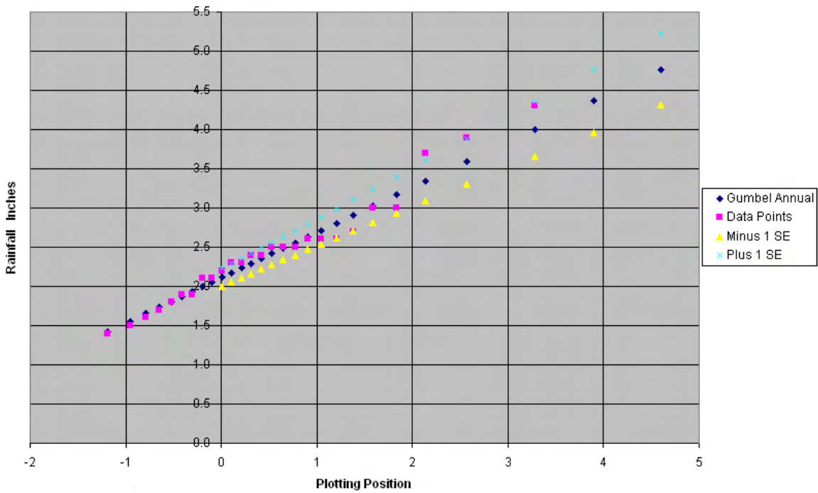
Figure 7-J1. Plot of 1-hour data points versus Gumbel analysis for Pohnpei Hospital, FSM.
