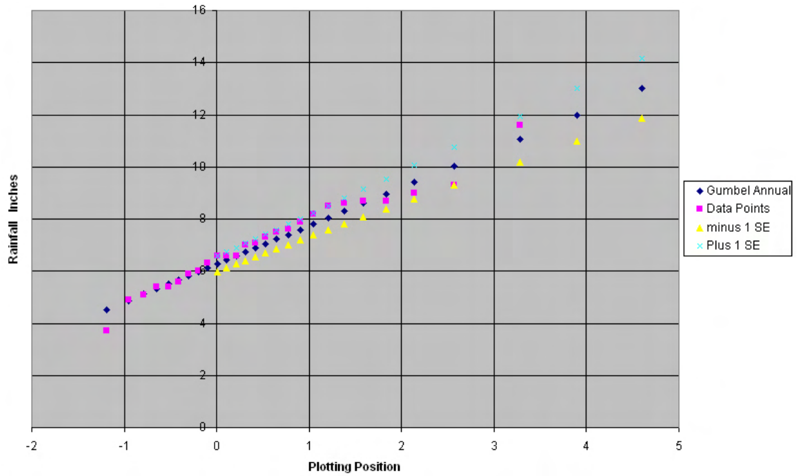
Figure 7-P3. Plot of 24-hour data points versus Gumbel analysis for Malaeloa, Tutuila, American Samoa.
