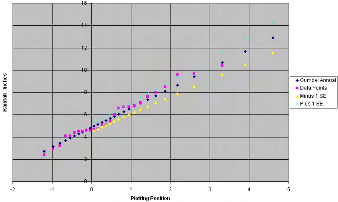
Figure 7-C3. Plot of 24-hour data points versus Gumbel analysis for Piti, Guam.
