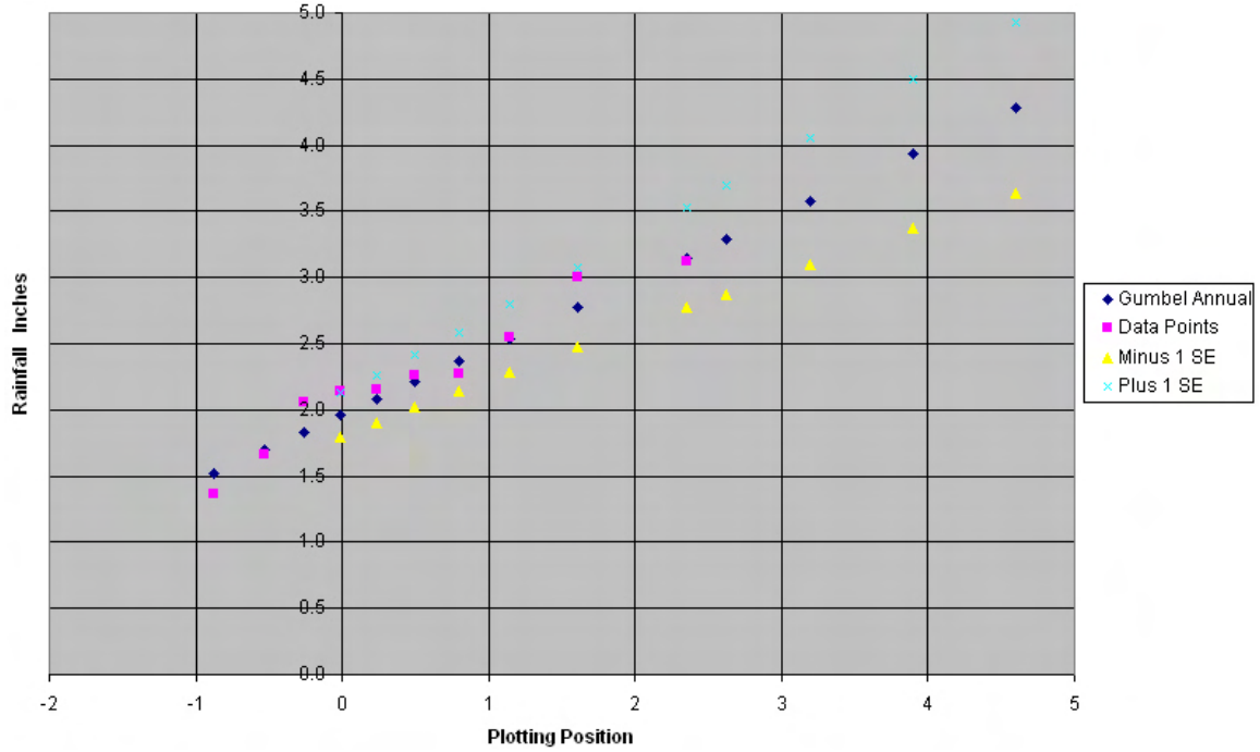
Figure 7-K1. Plot of 1-hour data points versus Gumbel analysis for Pohnpei WSO, FSM.
