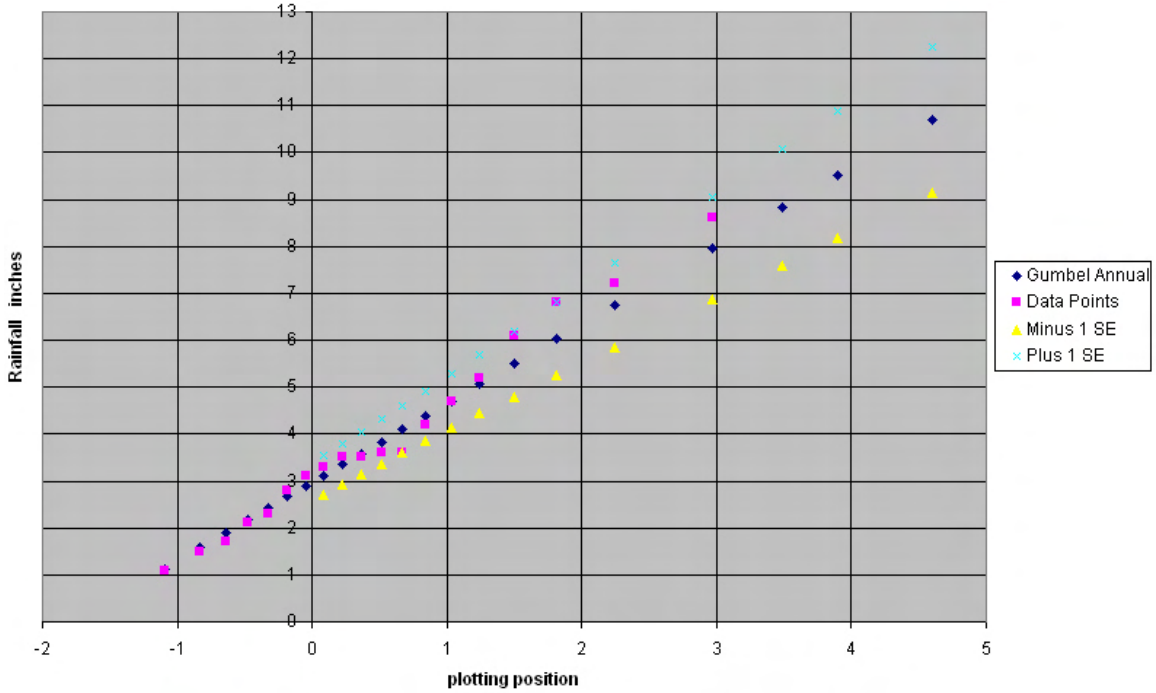
Figure 7-E3. Plot of 24-hour data points versus Gumbel analysis for Capitol Hill, CNMI.
