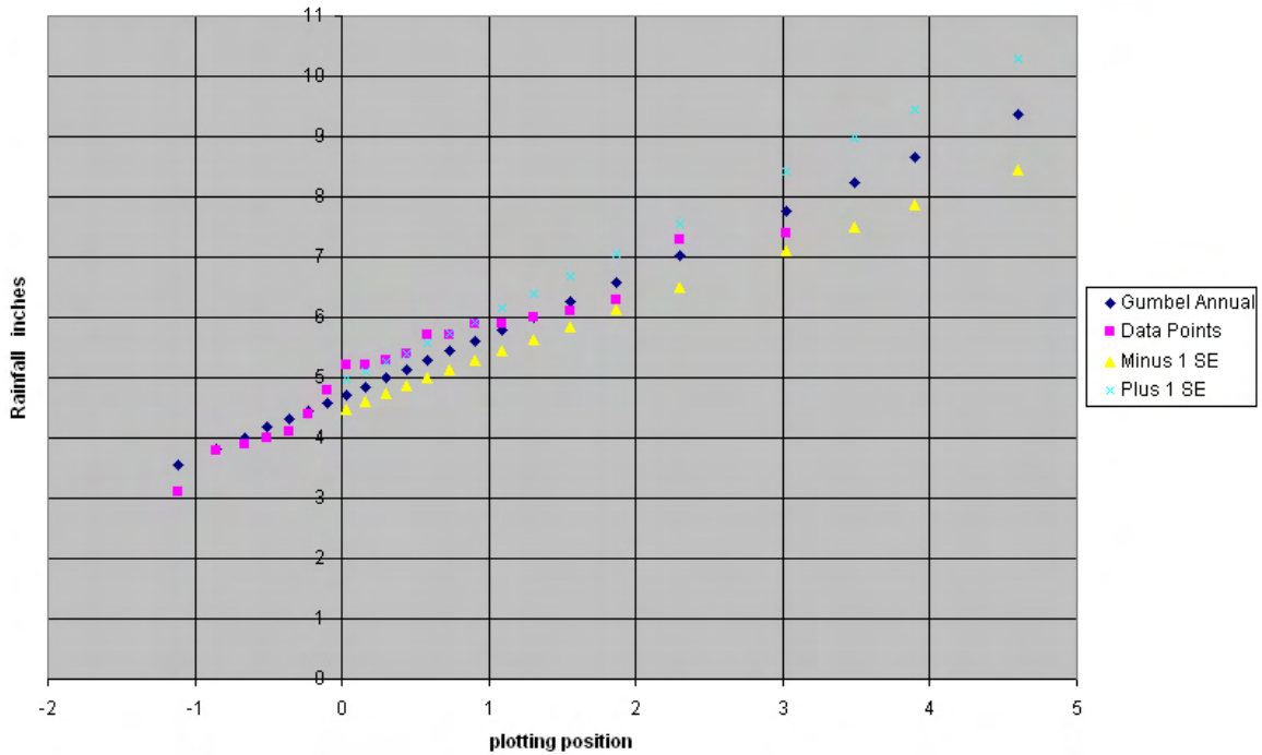
Figure 7-O2. Plot of 6-hour data points versus Gumbel analysis for Atuu, Tutuila, American Samoa.
