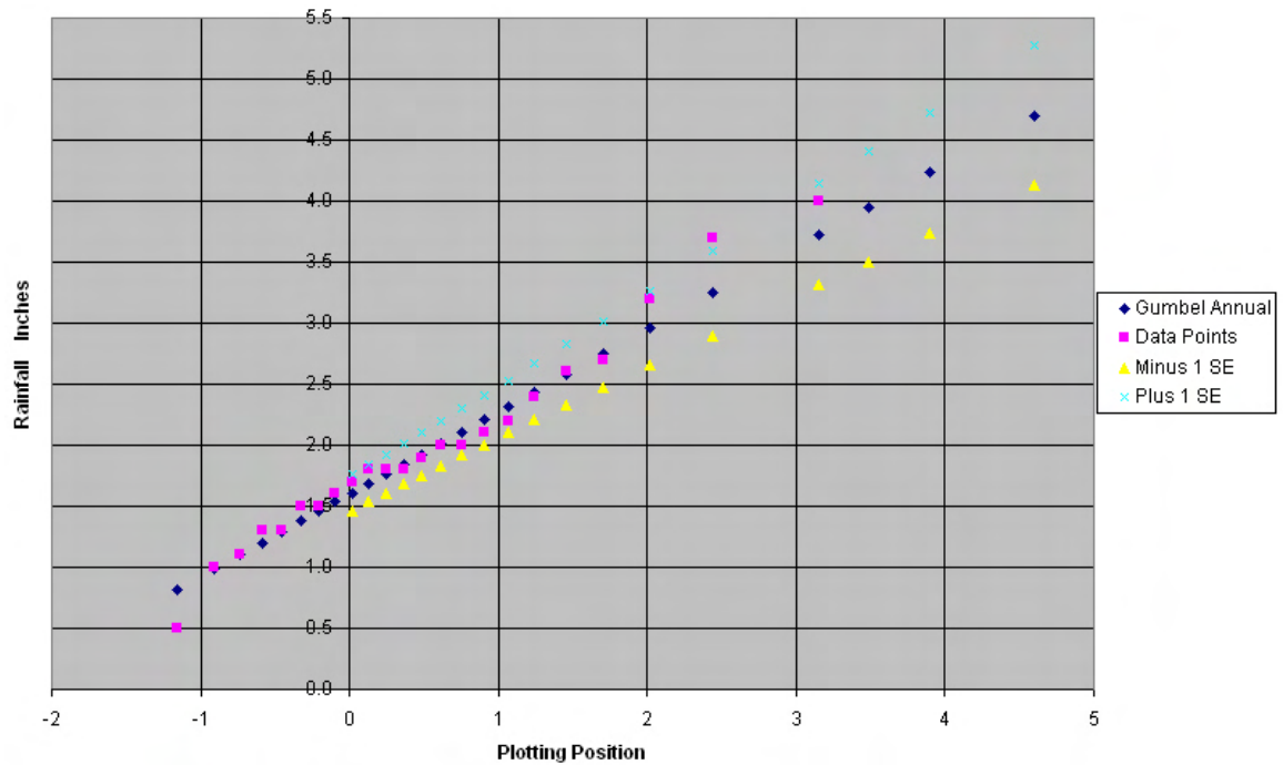
Figure 7-F1. Plot of 1-hour data points versus Gumbel analysis for Rota, CNMI.
