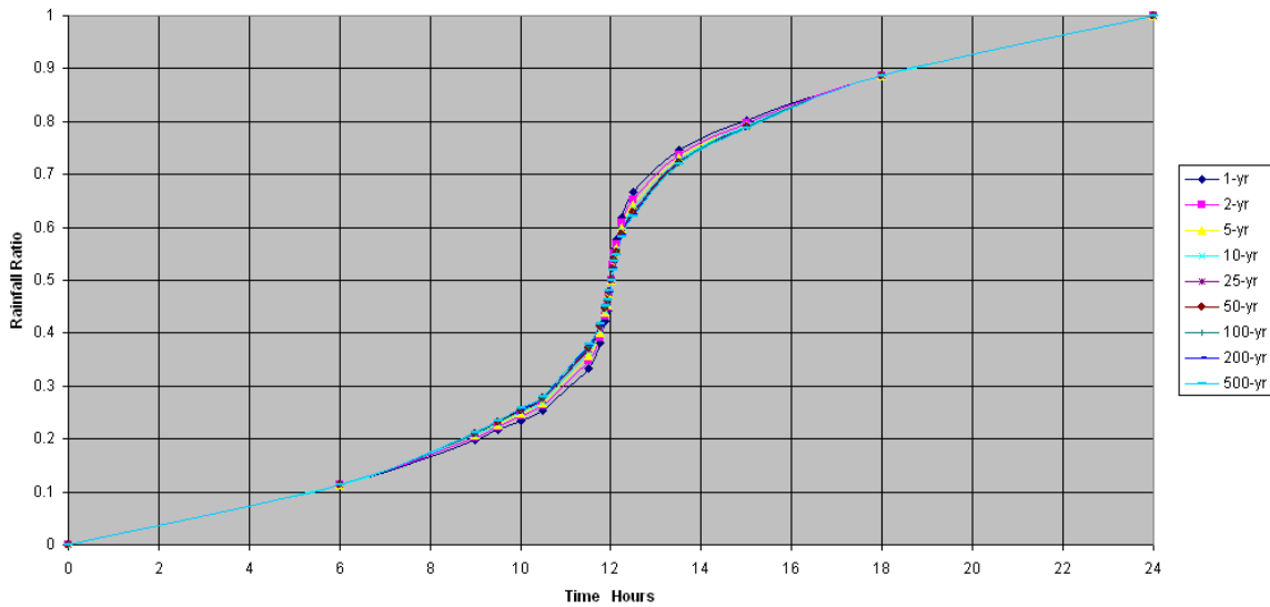
Figure 5-1A. Design rainfall distribution for 1-year to 500-year for Fena Lake (914200), Guam
