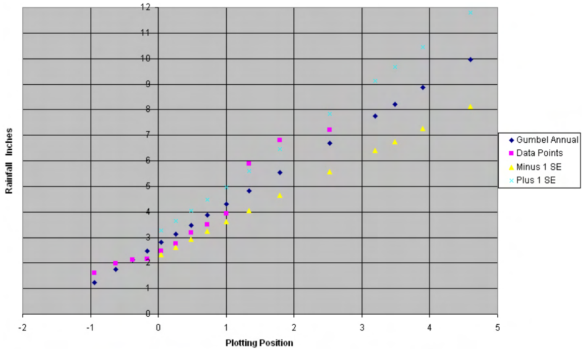
Figure 7-Q3. Plot of 24-hour data points versus Gumbel analysis for Wake Island.
