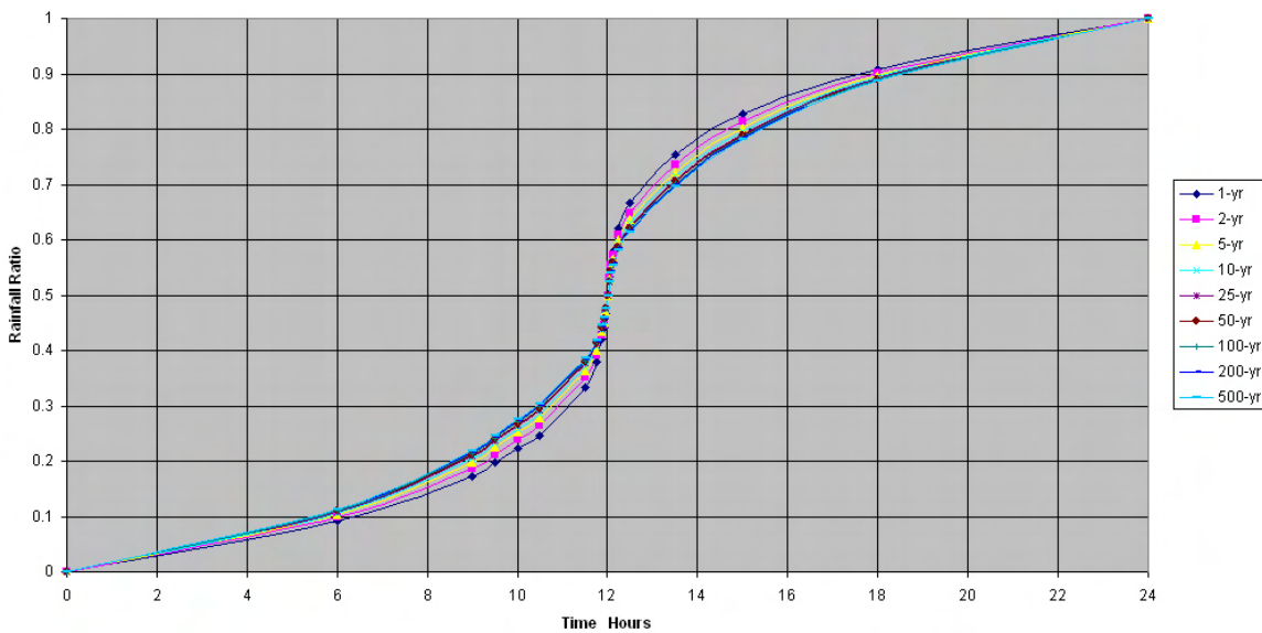
Figure 5-1B. Design rainfall distribution for 1-year to 500-year for Inarajan (914278), Guam
