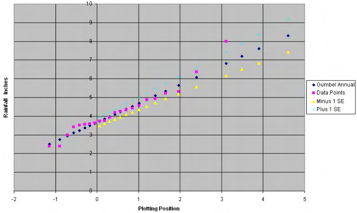
Figure 7-N2. Plot of 6-hour data points versus Gumbel analysis for Majuro, Marshall Islands (1984-2005).
