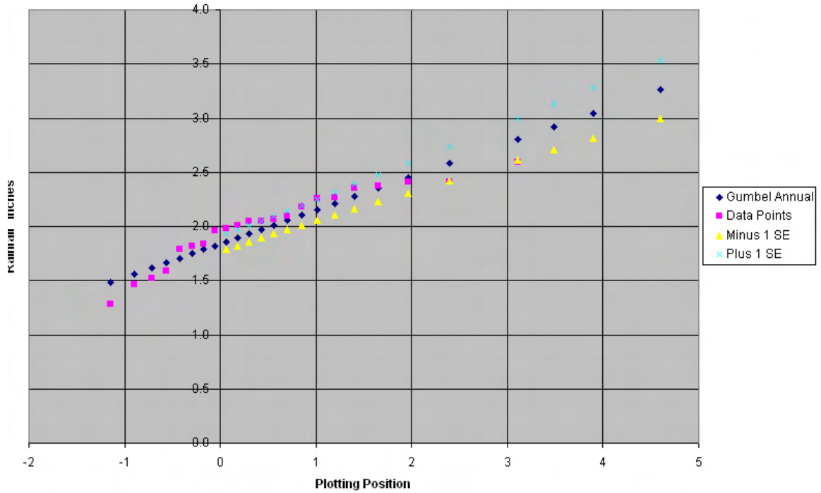
Figure 7-N1. Plot of 1-hour data points versus Gumbel analysis for Majuro, Marshall Islands (1984-2005).
