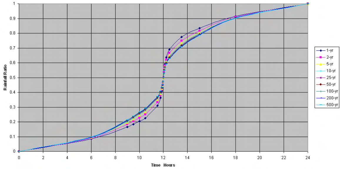
Figure 5-1G. Design rainfall distribution for 1-year to 500-year for Saipan International Airport (914855), CNMI
