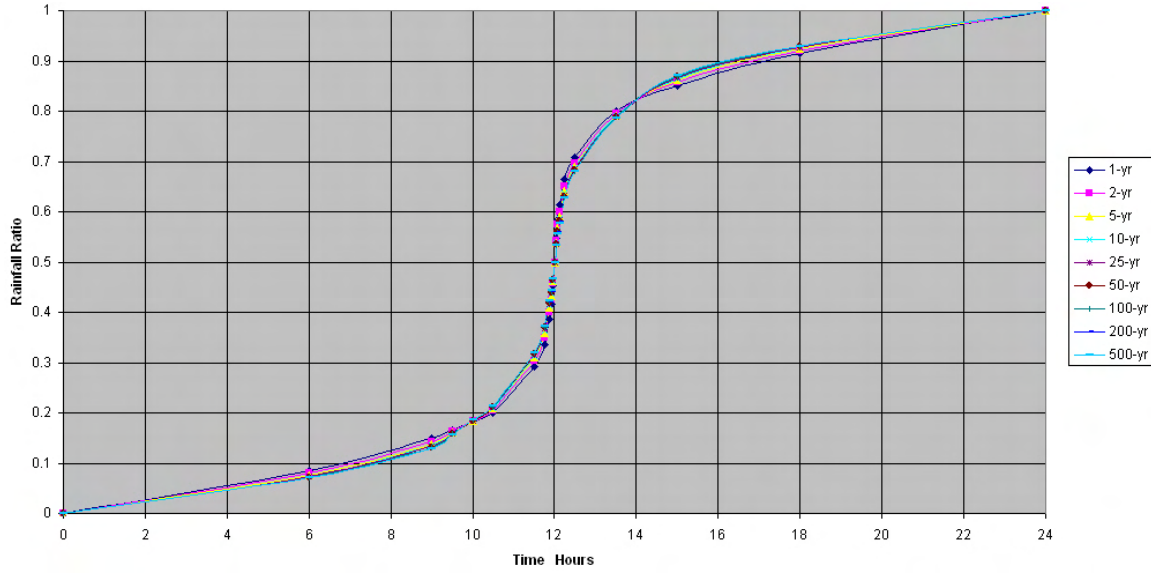
Figure 5-1E. Design rainfall distribution for 1-year to 500-year for Capitol Hill (914080), Saipan, CNMI.
