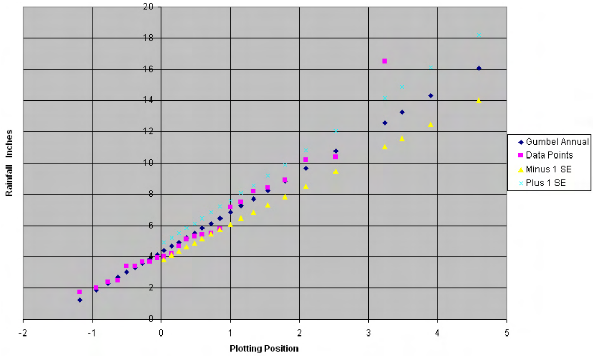
Figure 7-G3. Plot of 24-hour data points versus Gumbel analysis for Saipan IA, CNMI.
