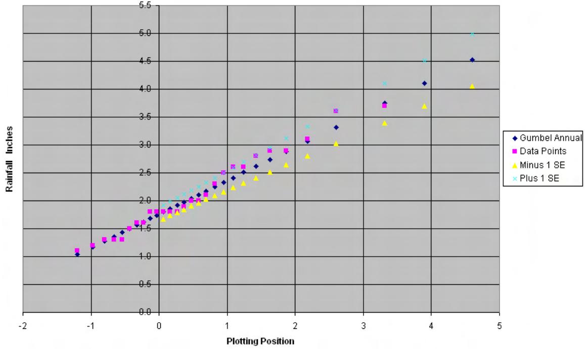
Figure 7-C1. Plot of 1-hour data points versus Gumbel analysis for Piti, Guam.
