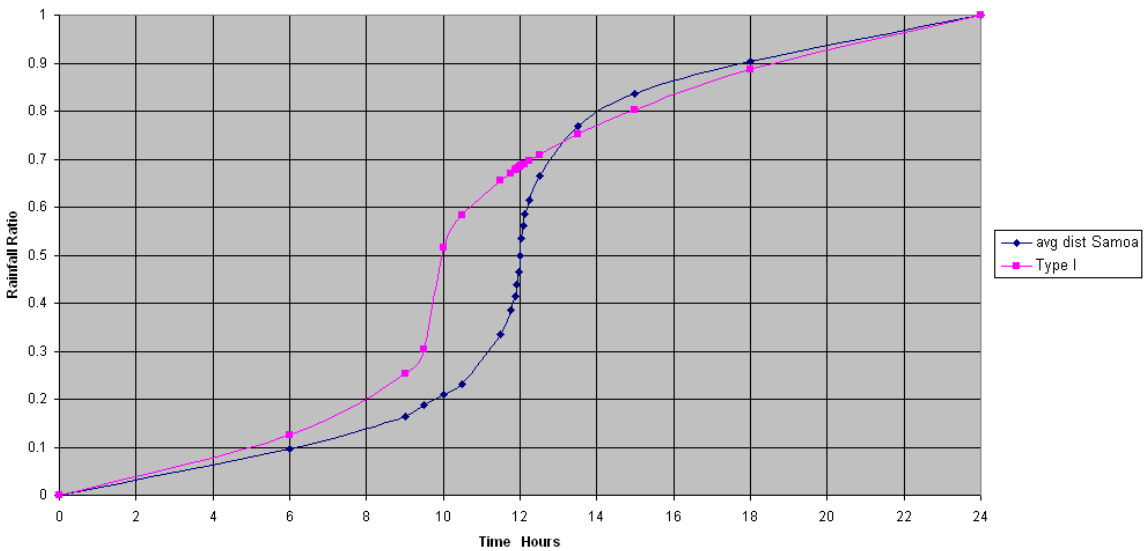
Figure 6-2. Design Rainfall Distribution for Tutuila, American Samoa.
