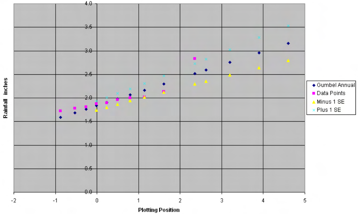
Figure 7-I1. Plot of 1-hour data points versus Gumbel analysis for Chuuk, FSM.
