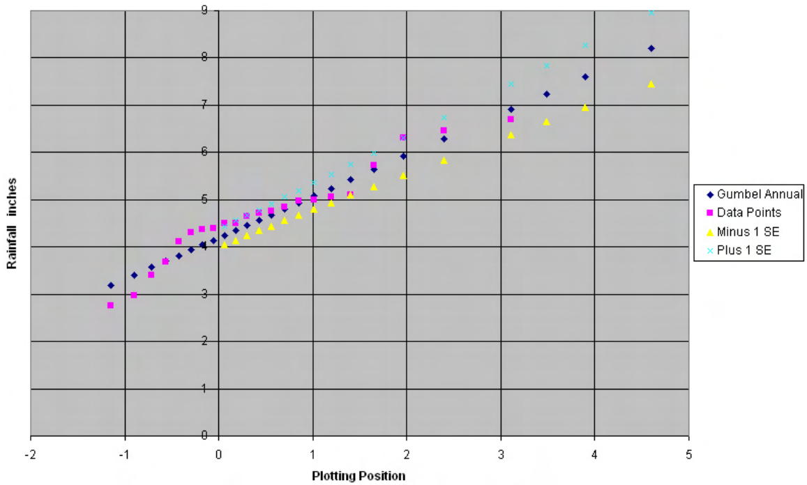
Figure 7-M2. Plot of 6-hour data points versus Gumbel analysis for Koror, Palau.
