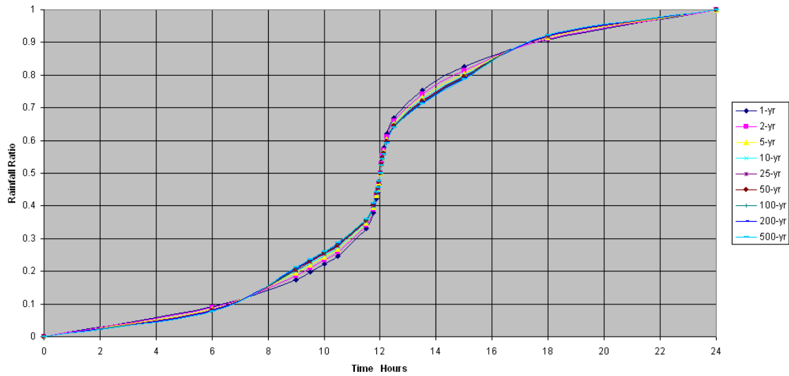
Figure 5-1J. Design rainfall distribution for 1-year to 500-year for Pohnpei Hospital (914745), FSM
