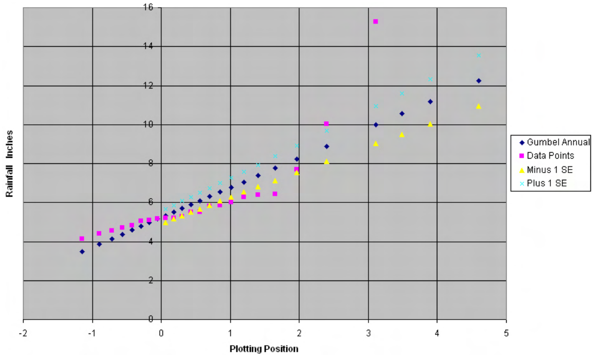
Figure 7-N3. Plot of 24-hour data points versus Gumbel analysis for Majuro, Marshall Islands (1984-2005).
