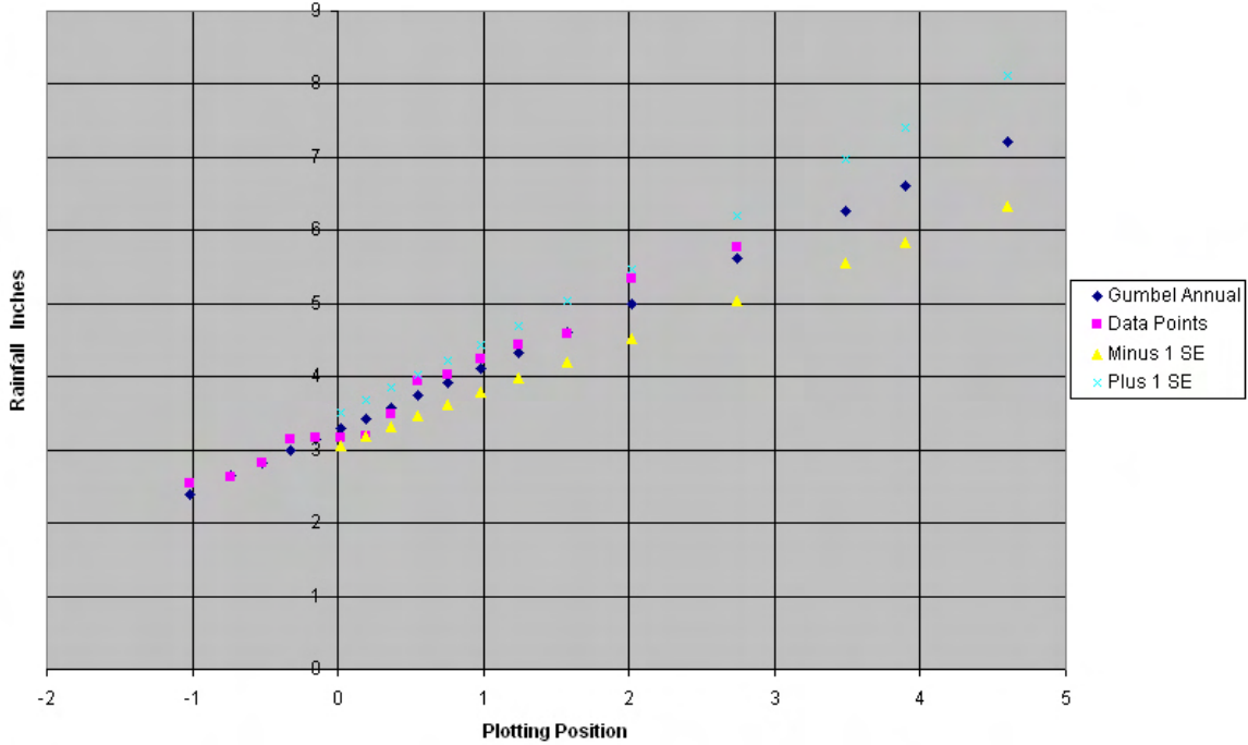
Figure 7-H2. Plot of 6-hour data points versus Gumbel analysis for Yap, FSM.
