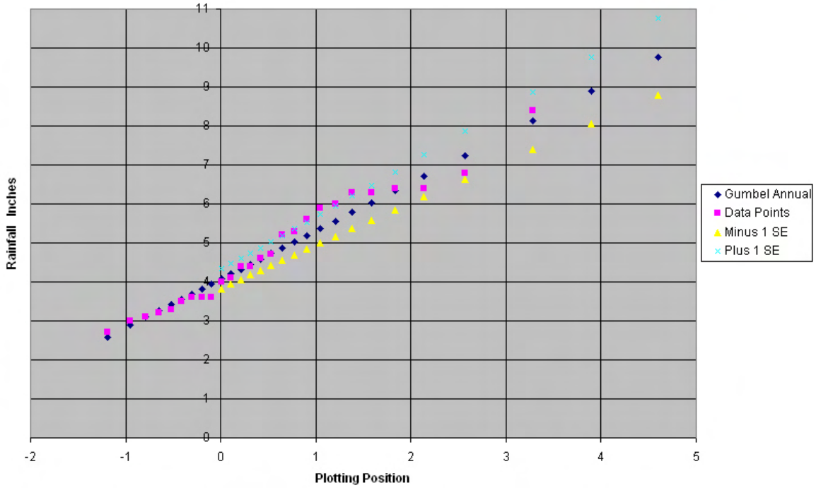
Figure 7-J2. Plot of 6-hour data points versus Gumbel analysis for Pohnpei Hospital, FSM.
