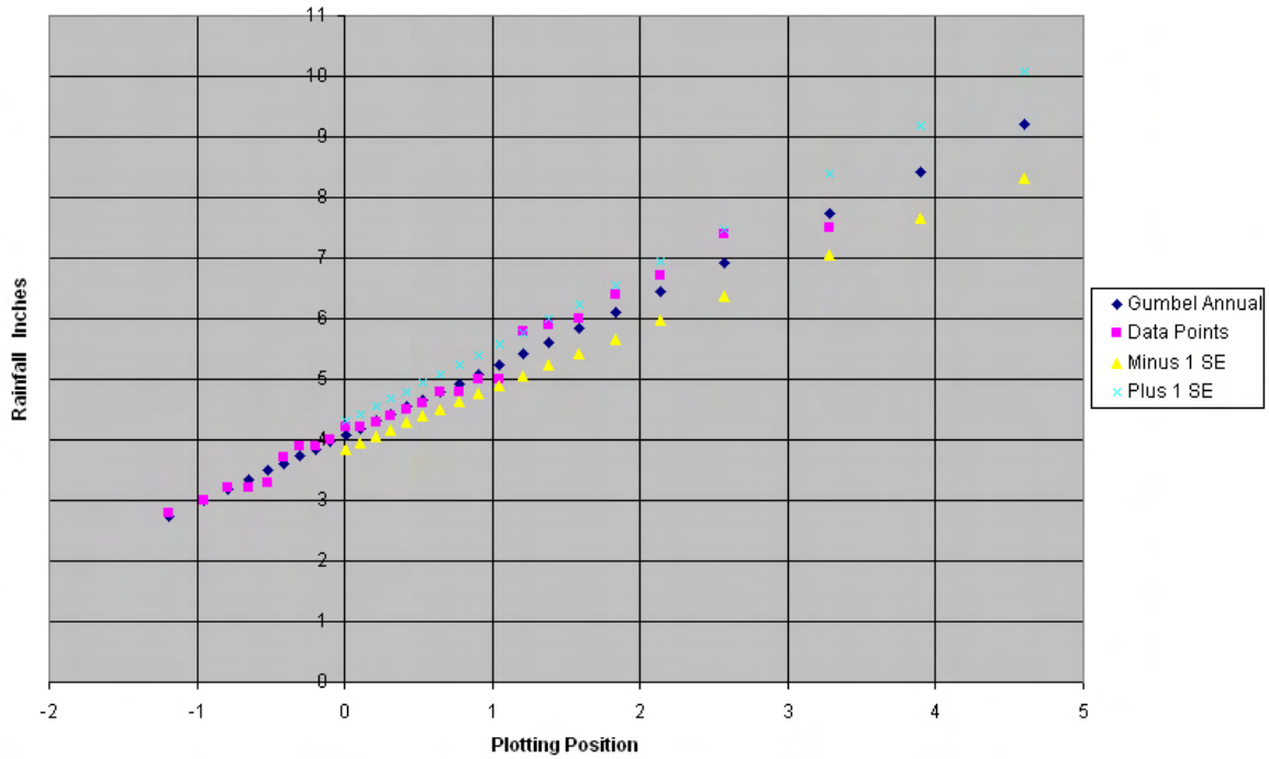
Figure 7-P2. Plot of 6-hour data points versus Gumbel analysis for Malaeloa, Tutuila, American Samoa.
