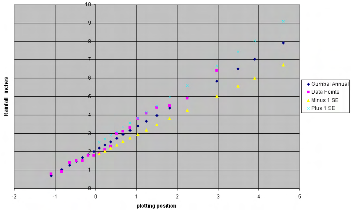
Figure 7-E2. Plot of 6-hour data points versus Gumbel analysis for Capitol Hill, CNMI.
