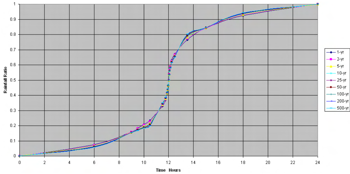
Figure 5-1I. Design rainfall distribution for 1-year to 500-year for Chuuk (914851), FSM
