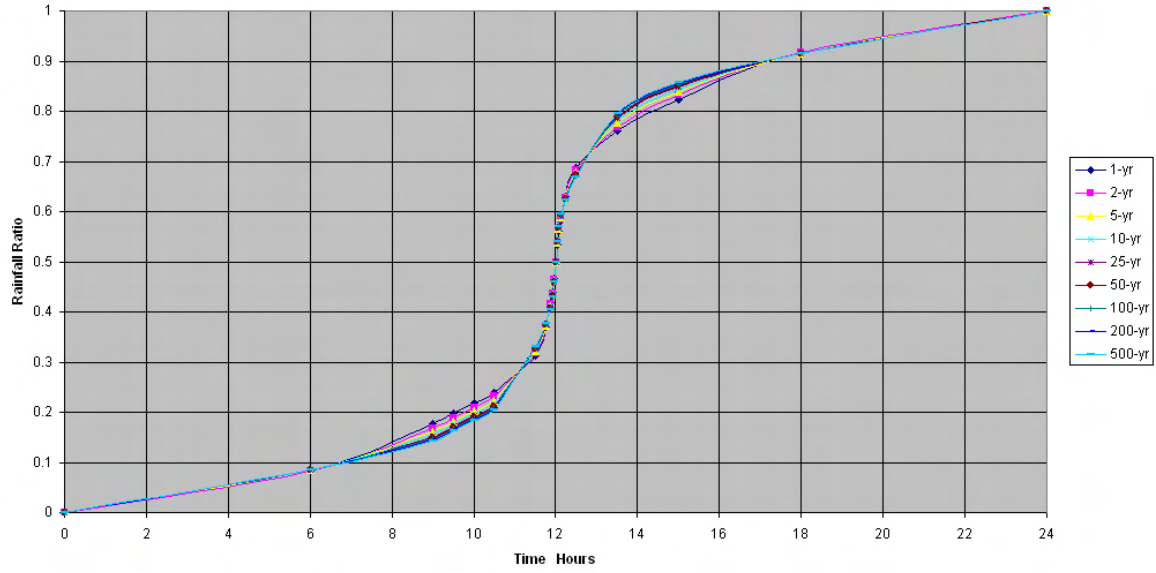
Figure 5-1O. Design rainfall distribution for 1-year to 500-year for Malaeloa (914594), Tutuila, American Samoa.
