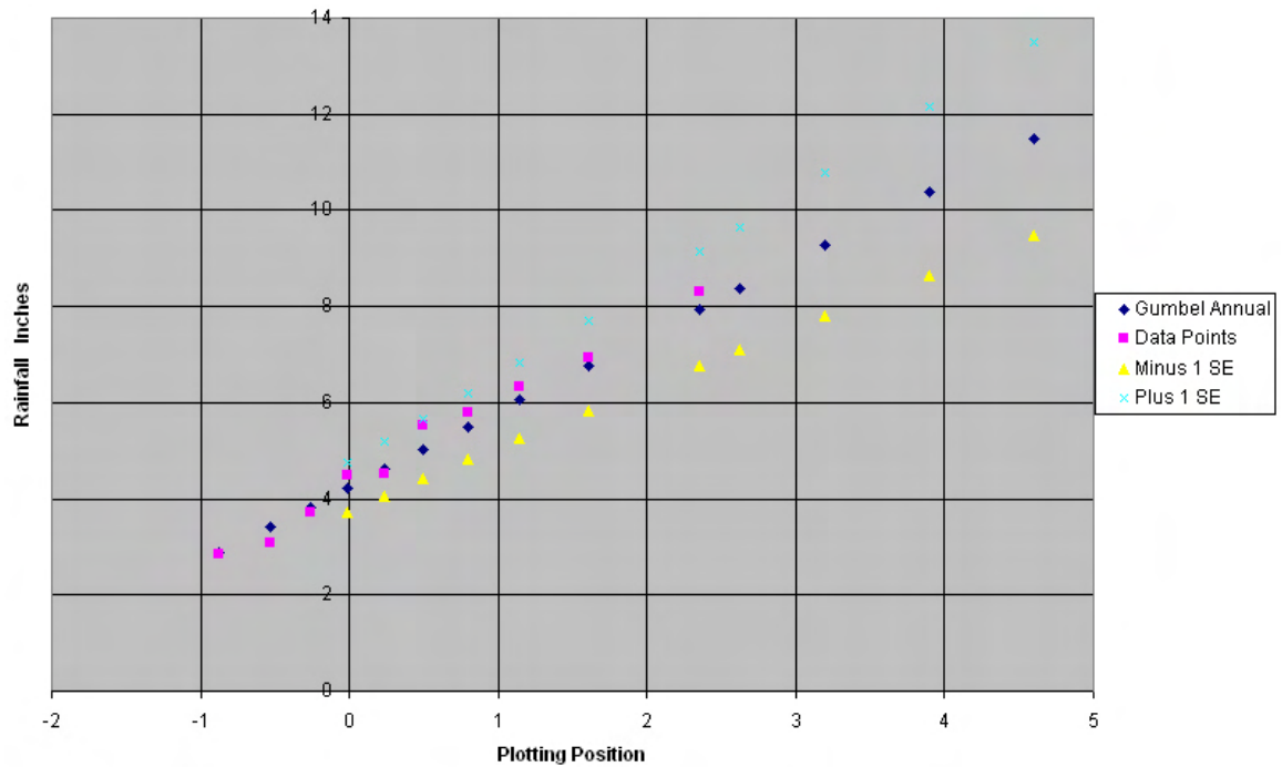
Figure 7-K2. Plot of 6-hour data points versus Gumbel analysis for Pohnpei WSO, FSM.
