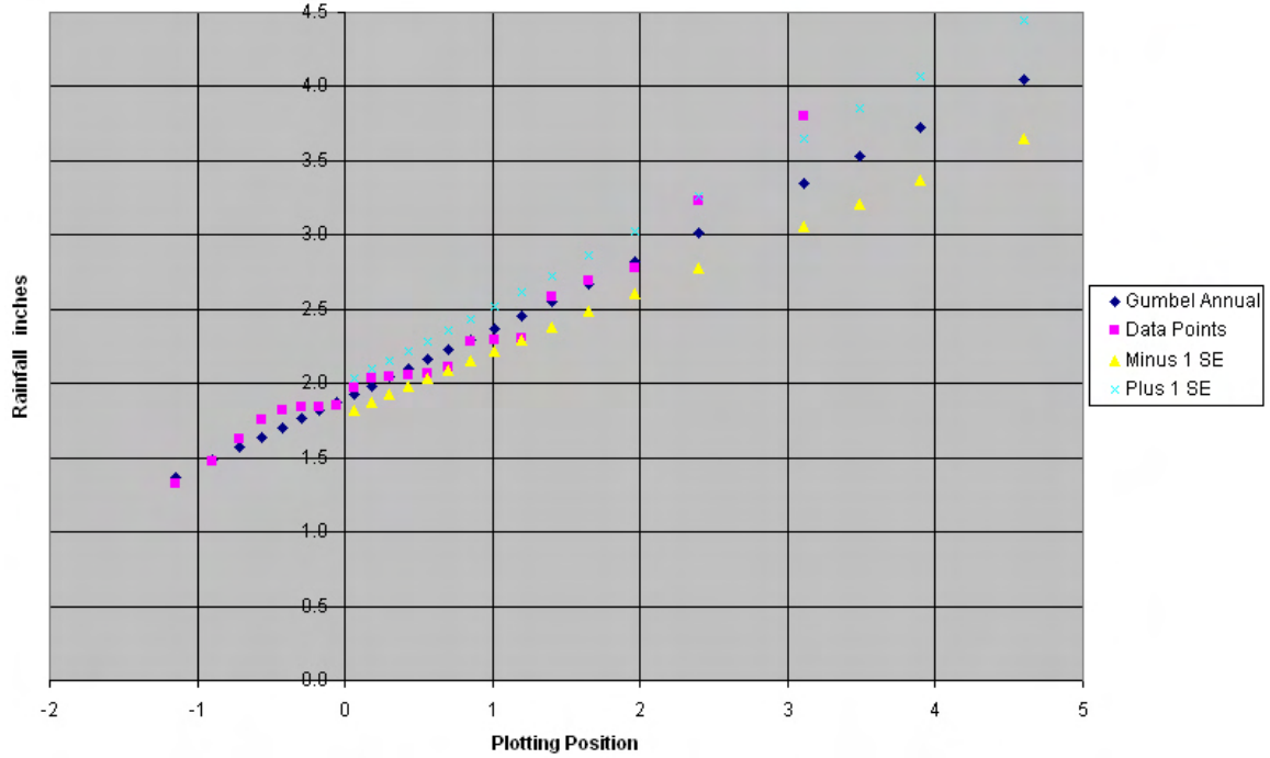
Figure 7-M1. Plot of 1-hour data points versus Gumbel analysis for Koror, Palau.
