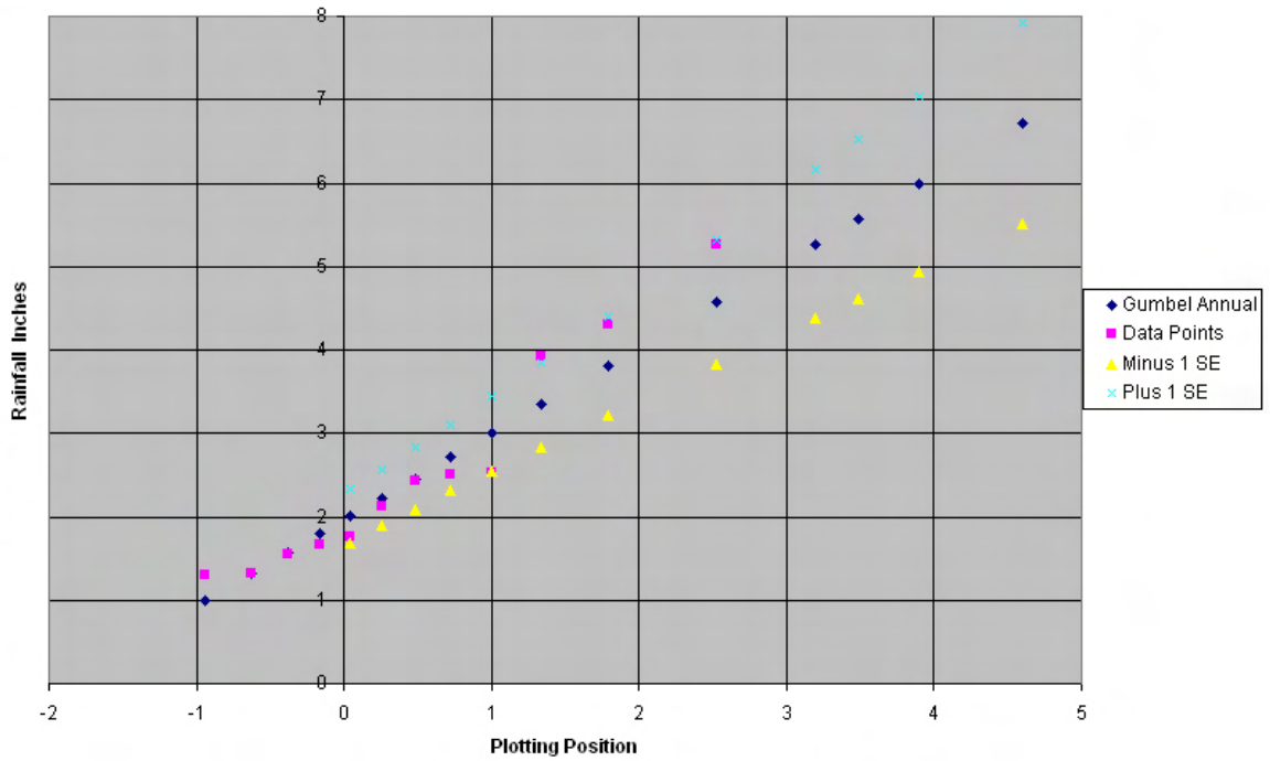
Figure 7-Q2. Plot of 6-hour data points versus Gumbel analysis for Wake Island.
