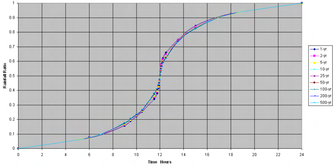
Figure 5-1K. Design rainfall distribution for 1-year to 500-year for Pohnpei WSO (914751), FSM
