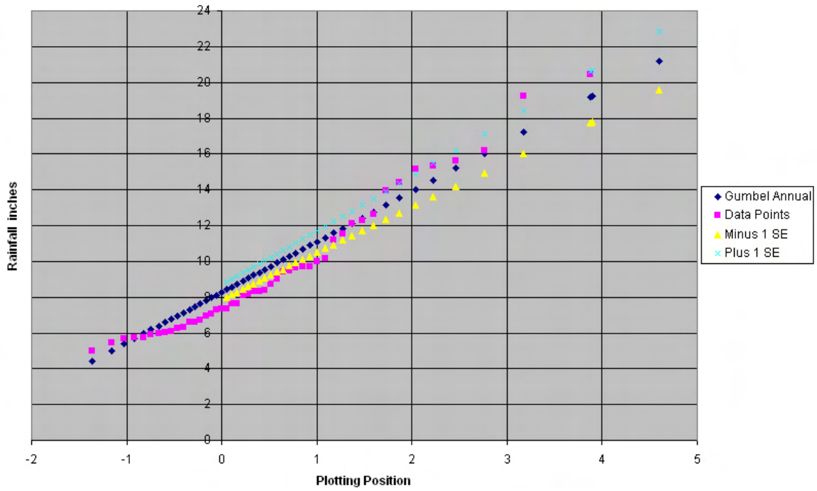
Figure 7-L3. Plot of 72-hour data points versus Gumbel analysis for Kosrae, FSM.
