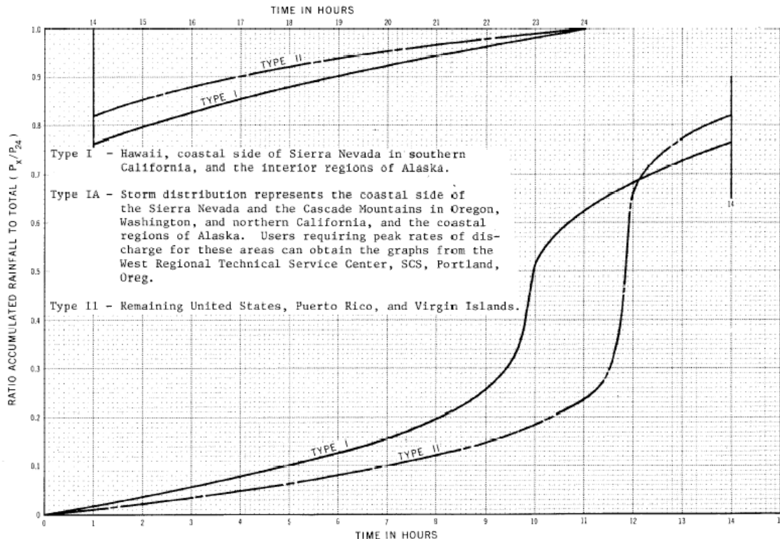
Figure 2. Type I and Type II rainfall distributions from TP-149.
