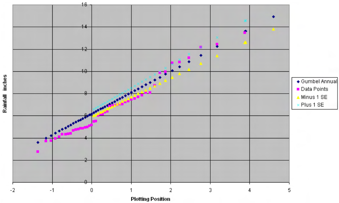
Figure 7-L1. Plot of 24-hour data points versus Gumbel analysis for Kosrae, FSM.
