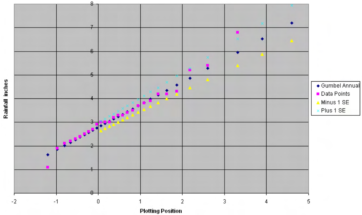
Figure 7-B2. Plot of 6-hour data points versus Gumbel analysis for Inarajan, Guam.
