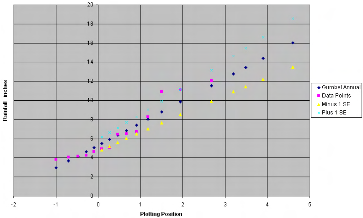
Figure 7-D3. Plot of 24-hour data points versus Gumbel analysis for Taguac, Guam.
