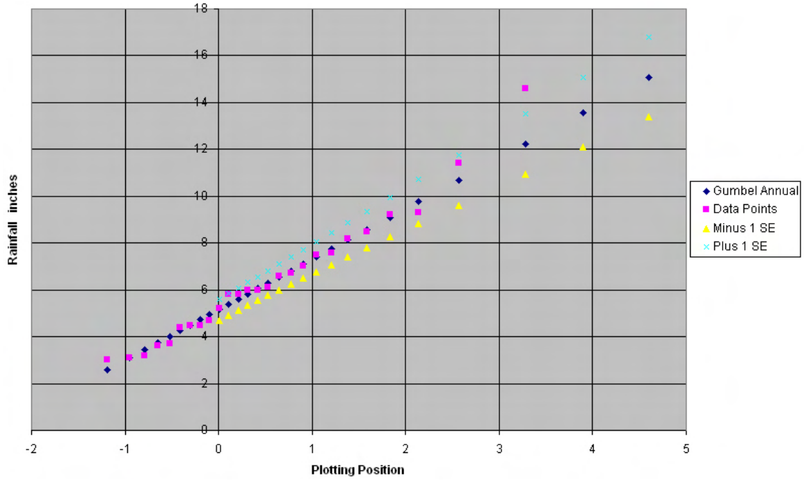
Figure 7-A3. Plot of 24-hour data points versus Gumbel analysis for Fena Lake, Guam.
