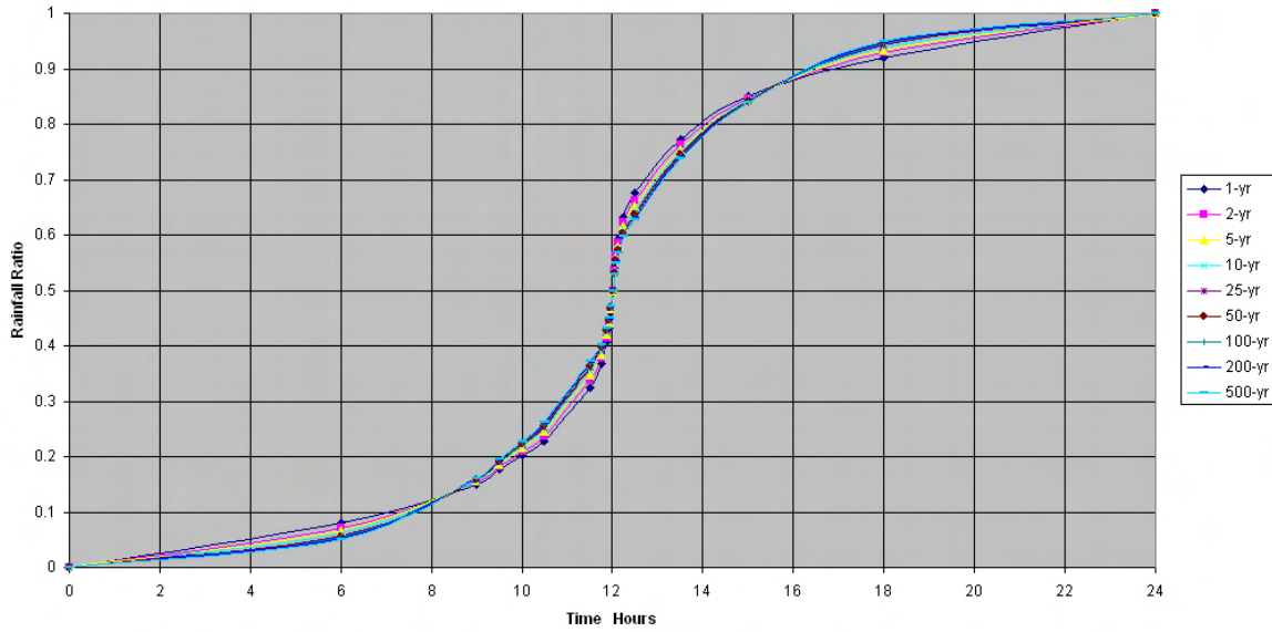
Figure 5-1M. Design rainfall distribution for 1-year to 500-year for Majuro (914460), Marshall Islands based on data from 1984-2005.
