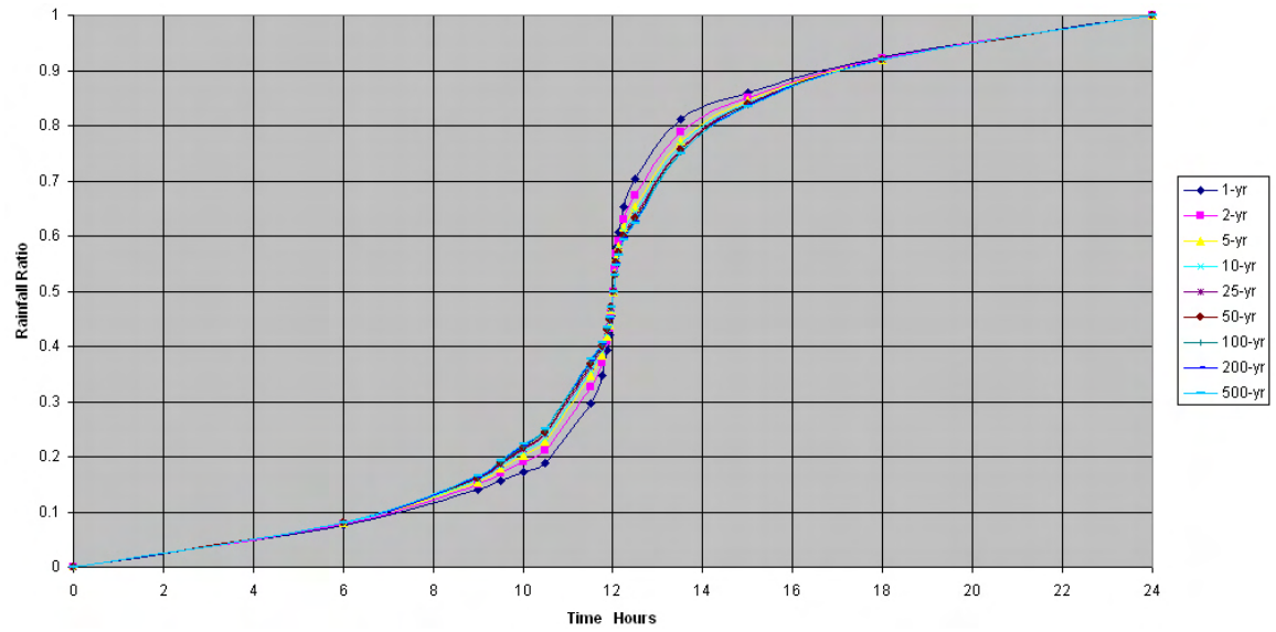
Figure 5-1P. Design rainfall distribution for 1-year to 500-year for Wake Island (914901).
