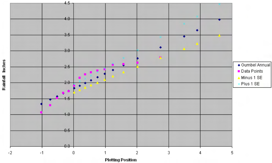
Figure 7-H1. Plot of 1-hour data points versus Gumbel analysis for Yap, FSM.
