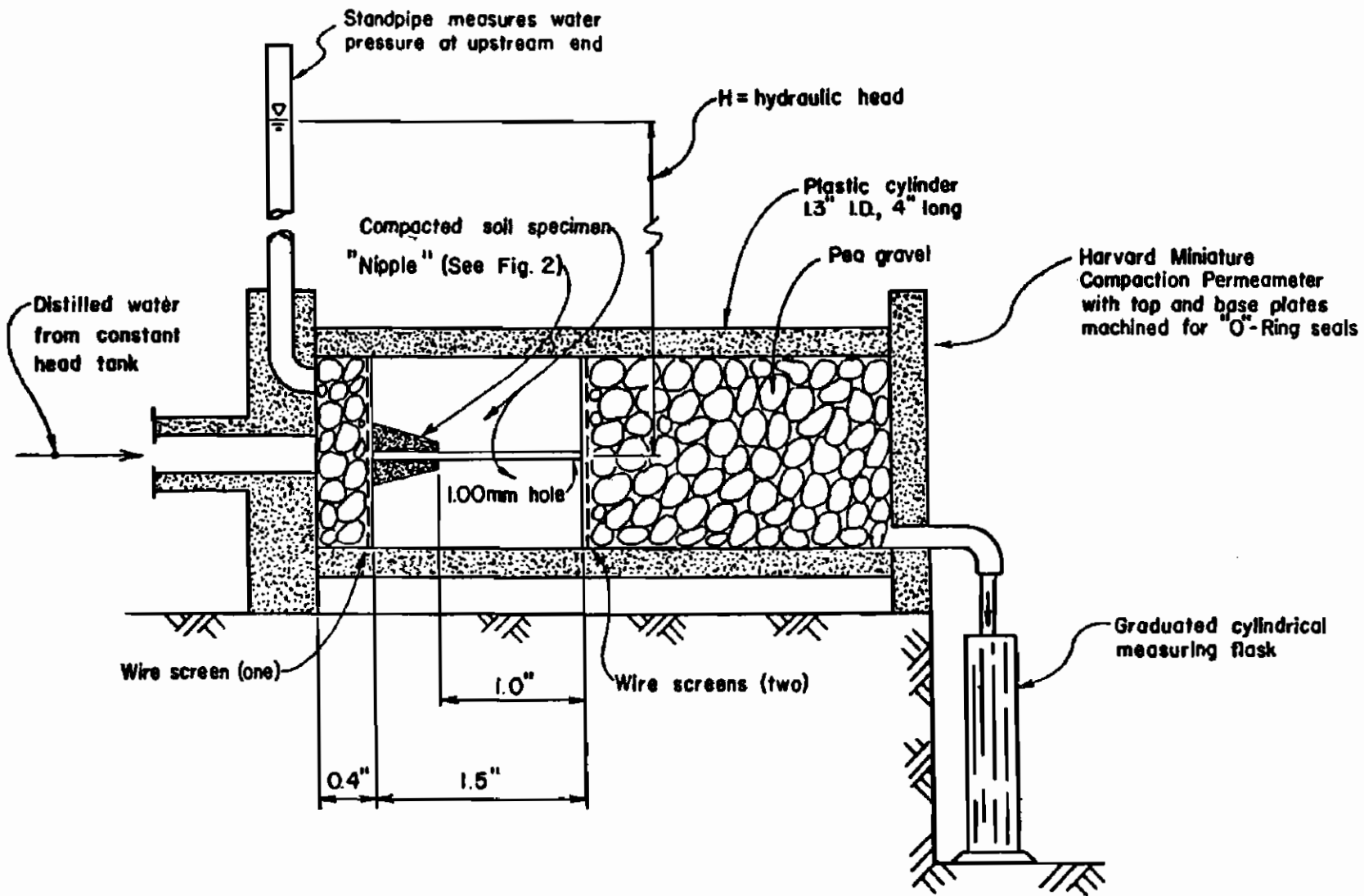
Figure 2 PINHOLE TEST APPARATUS (Schematic - Not to scale)
