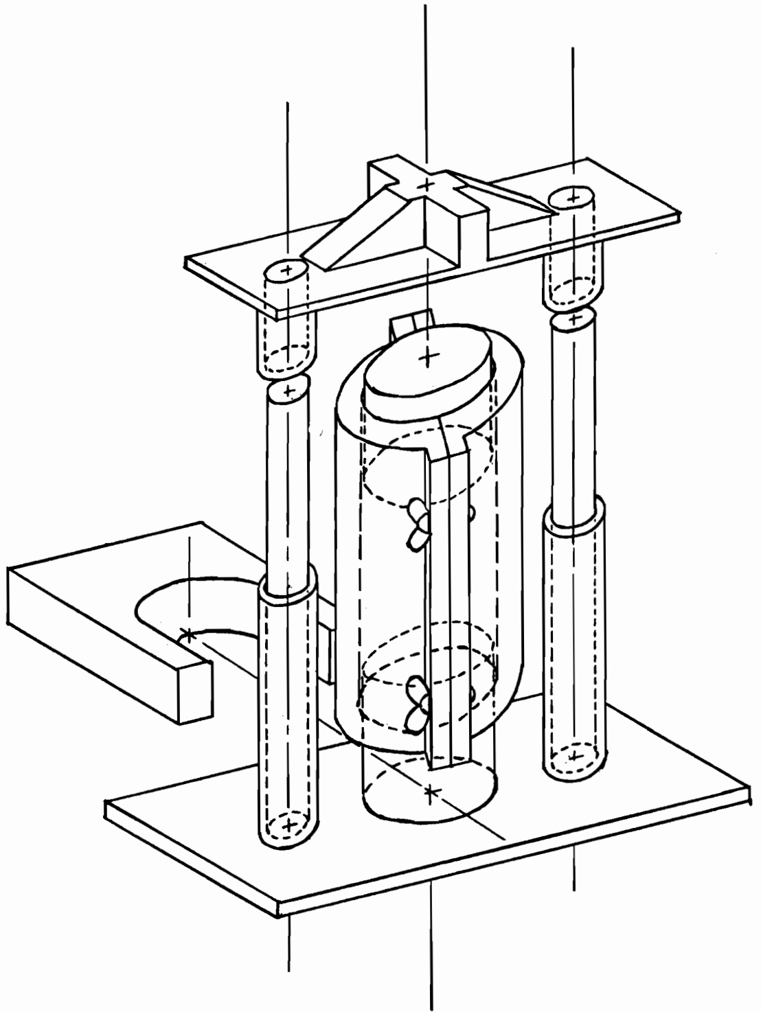
FIGURE 1. FLOATING MOLD COMPACTION DEVICE
