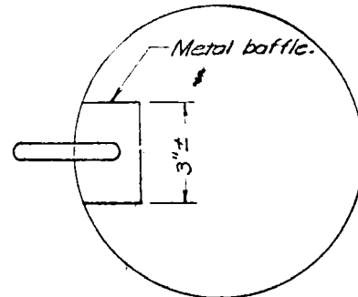
PLAN VIEW SHOWING BAFFLE
