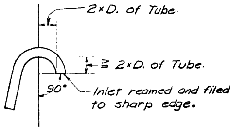
DETAIL OF TUBE ASSEMBLY (BAFFLE NOT SHOWN.)
