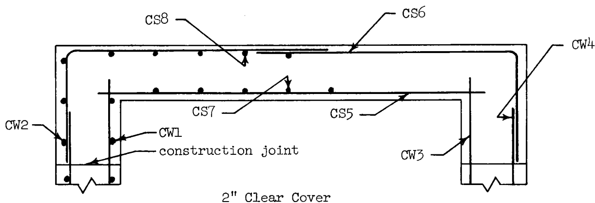
Figure 2-2. Cover slab and cover slab wall steel layout.
