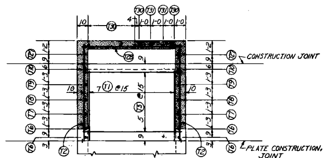
STEEL 2" FROM INSIDE FACE SECTION B-B
