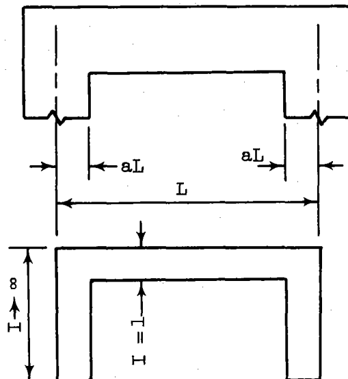
Figure 2-5. Assumed variation in moment of inertia.
