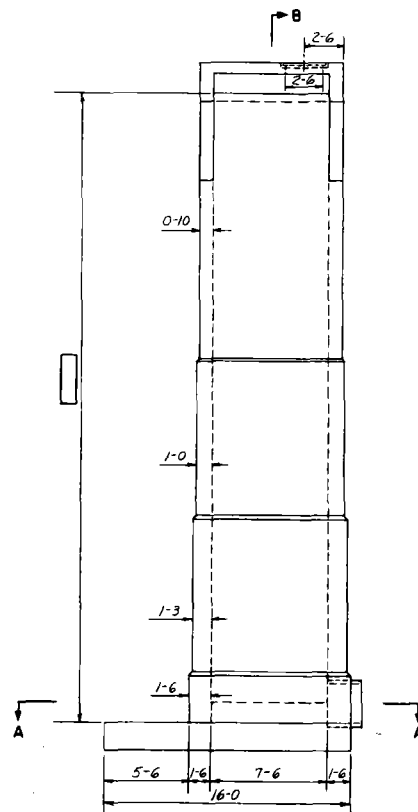
SIDEWALL ELEVATION
