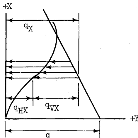
Figure 2-16. Typical load division curve.
