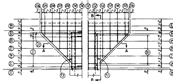
STEEL 2" FROM OUTSIDE FACE STEEL 2" FROM INSIDE FACE ENDWALL ELEVATION COVER SLAB STEEL NOT SHOWN
