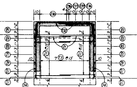
STEEL 2" FROM OUTSIDE FACE SECTION B-B
