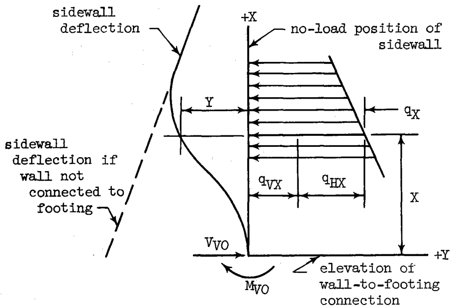
Figure 2-11. Vertical section through sidewall
