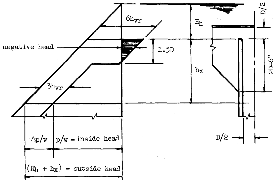
Figure 1-2. Representation of heads during pipe flow.
