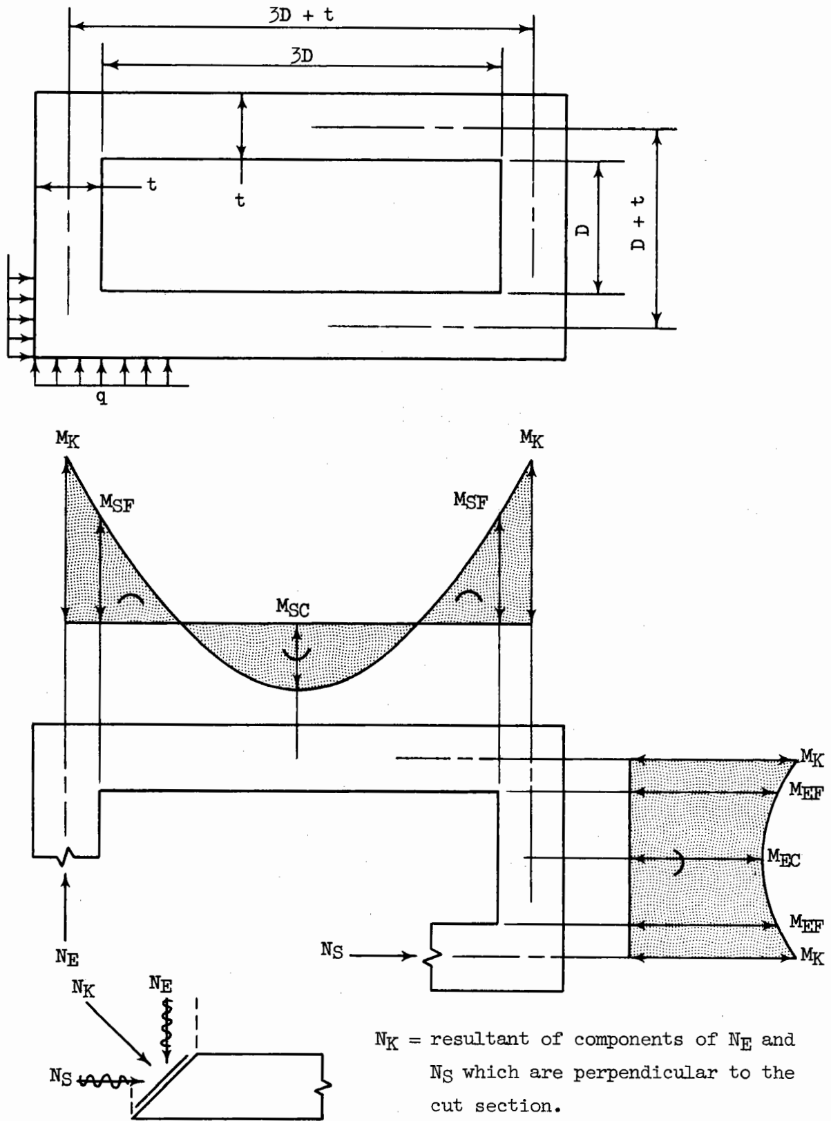
Figure 2-3. Definition sketch for horizontal bending.
