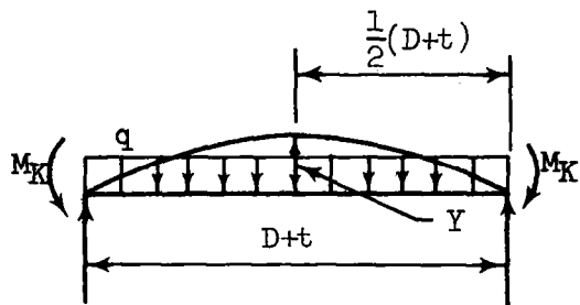
endwall deflections
