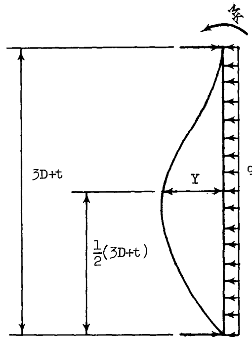
sidewall deflections
