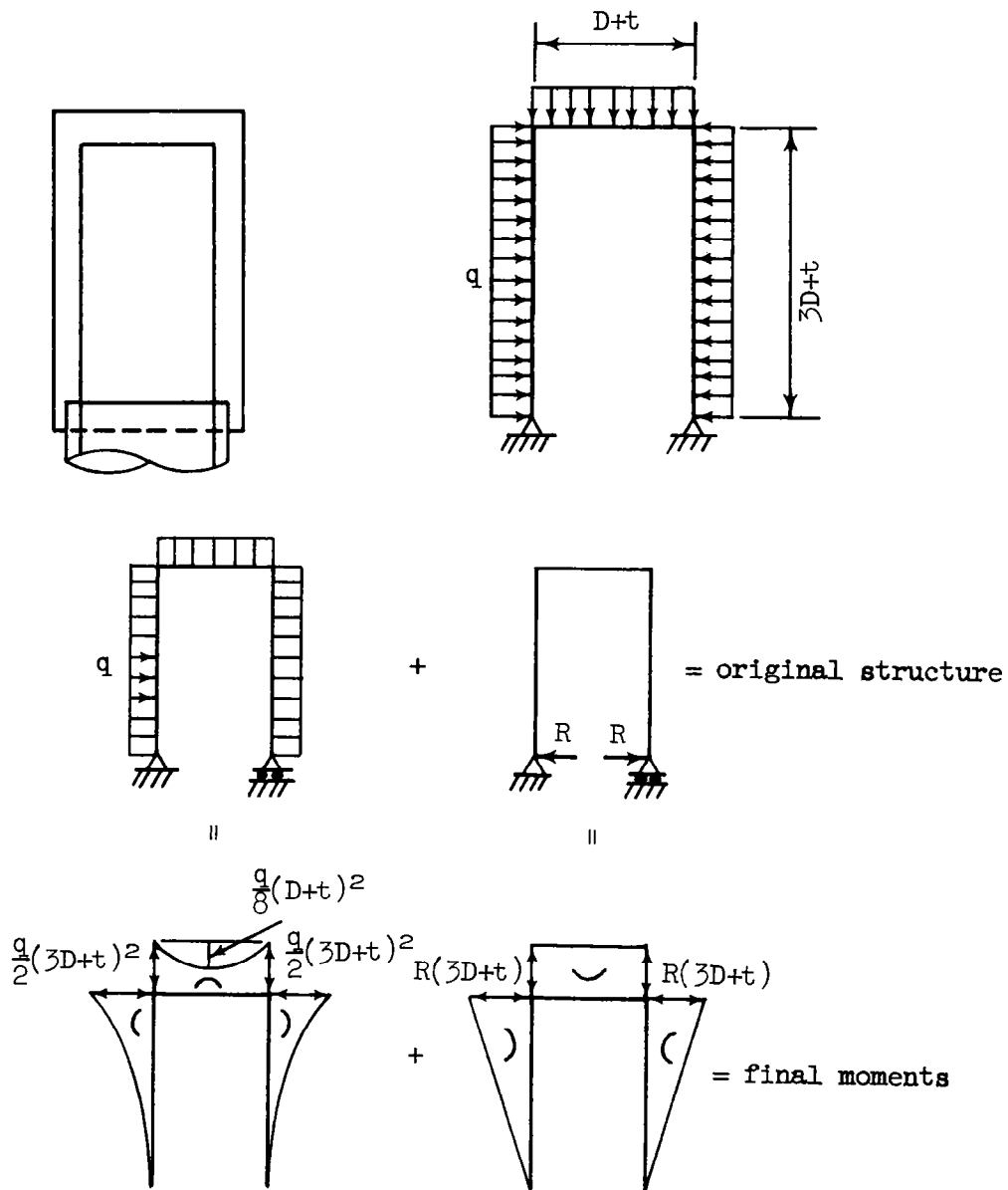
Figure 2-13. Sketches for analysis of pinned frame.
