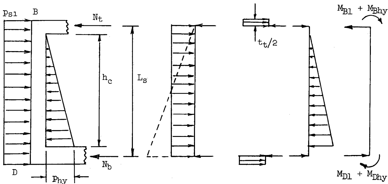
Figure 27. Components of direct force in top and bottom slabs with loading B2-IC#1
