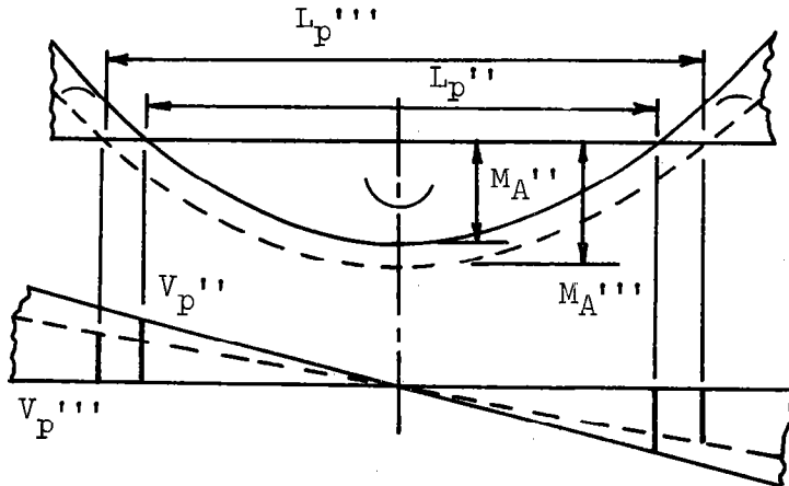
Figure 34. Points of inflection with loadings B2-IC#1 and B3-IC#1.
