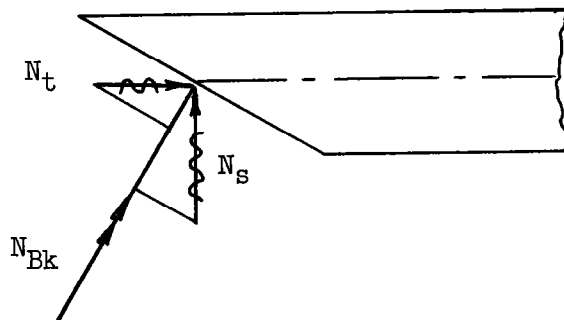
Figure 32. Resultants on top corner diagonal.
