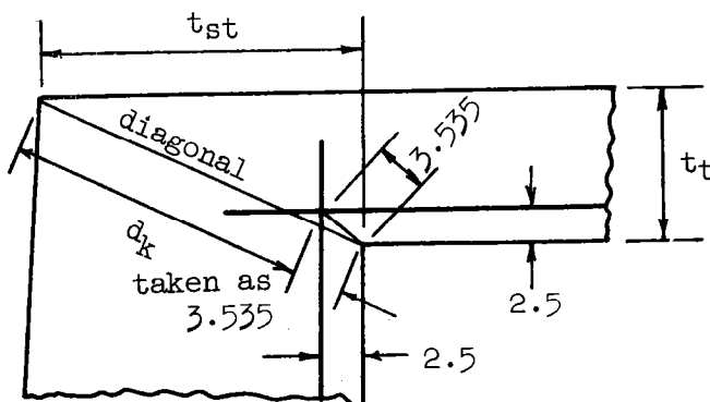
Figure 31. Top corner geometry.
