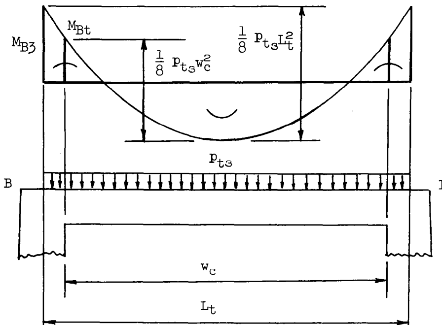
Figure 23. Moments in top slab with loading Bl-LC#3.
