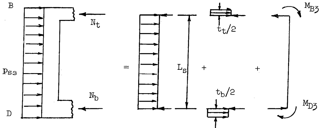
Figure 24. Components of direct force in top and bottom slabs with loading Bl-IC#3.
