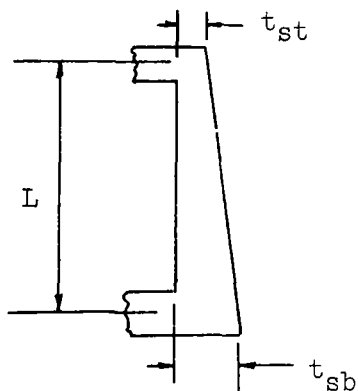
Figure 7. Sidewall batter.
