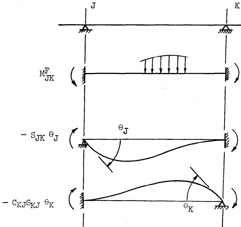
Figure 8. Development of Slope Deflection Equation.
