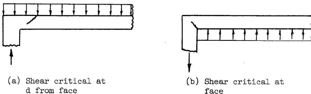
Figure 10. Location of critical shear.
