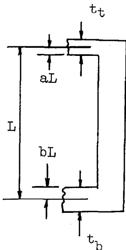
Figure 6. Unequal slab thicknesses.
