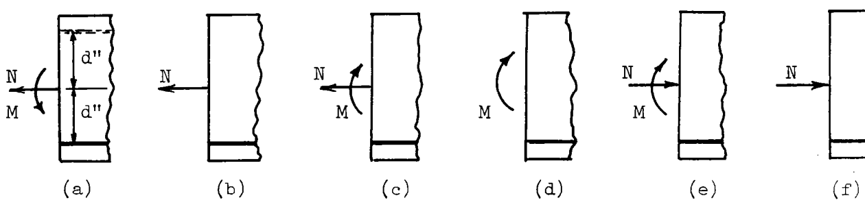
Figure 30. Existence of tension in bottom steel.
