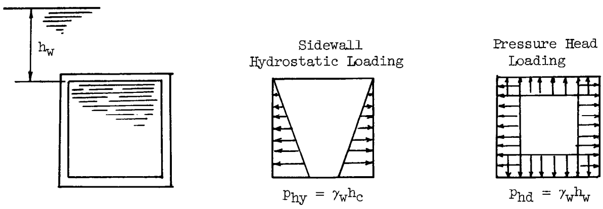
Figure 3. Treatment of internal water loads.
