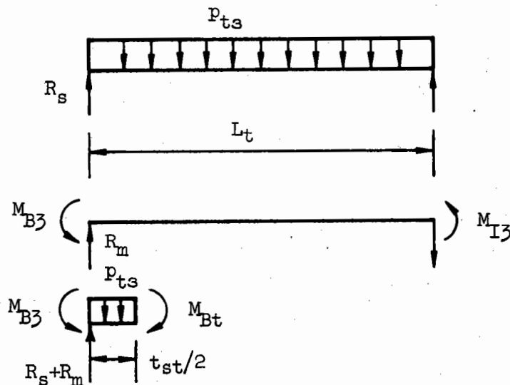
Figure 2-14. Negative bending in top slab with loading Bl-IC#3
