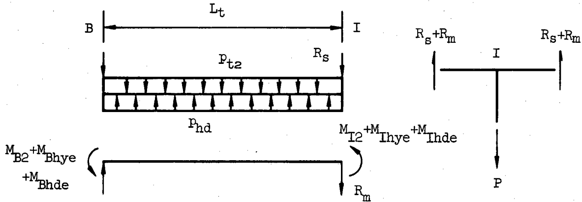
Figure 2-15. Centerwall tension for loading B3-LC#2
