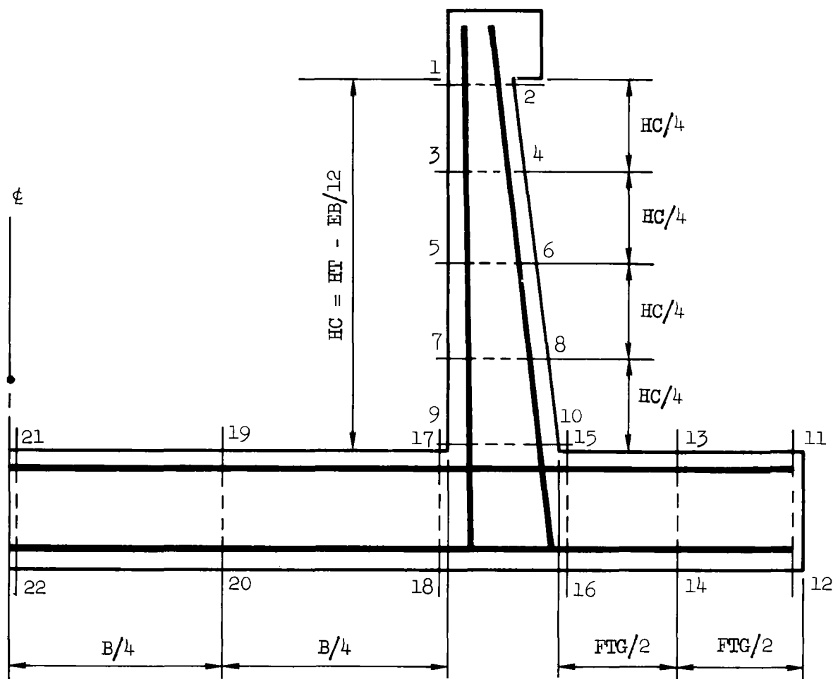
Figure 39. Type T1S steel layout and point locations.
