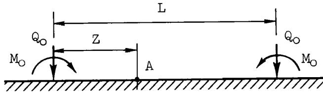
Figure 27. Q_0 and M_0 loadings, infinite beam.
