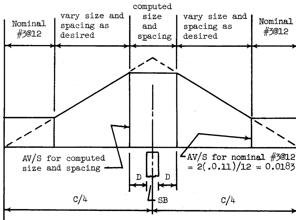
Figure 42. Layout of edge beam stirrups.
