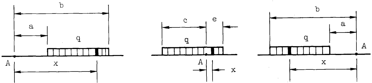
Figure 26. Uniform loading cases, infinite beams.
