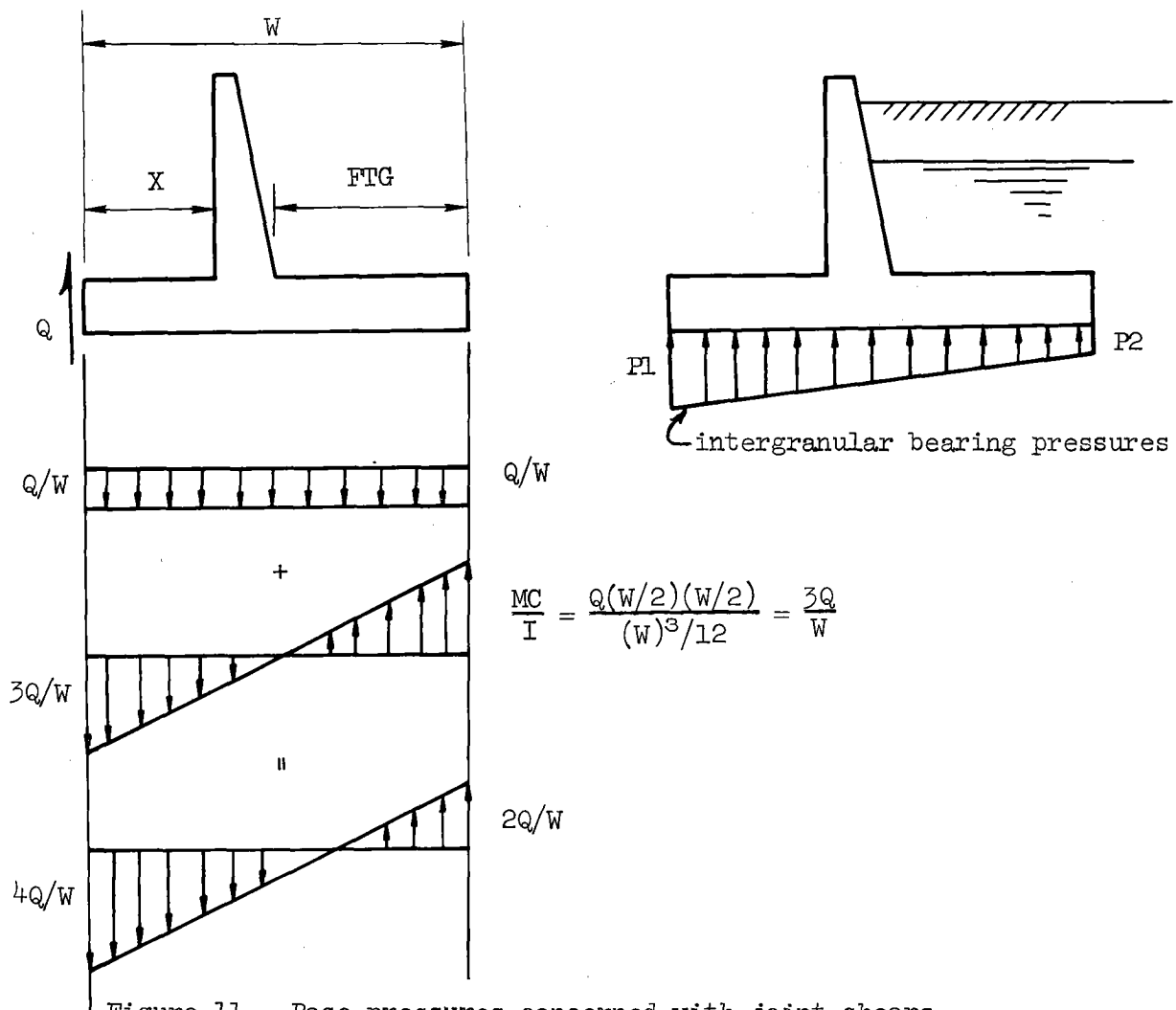
Figure 11. Base pressures concerned with joint shears.
