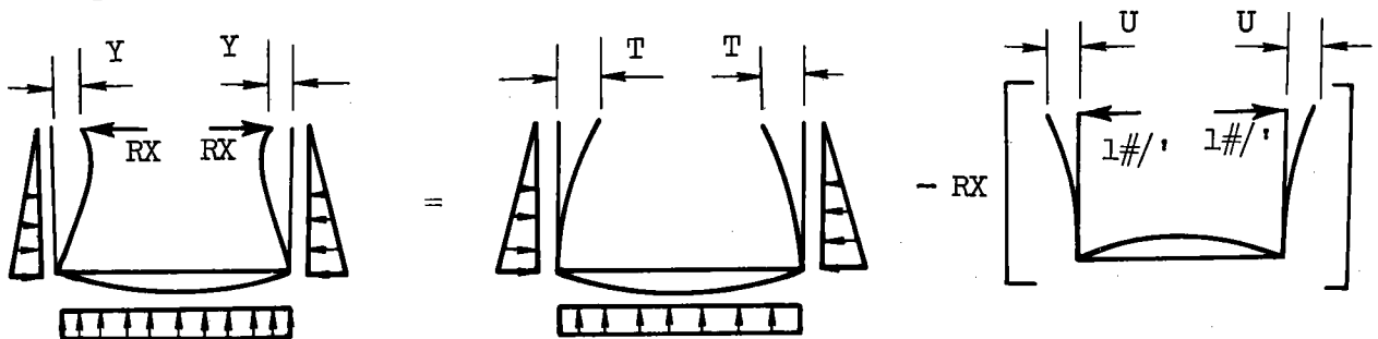
Figure 16. Type TLS frame displacements, typical loading.
