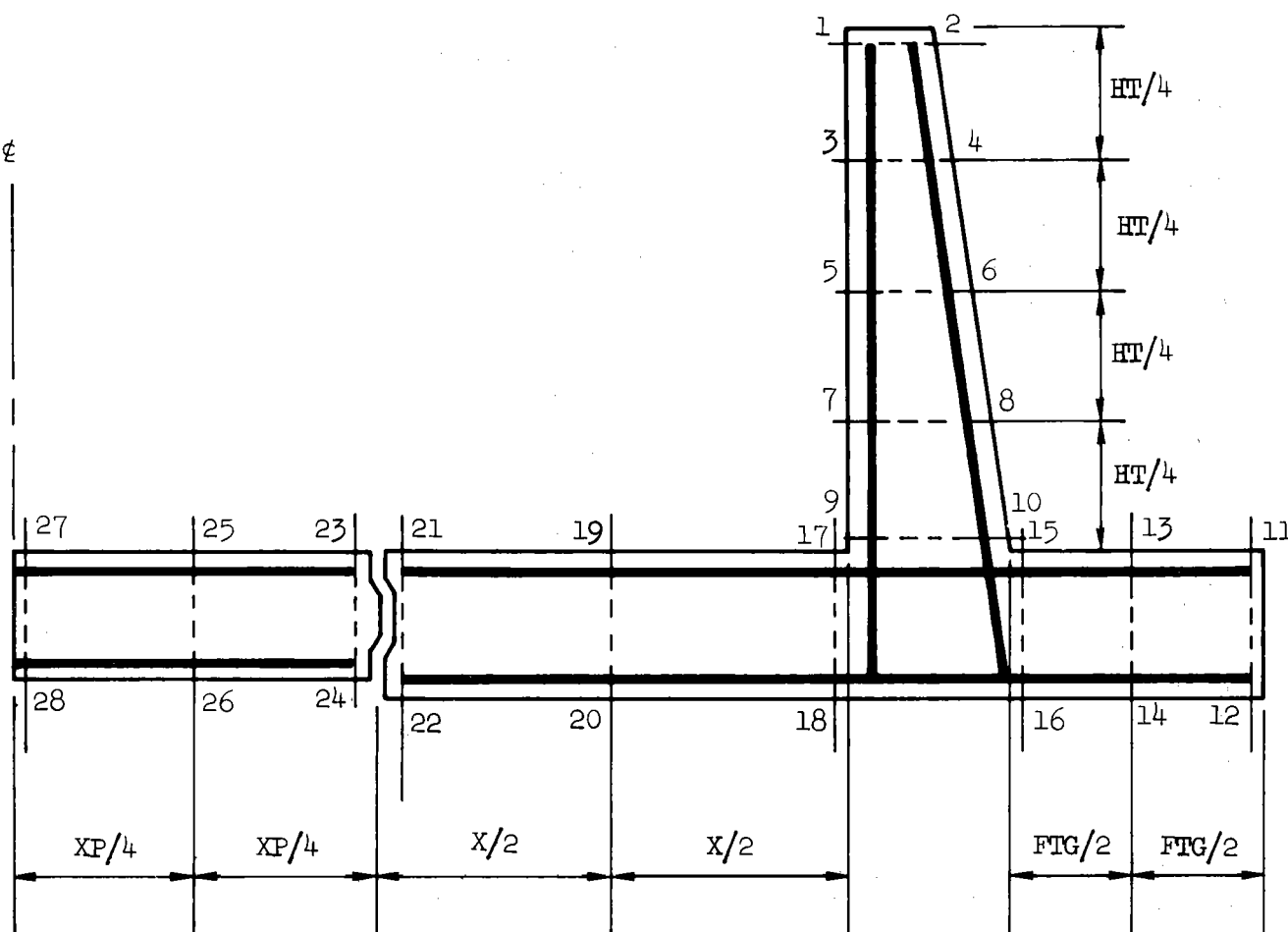
Figure 36. Type T3FV steel layout and point locations.
