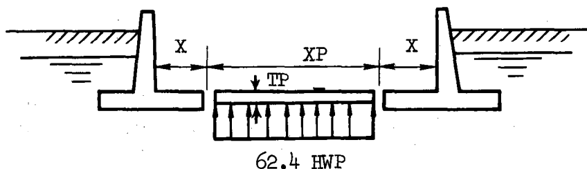
Figure 9. Pavement slab flotation, type T3F.
