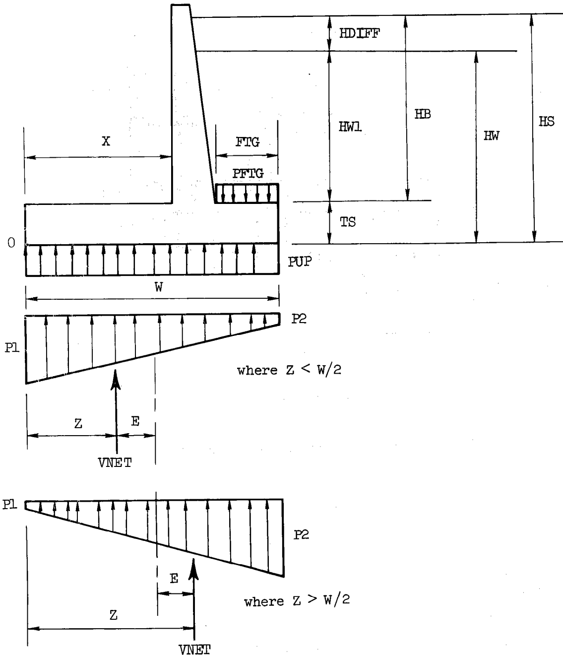
Figure 7. Bearing pressures, IC#1 when H_B > H_{WL} .
