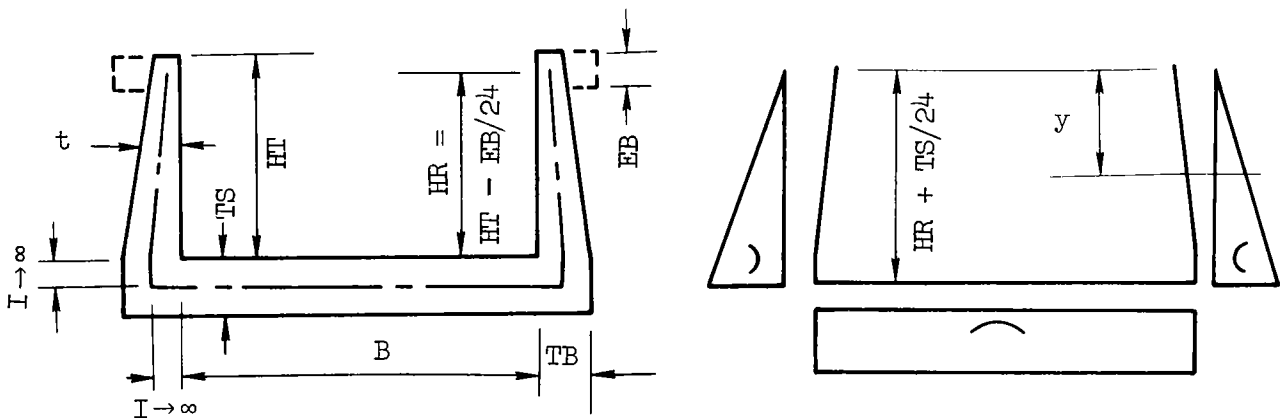
Figure 18. Evaluation of frame U and n.
