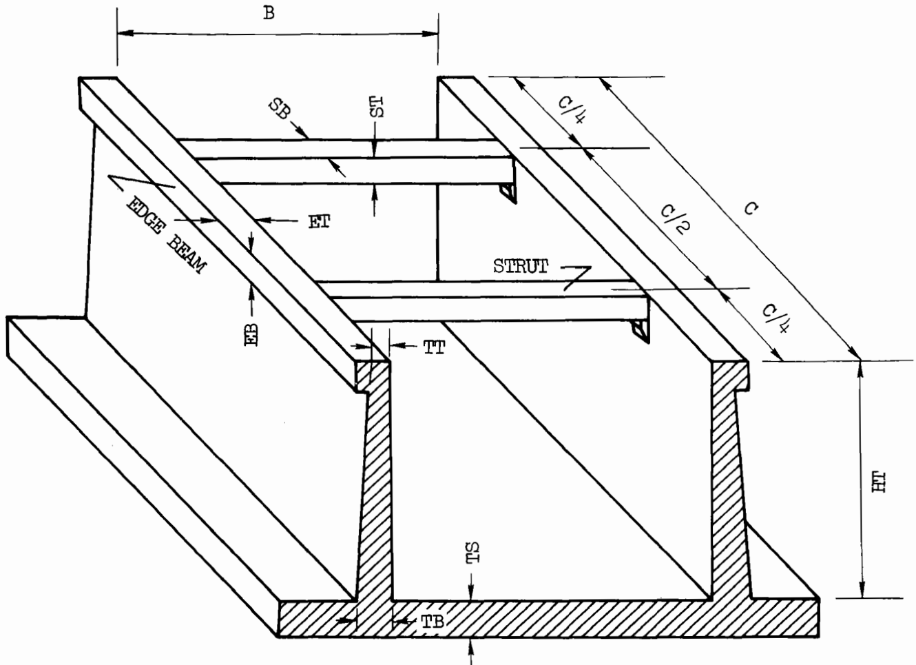
Figure 13. Definition sketch, type TLS channel.
