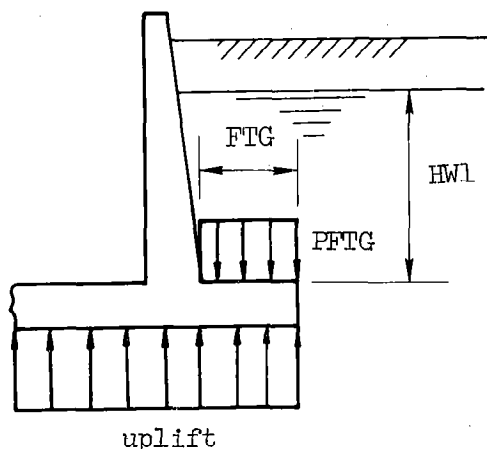
Figure 4. Flotation conditions.
