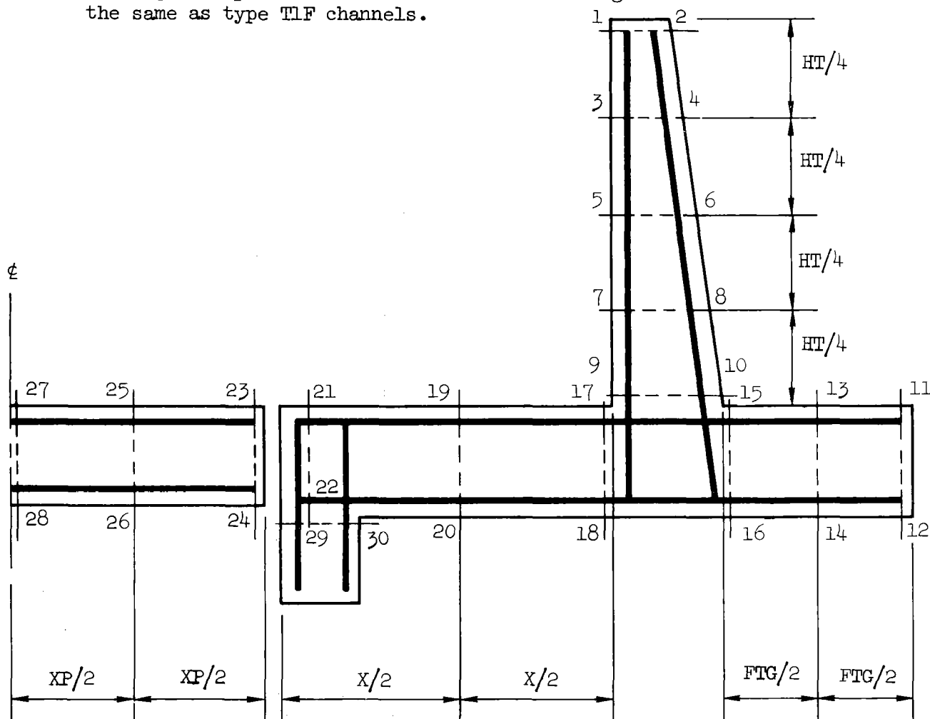
Figure 33. Type T3F steel layout and point locations.
