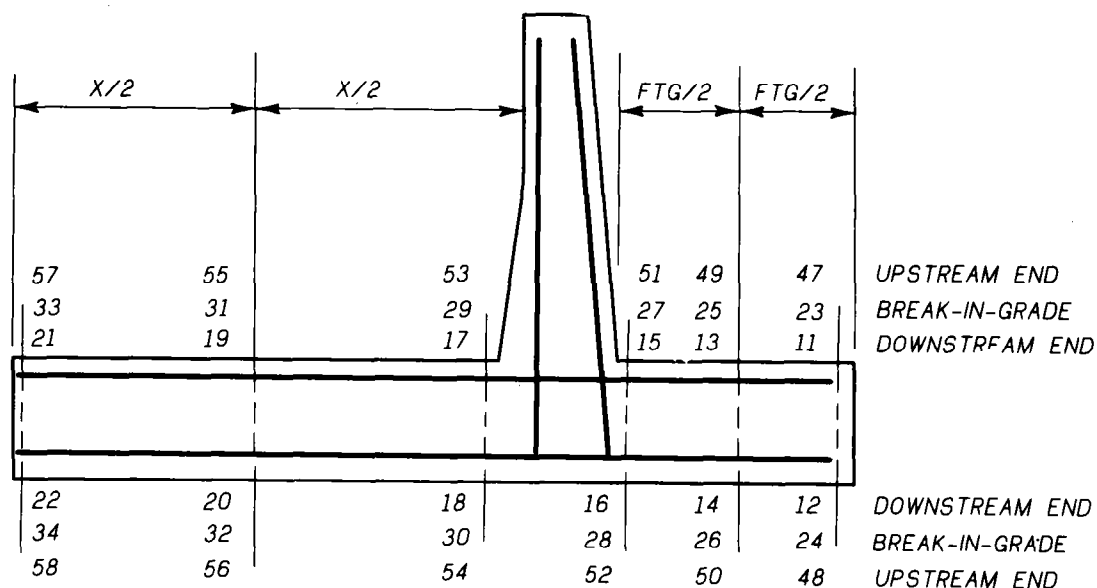
Figure 45. Base slab steel layout and point locations
