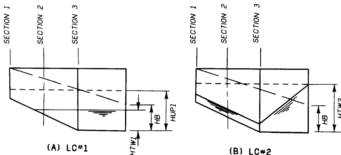
Figure 23. Considerations for sidewall bending, Type (B) basin
