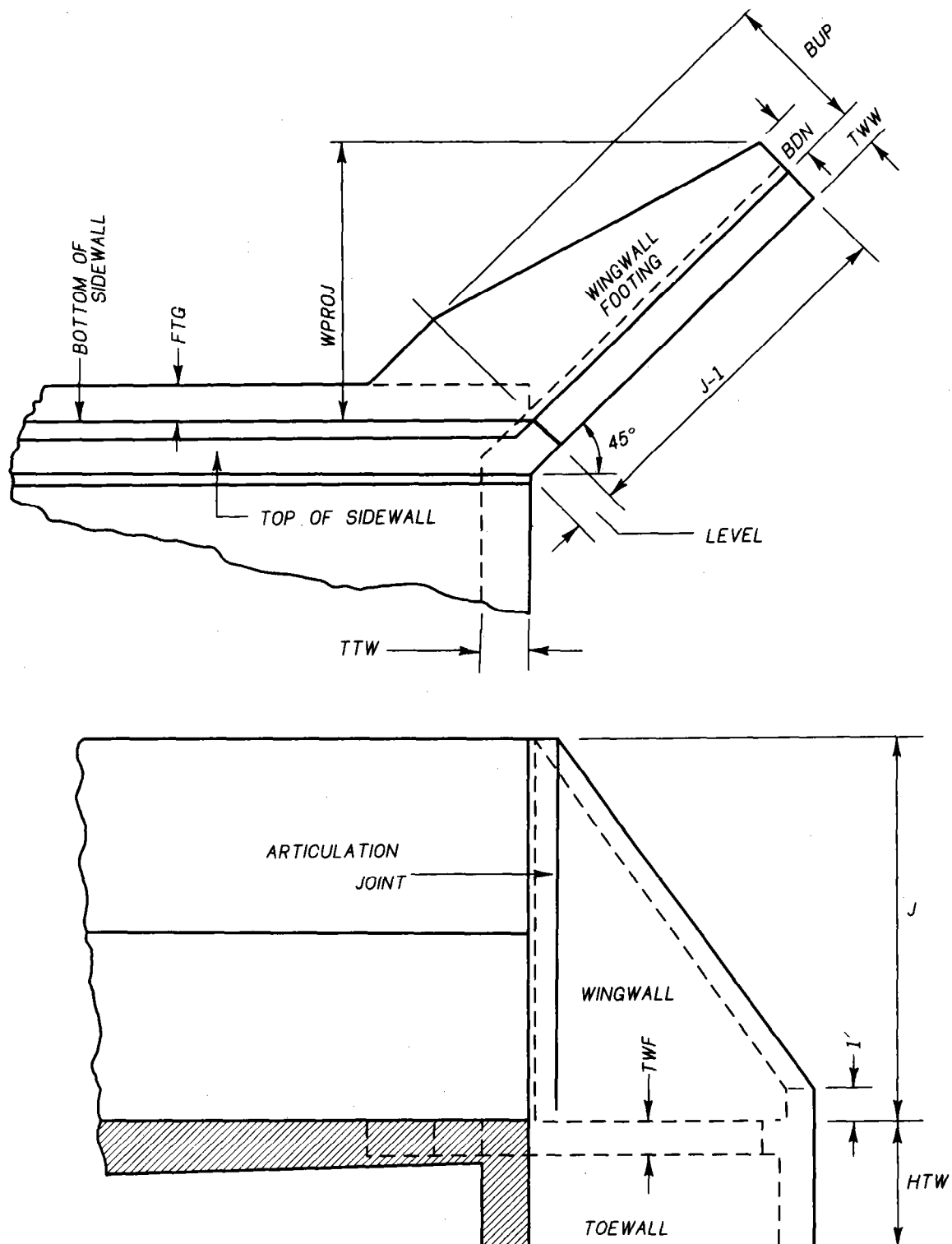
Figure 4. Wingwall layout
