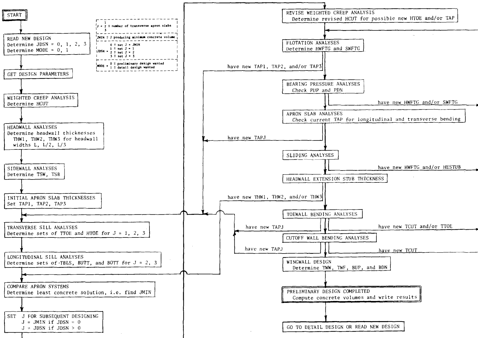
Figure 5. Simplified flow chart for preliminary design.
