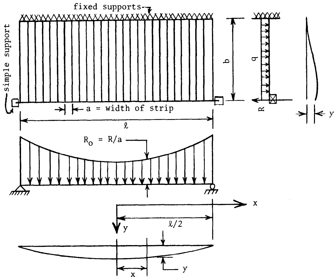
Figure 19. Transverse sill analysis - no longitudinal sills.
