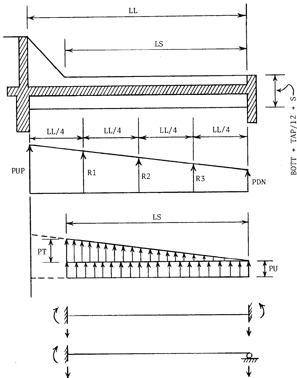
Figure 42. Longitudinal sill design.
