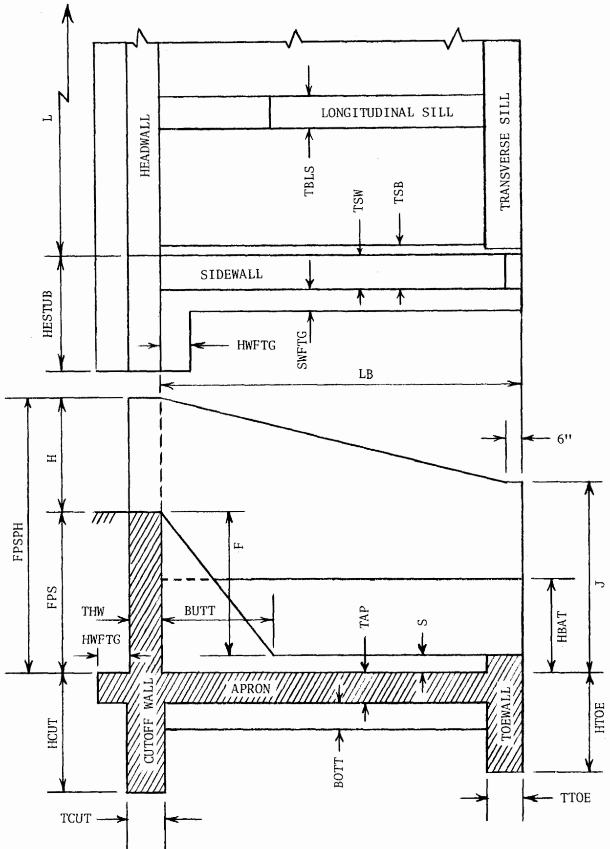
Figure 1. Straight drop spillway definition sketch.
