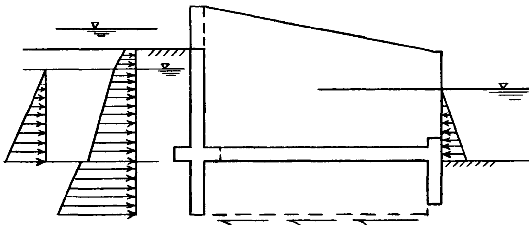
Figure 27. Sketch for sliding analyses.
