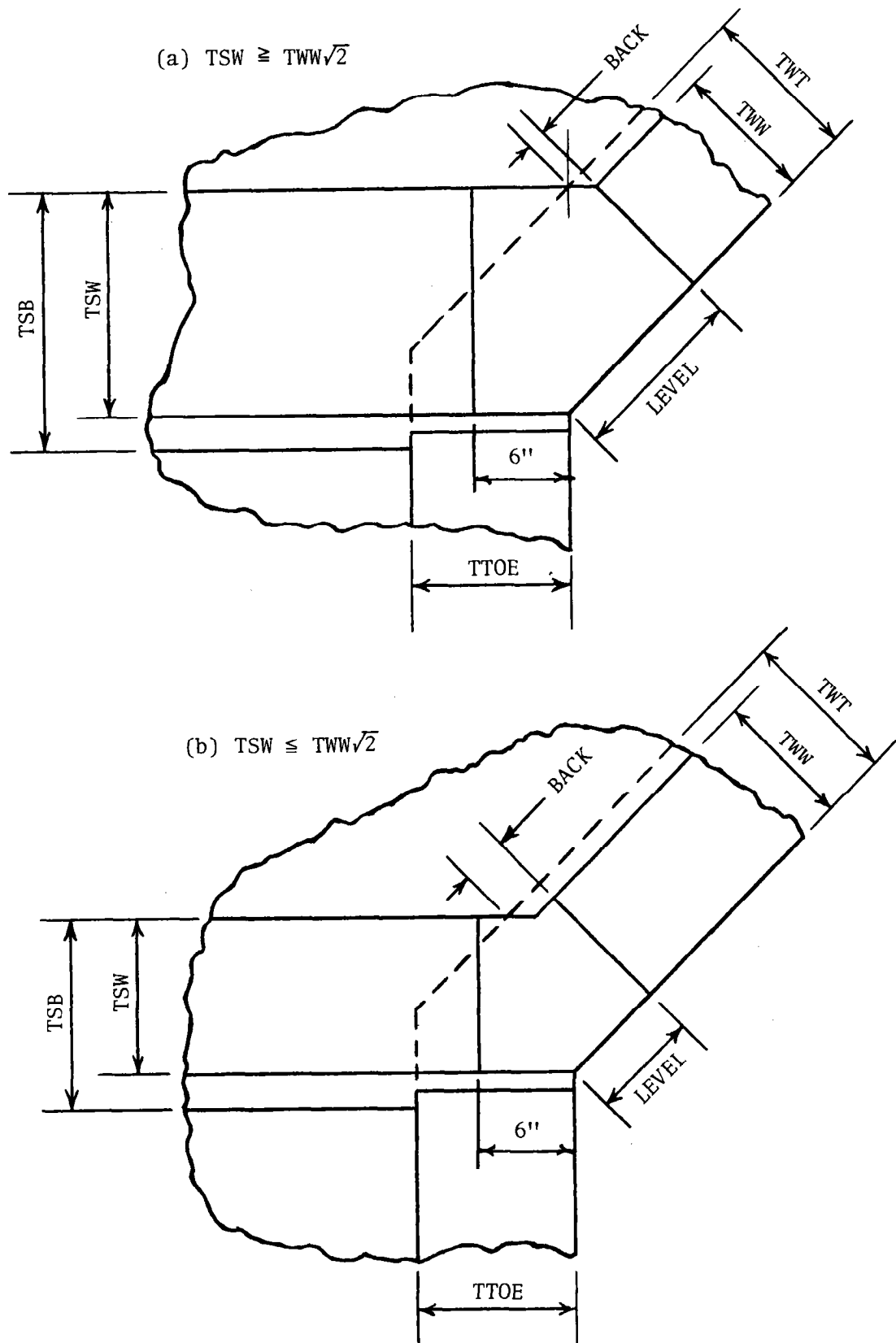
Figure 48. Corner detail, wingwall-to-sidewall.
