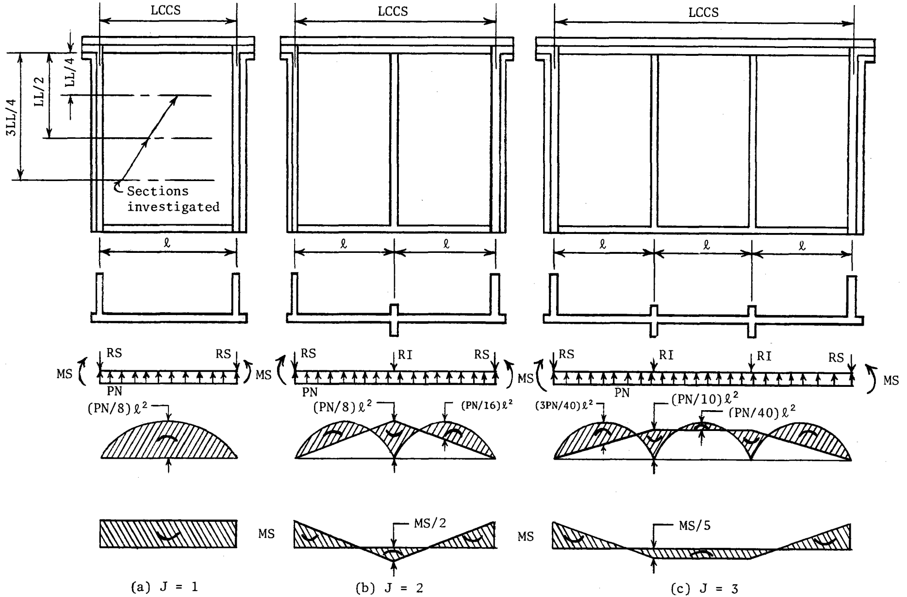
Figure 26. Transverse bending of the apron slab.
