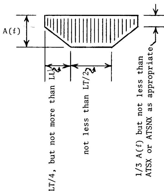
Transverse envelope of longitudinal steel except A(32) and A(39)
