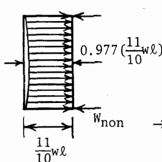
(b) longitudinal sill loading, if transverse sill were non-yielding
