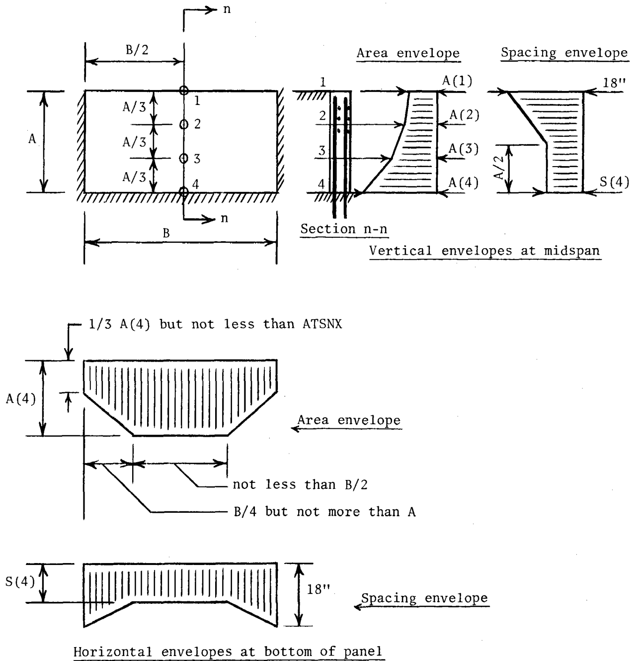
Figure 33. Vertical steel in headwall panel.
