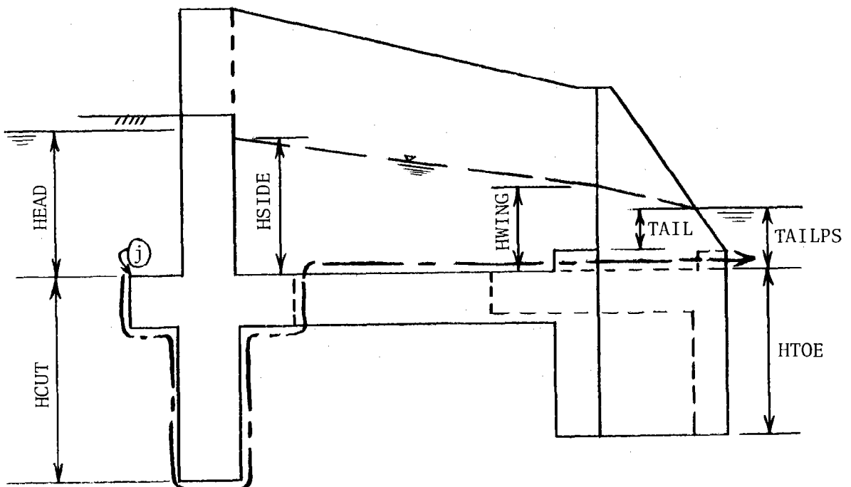
Figure 10. Sidewall water heads for given loading.
