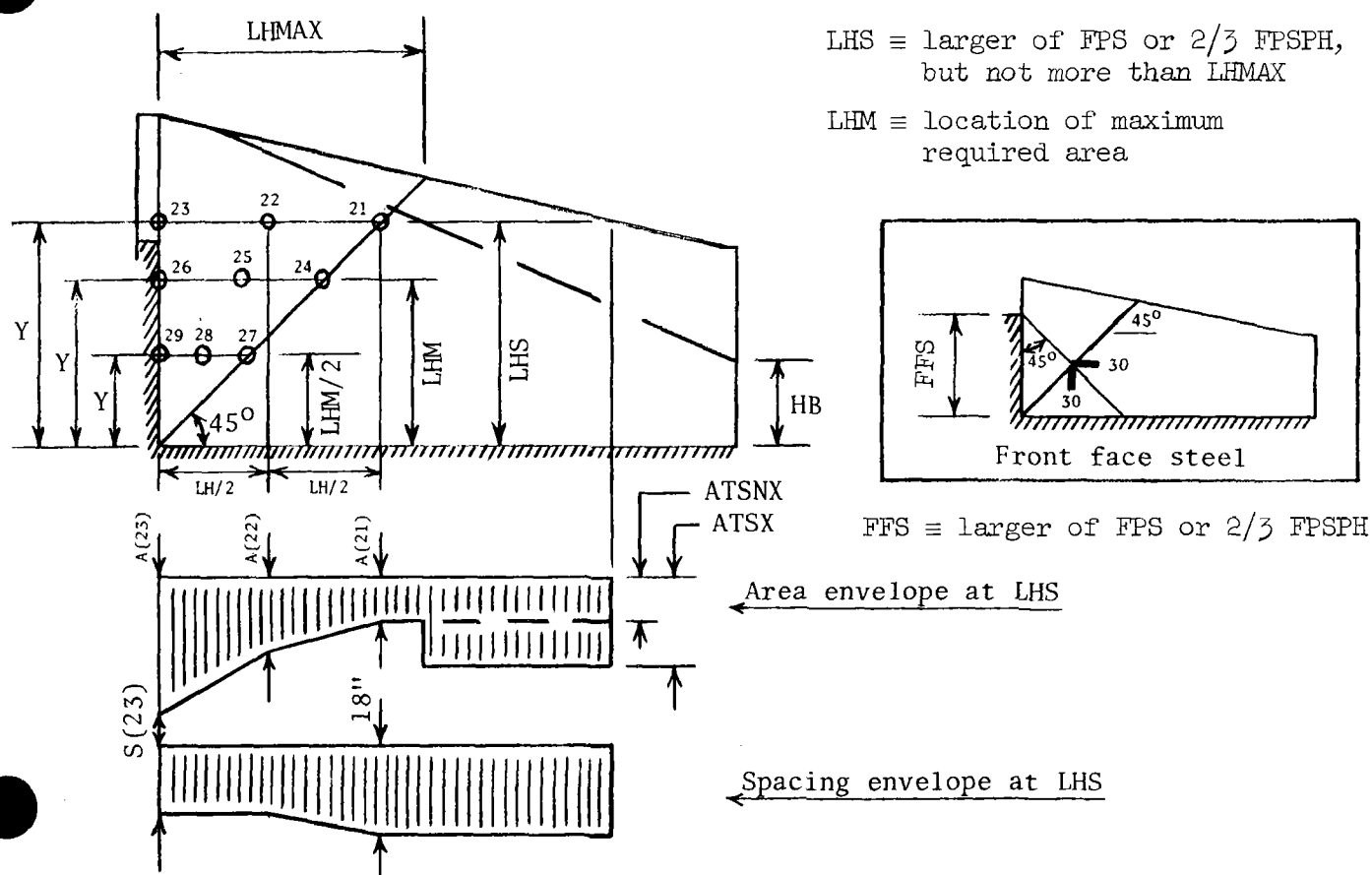
Figure 36. Horizontal steel in sidewall.
