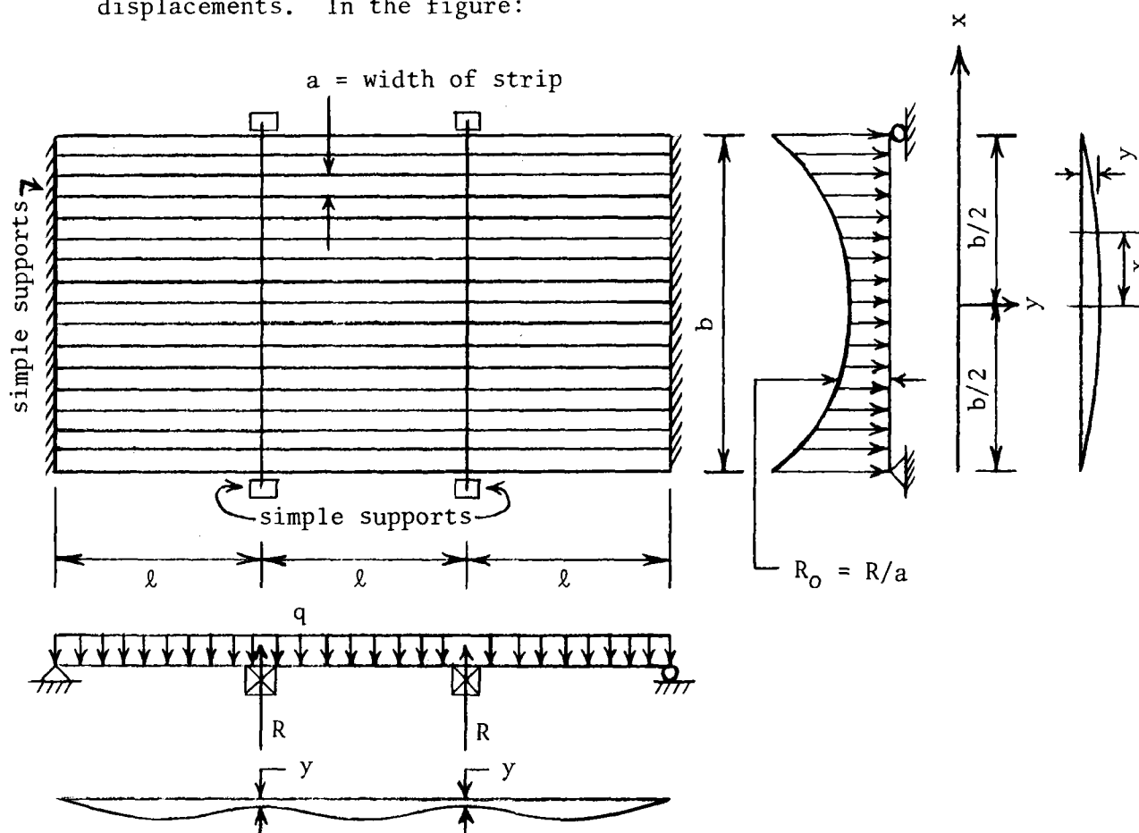
Figure 15. Longitudinal sill analysis - two sills.
