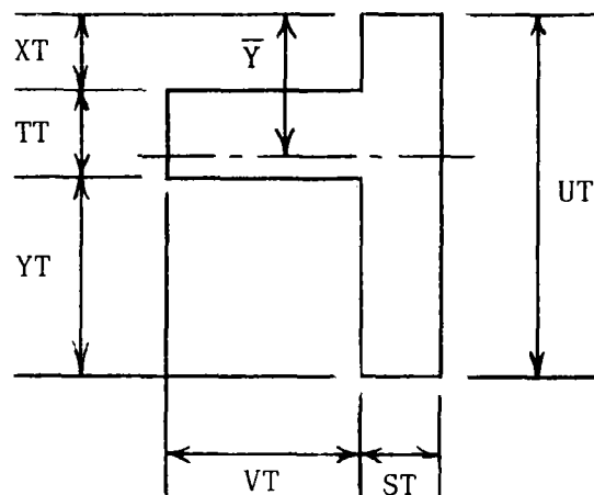
Figure 22. Transverse sill cross section.
