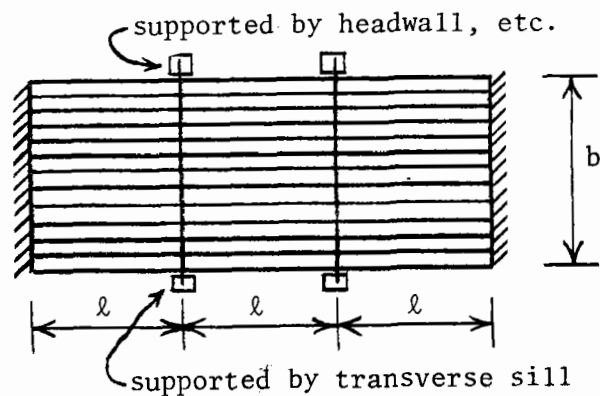
(a) plan of apron and sills
