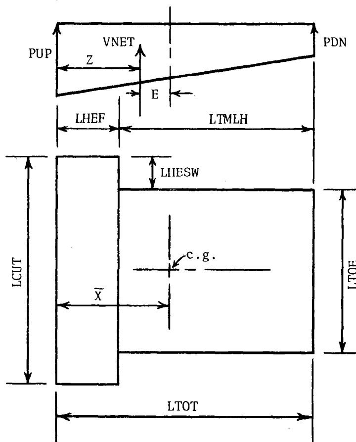
Figure 24. Determination of bearing pressures.
