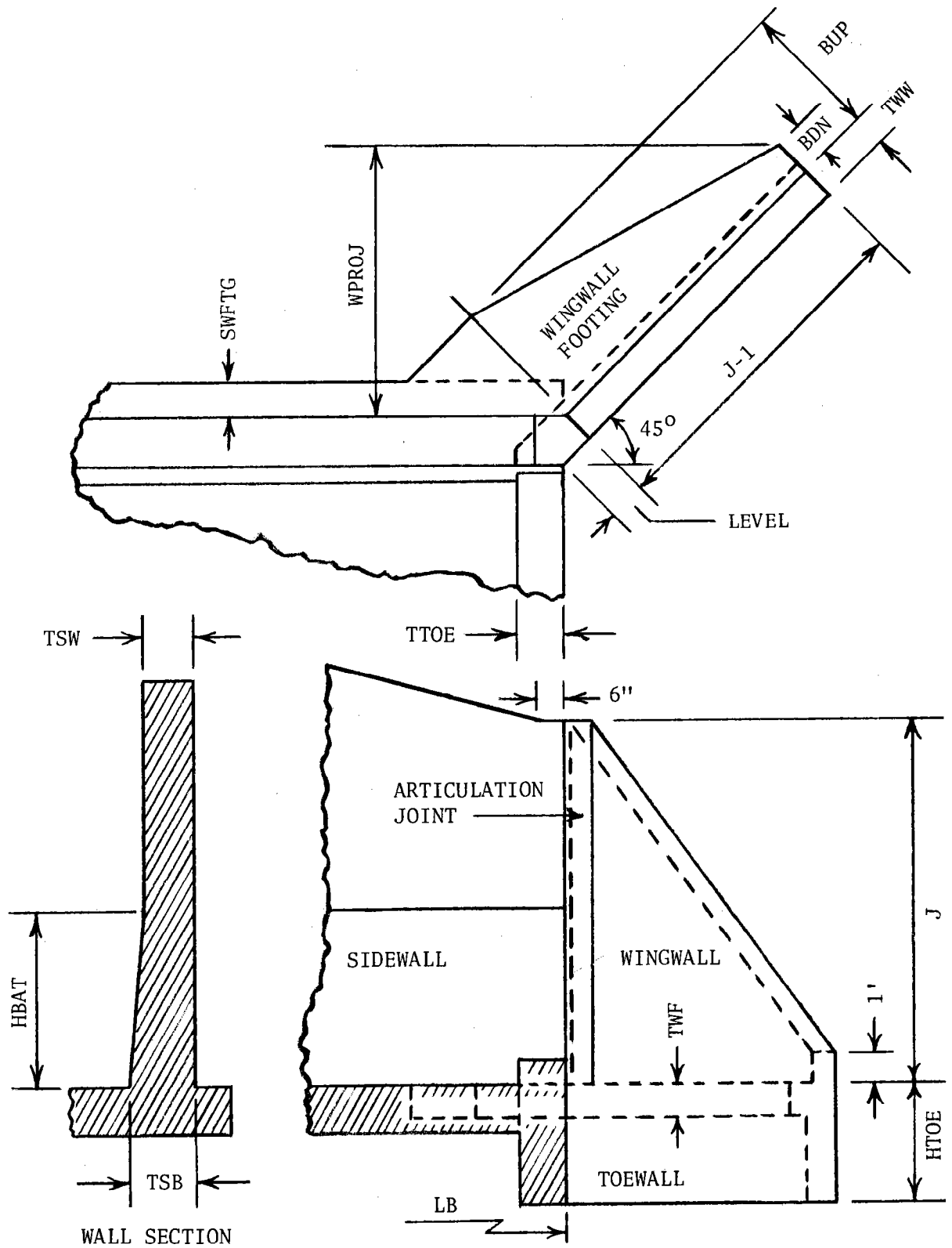
Figure 2. Wingwall layout.
