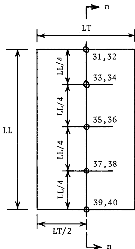
Apron panel
