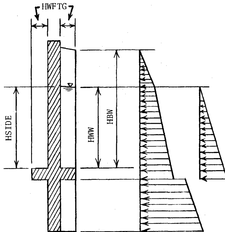
Figure 28. Section through headwall extension stub.
