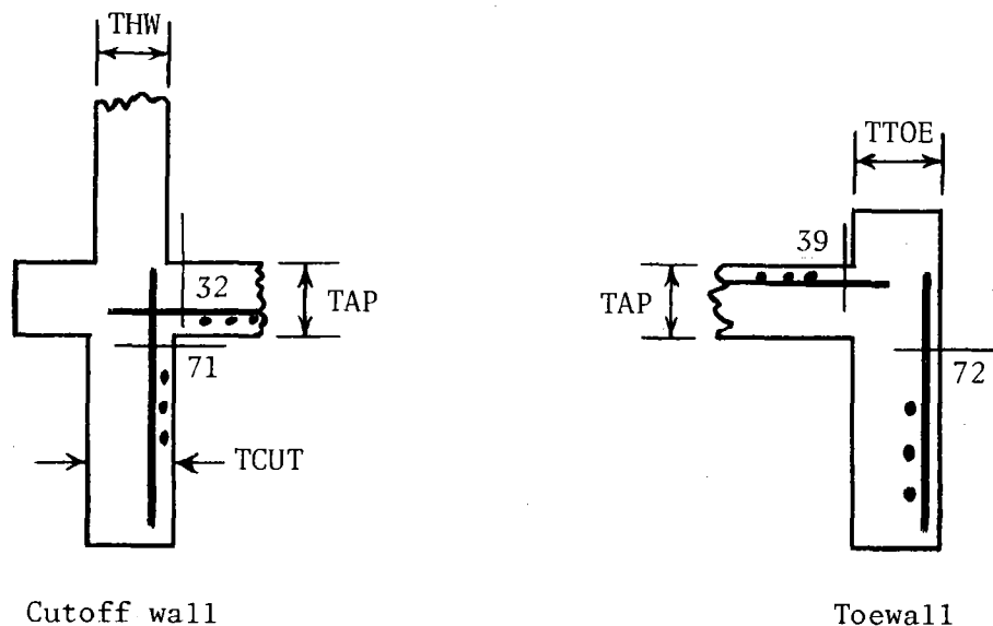
Figure 46. Cutoff wall and toewall steels.
