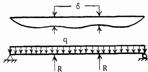
(e) displacement curve of strip adjacent to transverse sill
