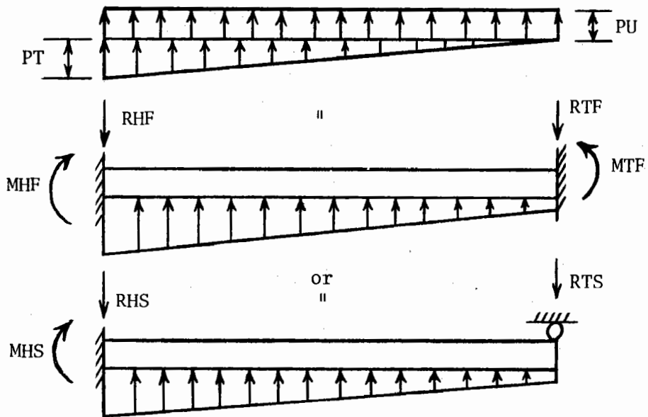
Figure 25. Longitudinal apron span loadings.
