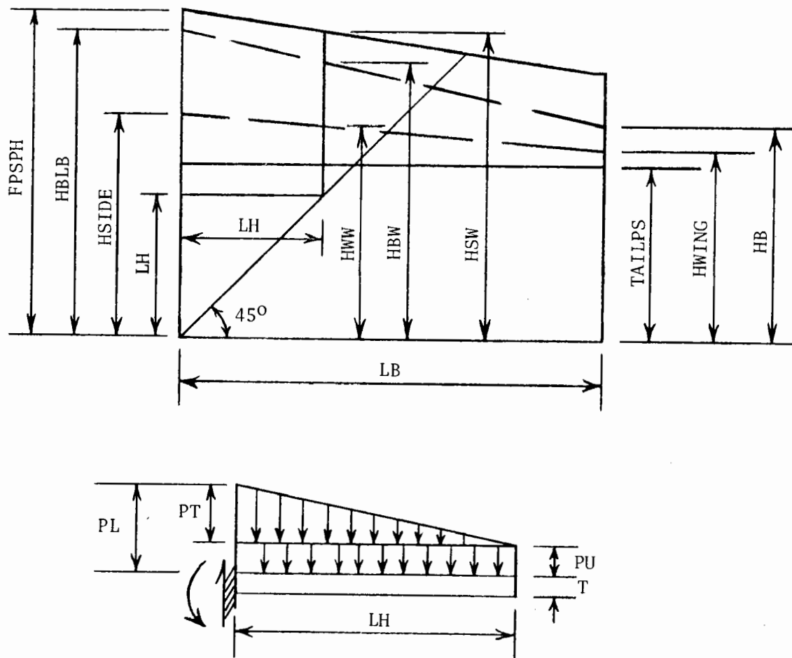
Figure 14. Horizontal bending of the sidewall.
