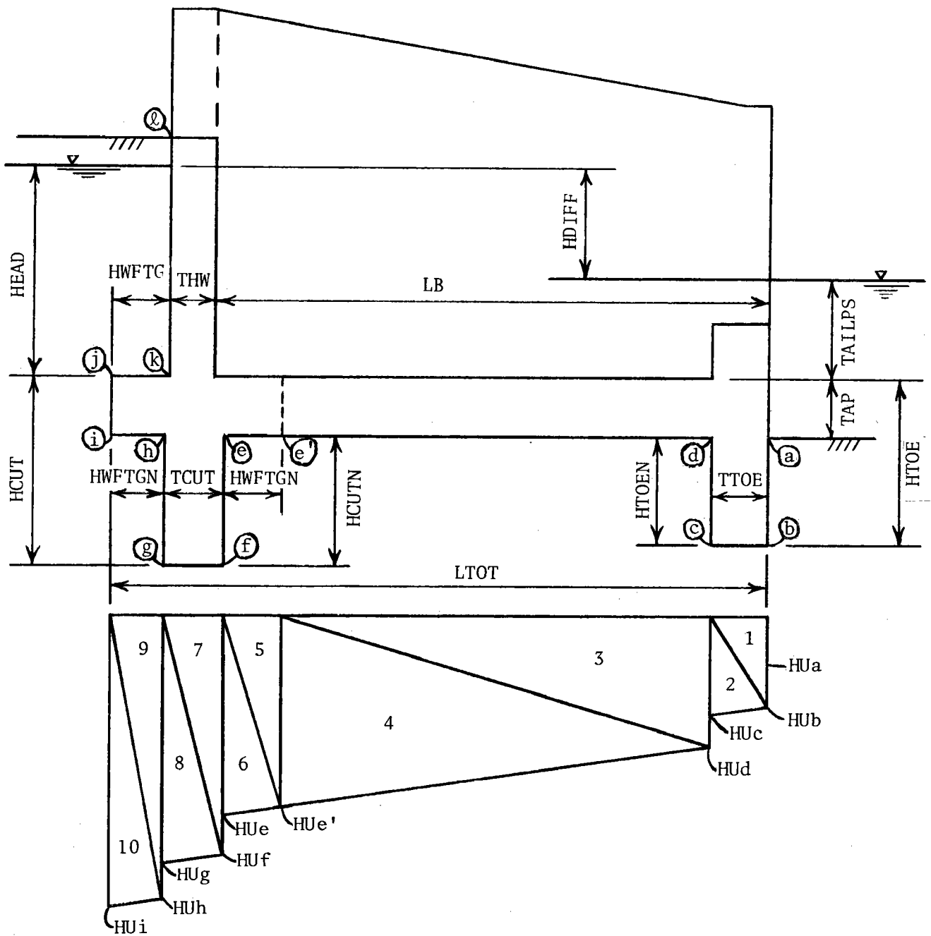
Figure 23. Drop spillway uplift diagram.
