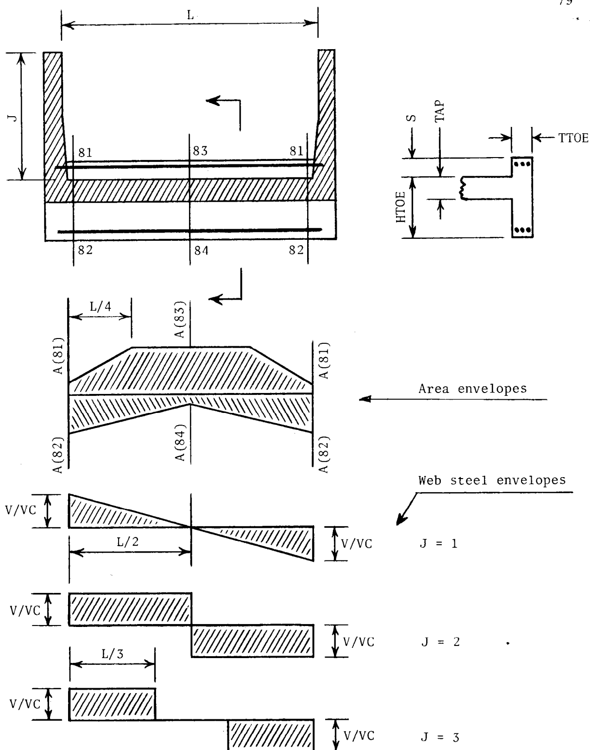
Figure 45. Transverse sill steel.
