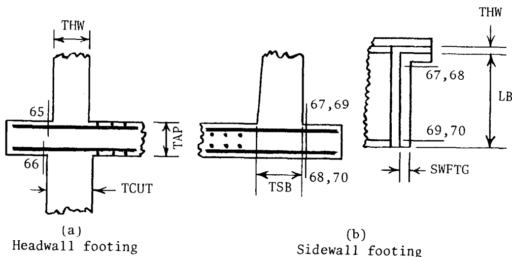
Figure 40. Headwall and sidewall footing steel.
