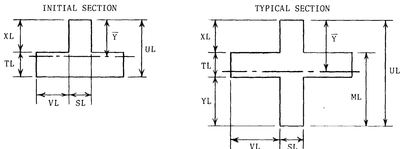
Figure 17. Longitudinal sill cross sections.
