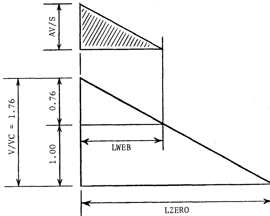
Figure 44. Region of required web steel.
