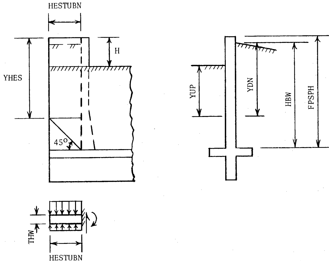
Figure 29. Headwall extension stub analysis.
