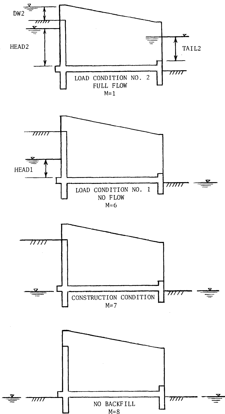
Figure 4. Loading cases considered.
