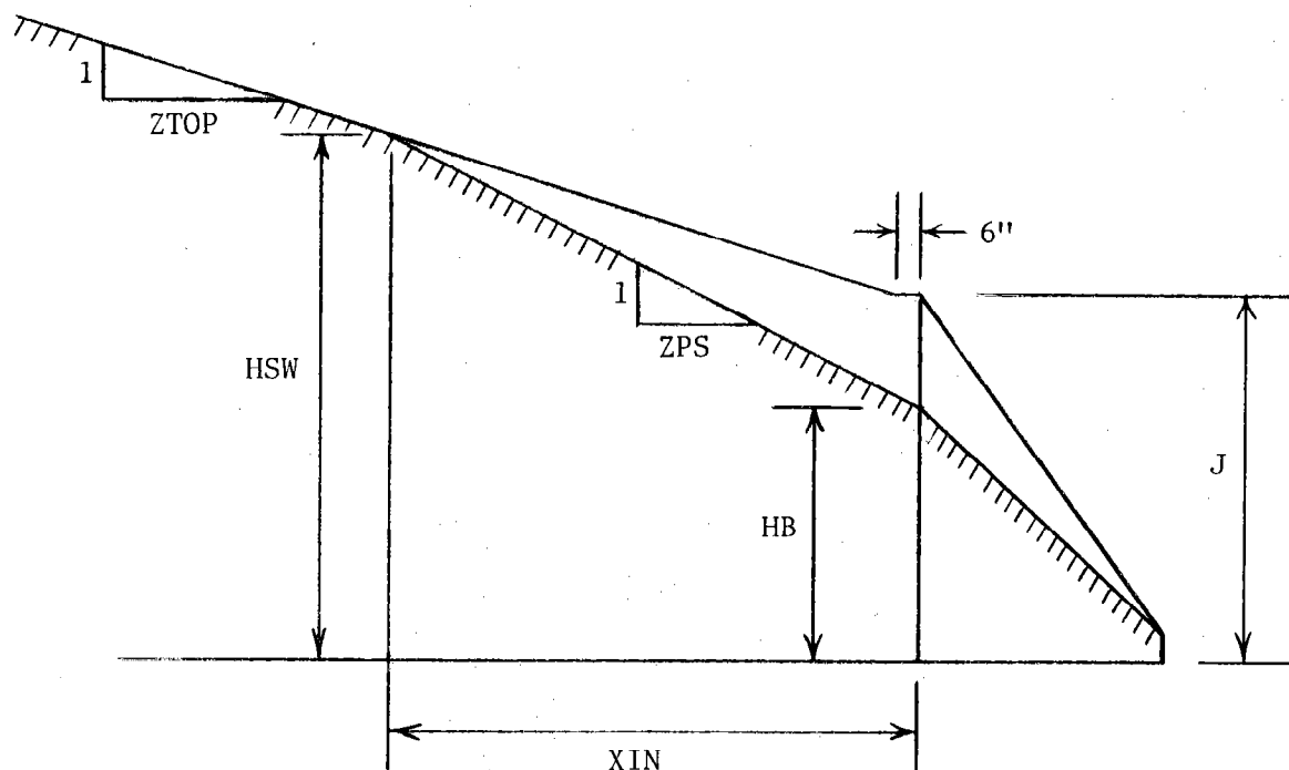
Figure 32. Adaptation of earthfill slope parameter.
