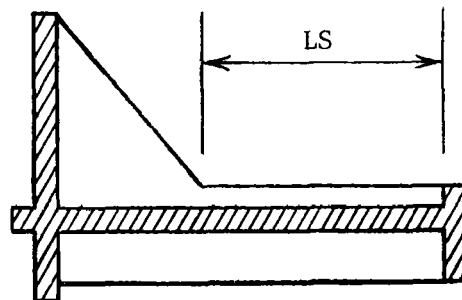
Figure 18. Development of longitudinal sill.
