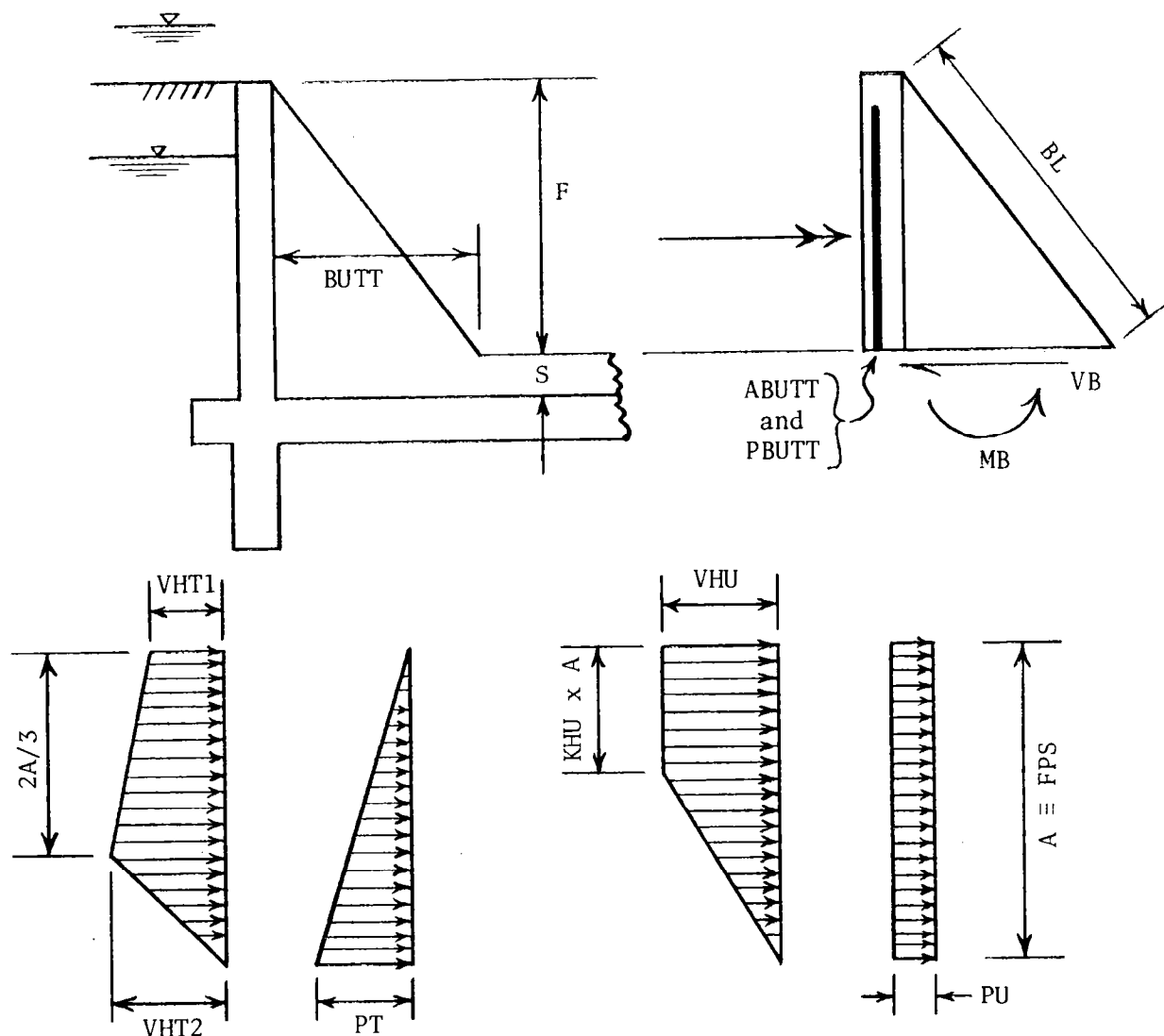
Figure 41. Buttruss loadings.
