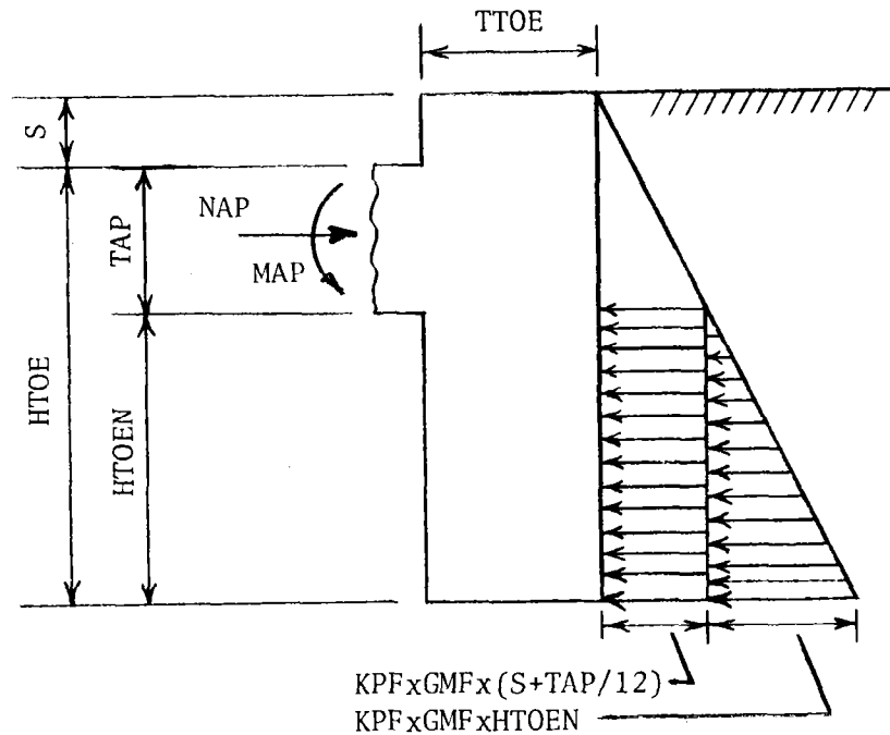
Figure 30. Toewall cantilever bending.
