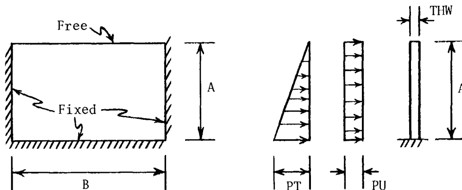
Figure 9. Headwall panel and loading.
