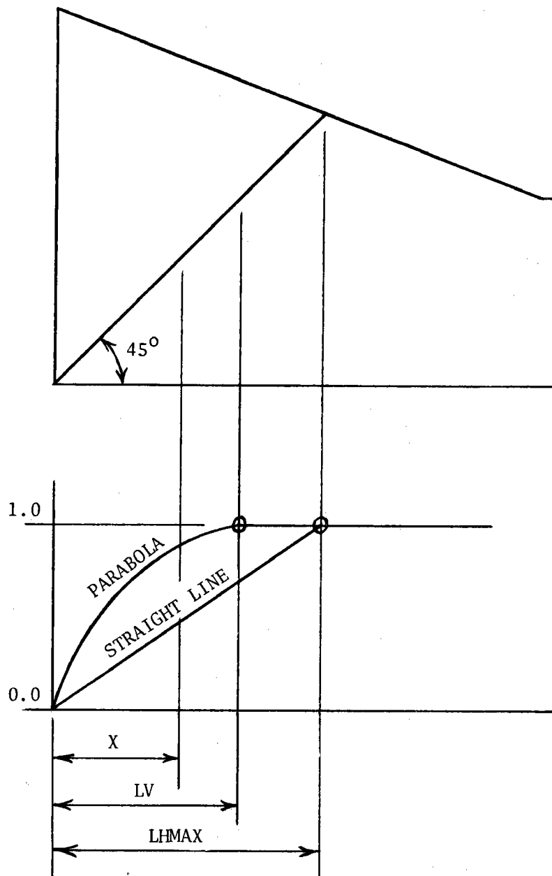
Figure 38. Effect of statical sidewall moments.
