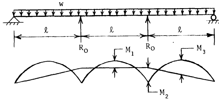
Figure 16. Effect of reactive support on moments, 3 spans.
