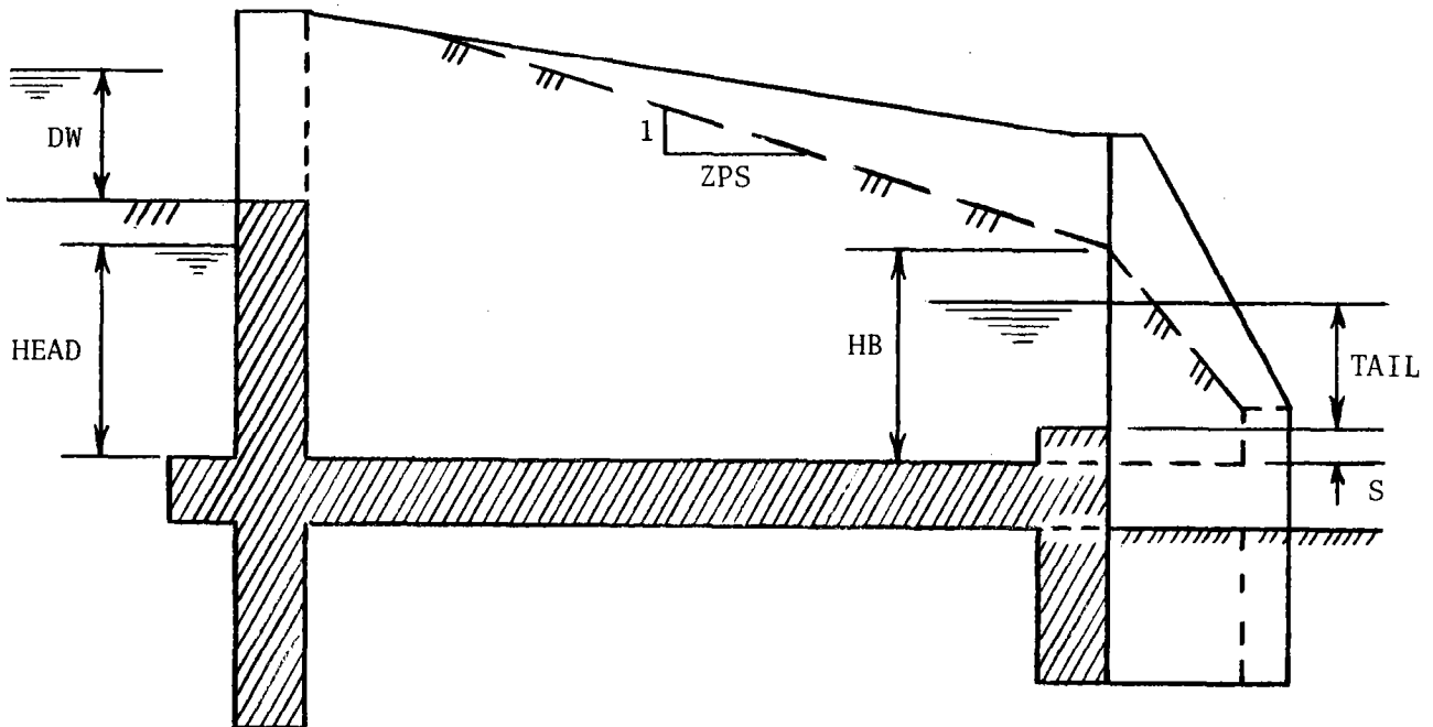
Figure 3. Typical loading case and variation of earthfill.
