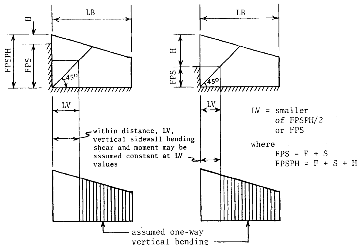
Figure 11. Assumptions for vertical sidewall bending.
