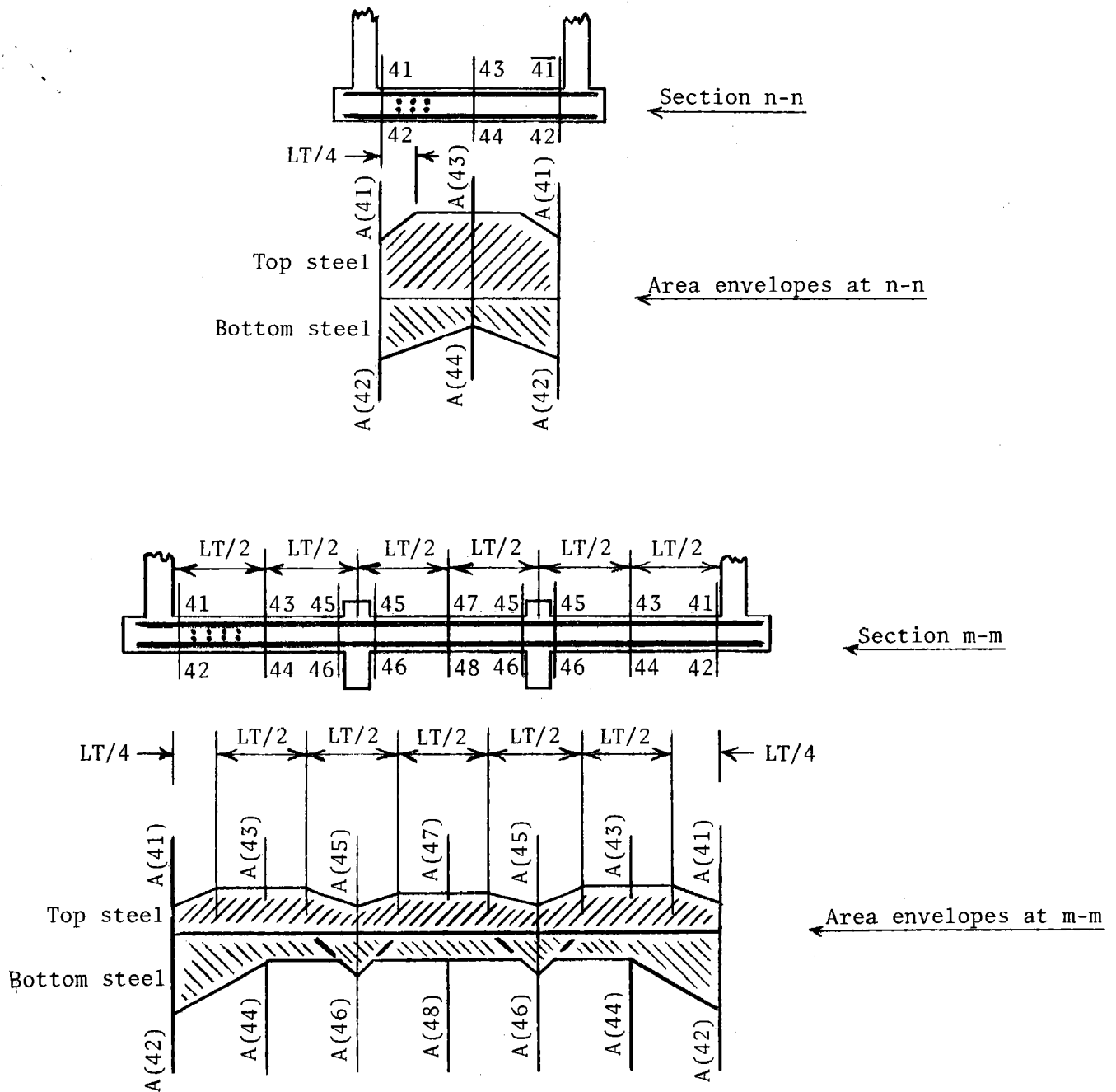
b. Transverse cross sections.
