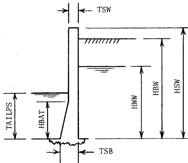
(b) SIDEWALL SECTION
