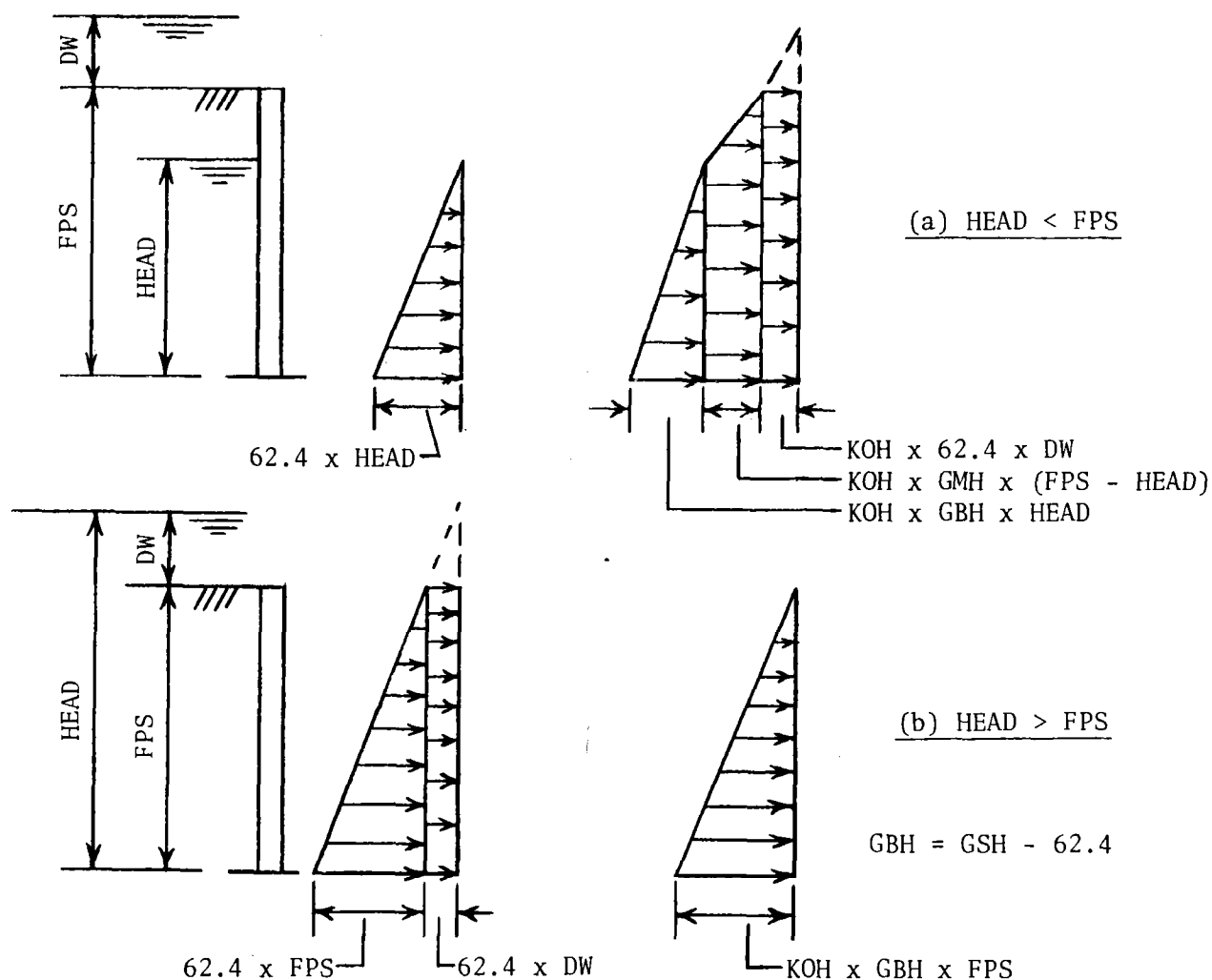
Figure 7. Treatment of upstream headwall pressures.
