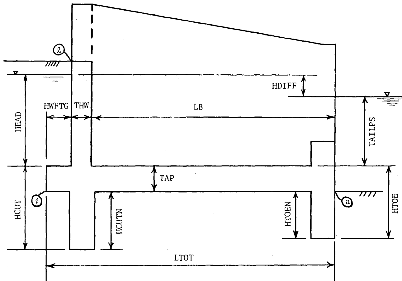
Figure 6. Determination of HCUT.
