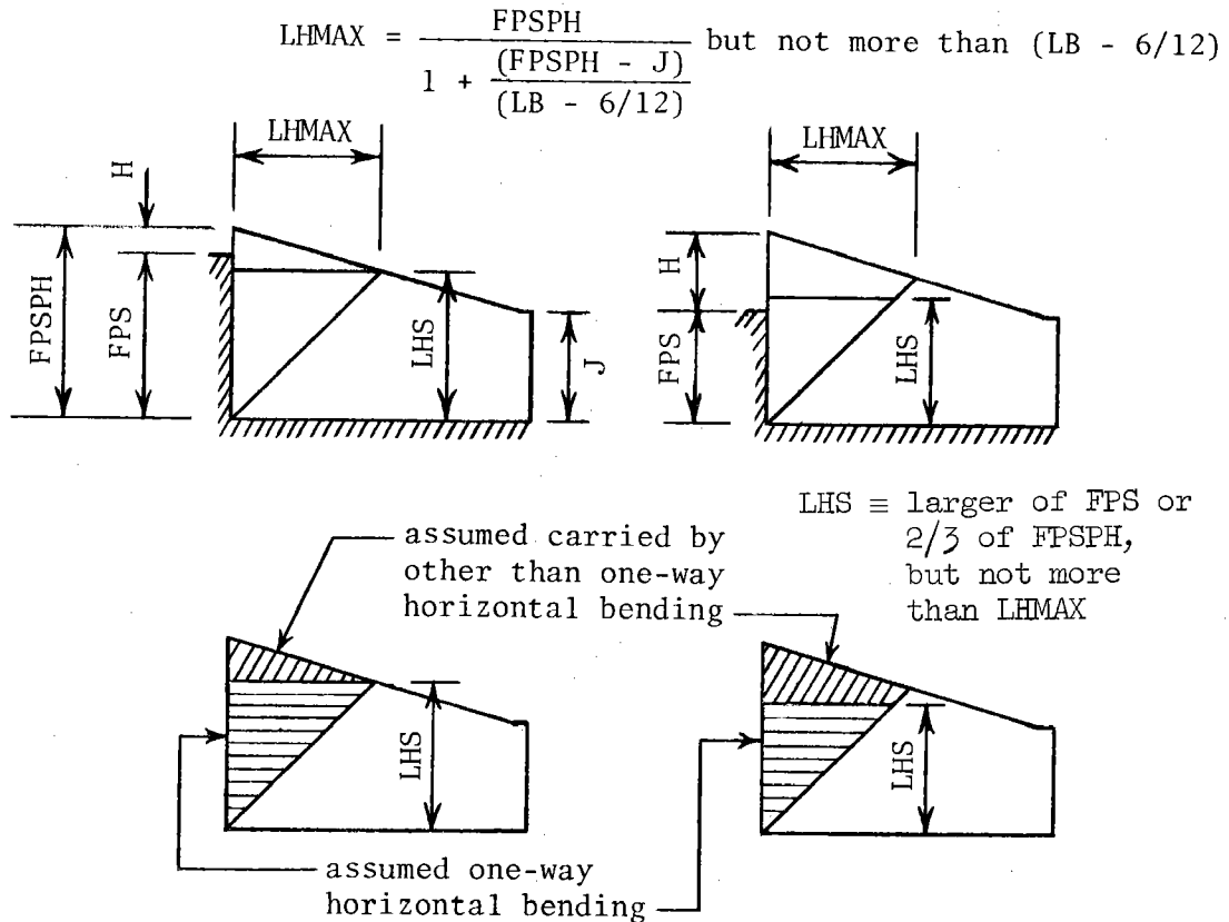
Figure 13. Assumptions for horizontal sidewall bending.
