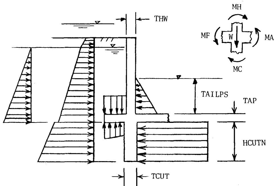
Figure 31. Cutoff wall bending
