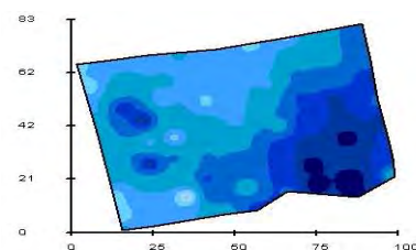
High Traffic area 3.0" rod length Pre-Irrigation DU= 89
