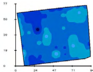
Medium Traffic area Catch Can DU= 78
